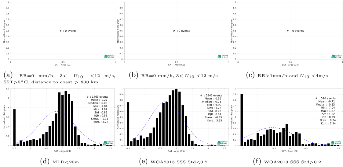
Figure 13: Normalized histogram of \Delta\text{SSS} (Aquarius SSS L3 OR v5 - Monthly (NASA-GSFC) - Argo) for 6 different subdatasets corresponding to: RR=0 mm/h, 3 < U_{10} < 12 m/s, SST > 5^{\circ}\text{C} , distance to coast > 800 km (a), RR=0 mm/h, 3 < U_{10} < 12 m/s (b), RR > 1\text{mm/h} and U_{10} < 4\text{m/s} (c), MLD < 20\text{m} (d), WOA2013 SSS Std < 0.2 (e), WOA2013 SSS Std > 0.2 (f).
