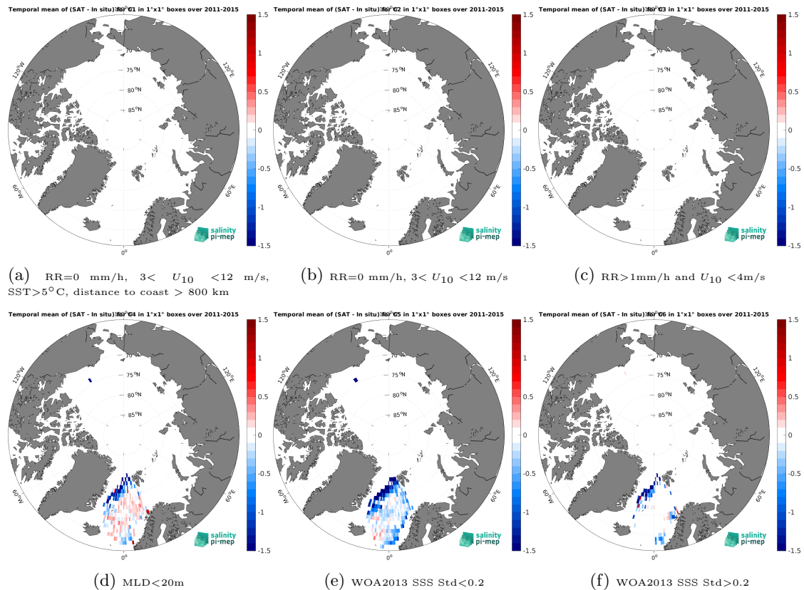
Figure 12: Temporal mean gridded over spatial boxes of size 1^{\circ}\times 1^{\circ} of \Delta\text{SSS} (Aquarius SSS L3 OR v5 - Monthly (NASA-GSFC) - Argo) for 6 different subdatasets corresponding to: RR=0 mm/h, 3 < U_{10} < 12 m/s, SST > 5^{\circ}\text{C} , distance to coast > 800 km (a), RR=0 mm/h, 3 < U_{10} < 12 m/s (b), RR > 1 mm/h and U_{10} < 4 m/s (c), MLD < 20\text{m} (d), WOA2013 SSS Std < 0.2 (e), WOA2013 SSS Std > 0.2 (f).
