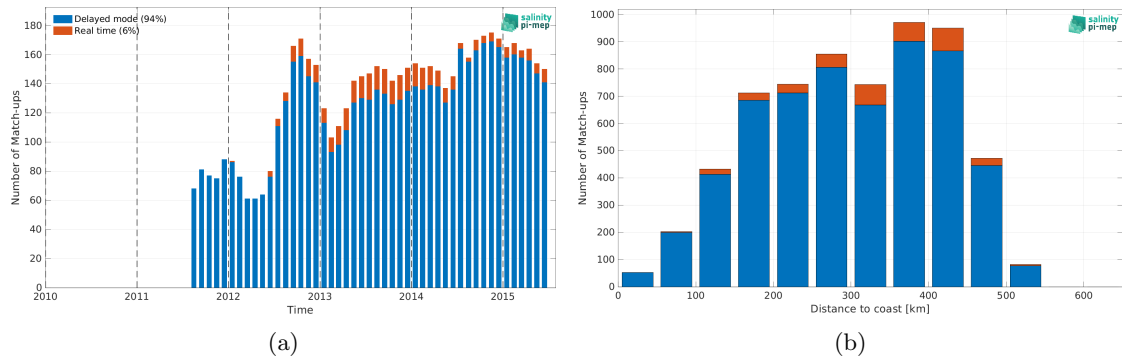
Figure 1: Number of match-ups between Argo and Aquarius SSS L3 OR v5 - Monthly (NASA-GSFC) SSS as a function of time (a) and as function of the distance to coast (b) over the Arctic Ocean Pi-MEP region and for the full satellite product period.
