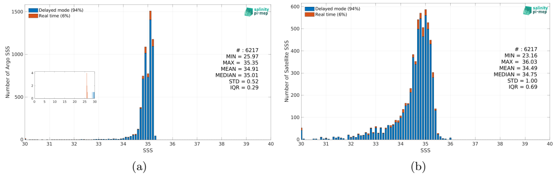
Figure 2: Histograms of SSS from Argo (a) and Aquarius SSS L3 OR v5 - Monthly (NASA-GSFC) (b) considering all match-up pairs per bins of 0.1 over the Arctic Ocean Pi-MEP region and for the full satellite product period.
