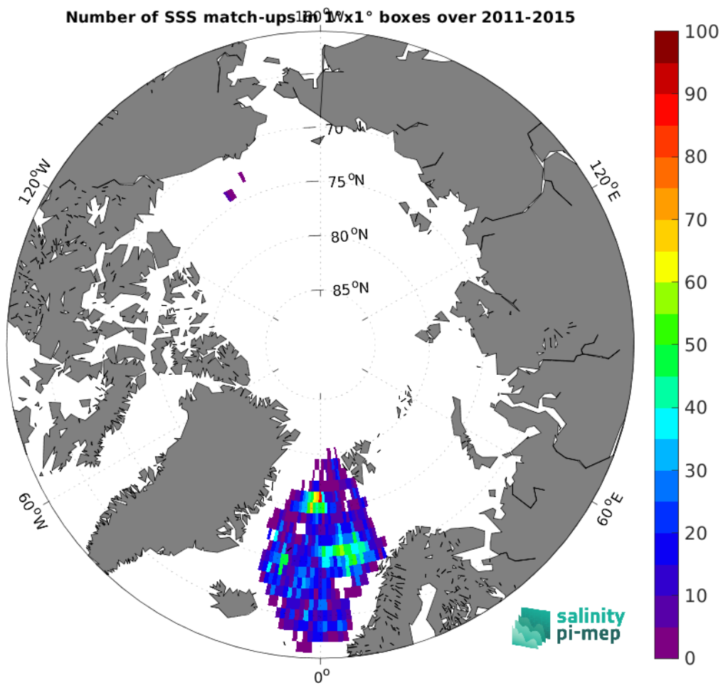
Figure 4: Number of SSS match-ups between Argo SSS and the Aquarius SSS L3 OR v5 - Monthly (NASA-GSFC) SSS product for the Arctic Ocean Pi-MEP region over 1^\circ \times 1^\circ boxes and for the full satellite product period.
