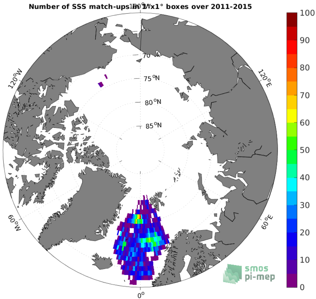
Figure 4: Number of SSS match-ups between Argo SSS and the Aquarius SSS L3 OR v5 - Monthly (NASA-GSFC) SSS product for the Arctic Ocean Pi-MEP region over 1^{\circ} \times 1^{\circ} boxes and for the full satellite product period.
