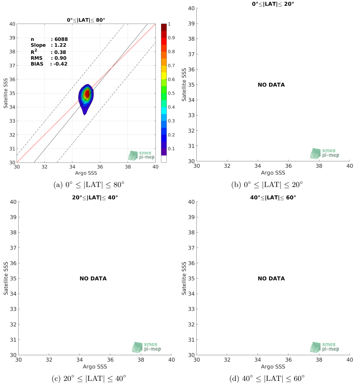
Figure 9: Contour maps of the concentration of Aquarius-L3-OR-V5-MONTHLY-1DEG SSS (y-axis) versus Argo SSS (x-axis) at match-up pairs for different latitude bands. For each plot, the red line shows x=y . The black thin and dashed lines indicate a linear fit through the data cloud and the \pm 95\% confidence levels, respectively. The number match-up pairs n , the slope and R^2 coefficient of the linear fit, the root mean square (RMS) and the mean bias between satellite and in situ data are indicated for each latitude band in each plots.
