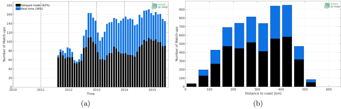
Figure 1: Number of match-ups between Argo and Aquarius-L3-OR-V5-MONTHLY-1DEG SSS as a function of time (a) and as function of the distance to coast (b) over the Arctic Ocean Pi-MEP region and for the full satellite product period.
