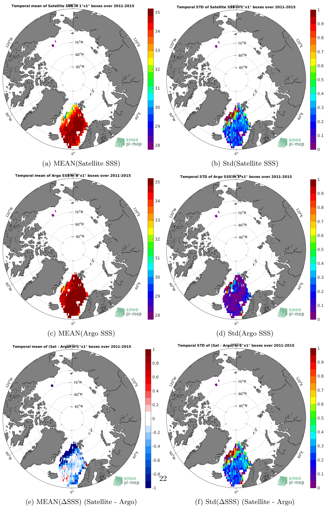
Figure 6: Temporal mean (left) and Std (right) of SSS from Aquarius-L3-OR-V5-MONTHLY-1DEG (top), Argo (middle), and of \Delta SSS (Satellite - Argo). Only match-up pairs are used to generate these maps.
