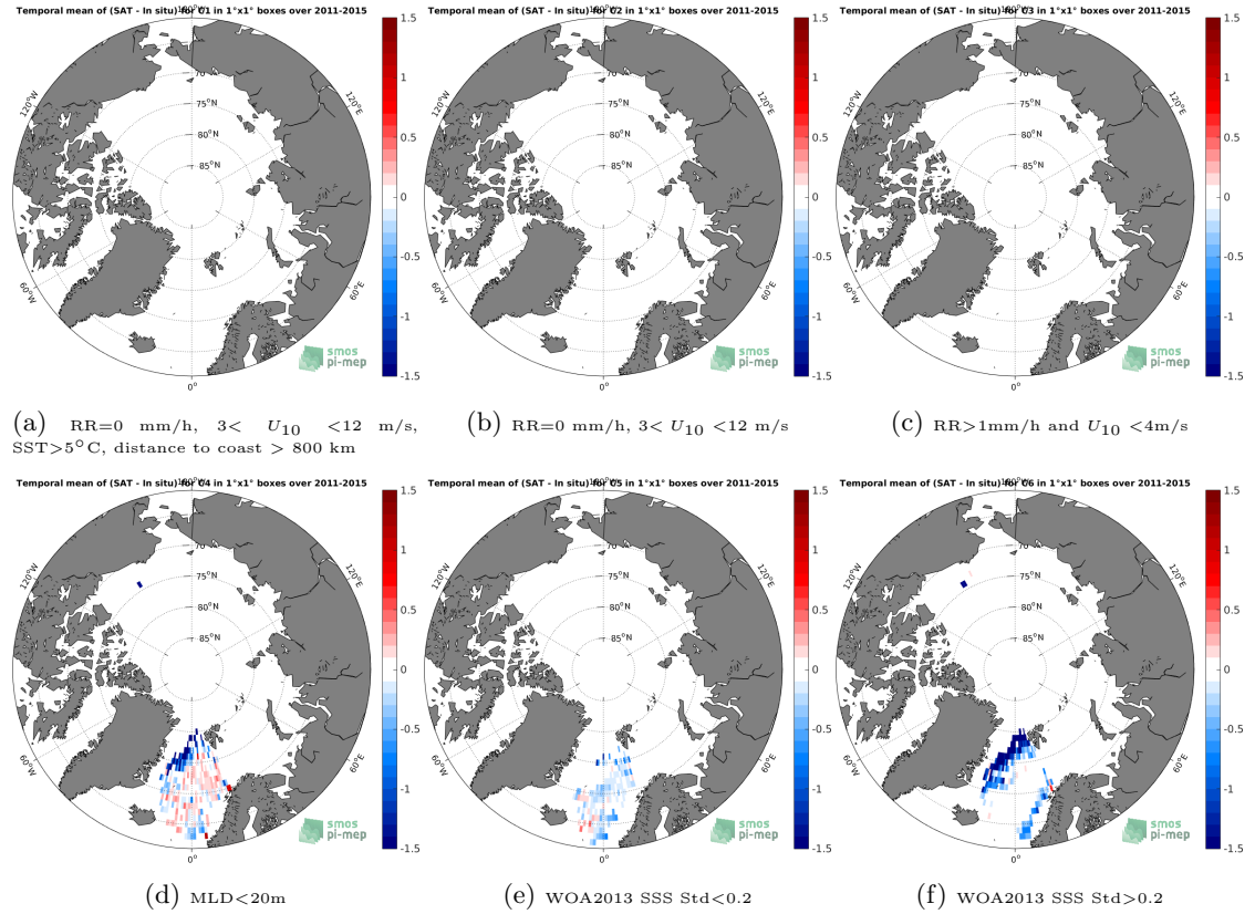
Figure 12: Temporal mean gridded over spatial boxes of size 1^\circ \times 1^\circ of \Delta SSS (Aquarius-L3-OR-V5-MONTHLY-1DEG - Argo) for 6 different subdatasets corresponding to: RR=0 mm/h, 3 < U_{10} < 12 m/s, SST > 5^\circ C , distance to coast > 800 km (a), RR=0 mm/h, 3 < U_{10} < 12 m/s (b), RR > 1 mm/h and U_{10} < 4 m/s (c), MLD < 20 m (d), WOA2013 SSS Std < 0.2 (e), WOA2013 SSS Std > 0.2 (f).
