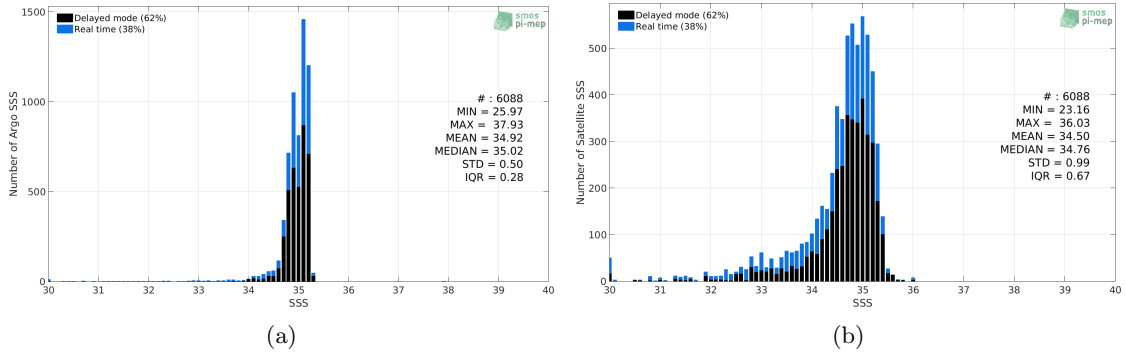
Figure 2: Histograms of SSS from Argo (a) and Aquarius-L3-OR-V5-MONTHLY-1DEG (b) considering all match-up pairs per bins of 0.1 over the Arctic Ocean Pi-MEP region and for the full satellite product period.
