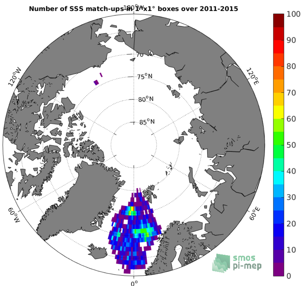
Figure 4: Number of SSS match-ups between Argo SSS and the Aquarius-L3-OR-V5-MONTHLY-1DEG SSS product for the Arctic Ocean Pi-MEP region over 1°x1° boxes and for the full satellite product period.
