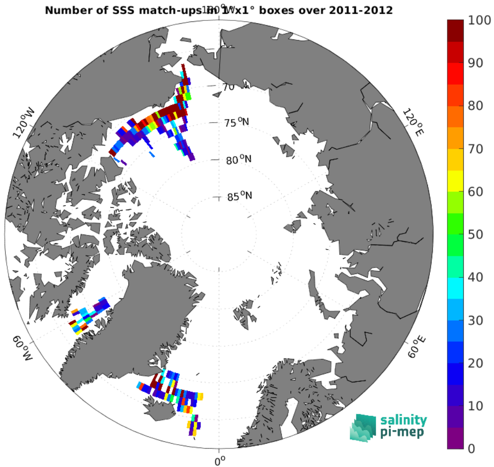
Figure 5: Number of SSS match-ups between TSG (SAMOS) SSS and the Aquarius SSS L3 OR v5 - Monthly - Rain mask (NASA-GSFC) SSS product for the Arctic Ocean Pi-MEP region over 1^\circ \times 1^\circ boxes and for the full satellite product period.
