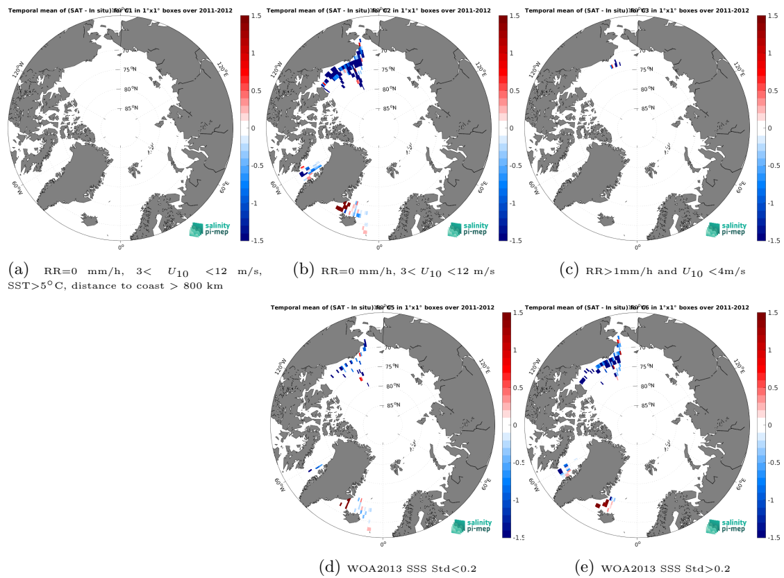
Figure 14: Temporal mean gridded over spatial boxes of size 1^\circ \times 1^\circ of \Delta\text{SSS} (Aquarius SSS L3 OR v5 - Monthly - Rain mask (NASA-GSFC) - TSG (SAMOS)) for 5 different subdatasets corresponding to:RR=0 mm/h, 3 < U_{10} < 12 m/s, SST>5°C, distance to coast > 800 km (a), RR=0 mm/h, 3 < U_{10} < 12 m/s (b), RR>1mm/h and U_{10} < 4 m/s (c), WOA2013 SSS Std<0.2 (d), WOA2013 SSS Std>0.2 (e).
