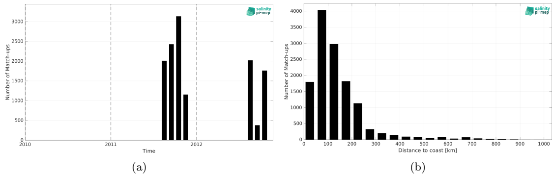
Figure 2: Number of match-ups between TSG (SAMOS) and Aquarius SSS L3 OR v5 - Monthly - Rain mask (NASA-GSFC) SSS as a function of time (a) and as function of the distance to coast (b) over the Arctic Ocean Pi-MEP region and for the full satellite product period.
