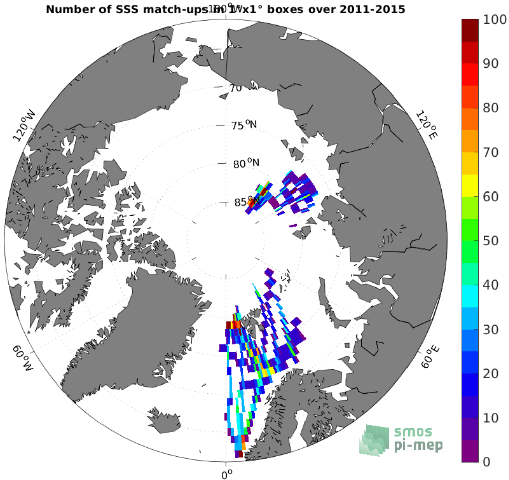
Figure 4: Number of SSS match-ups between TSG (Polarstern) SSS and the Aquarius SSS L3 OR v5 - Monthly - Rain mask (NASA-GSFC) SSS product for the Arctic Ocean Pi-MEP region over 1^\circ \times 1^\circ boxes and for the full satellite product period.
