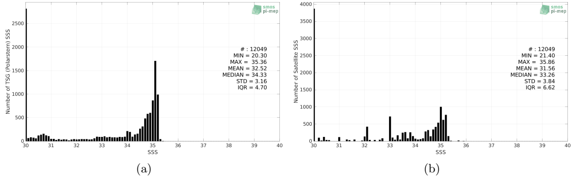
Figure 2: Histograms of SSS from TSG (Polarstern) (a) and Aquarius SSS L3 OR v5 - Monthly - Rain mask (NASA-GSFC) (b) considering all match-up pairs per bins of 0.1 over the Arctic Ocean Pi-MEP region and for the full satellite product period.
