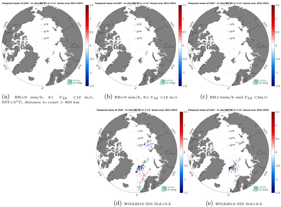
Figure 12: Temporal mean gridded over spatial boxes of size 1^{\circ}\times 1^{\circ} of \Delta\text{SSS} (Aquarius SSS L3 OR v5 - Monthly - Rain mask (NASA-GSFC) - TSG (Polarstern)) for 5 different subdatasets corresponding to:RR=0 mm/h, 3 < U_{10} < 12 m/s, SST > 5^{\circ}\text{C} , distance to coast > 800 km (a), RR=0 mm/h, 3 < U_{10} < 12 m/s (b), RR > 1 mm/h and U_{10} < 4 m/s (c), WOA2013 SSS Std < 0.2 (d), WOA2013 SSS Std > 0.2 (e).
