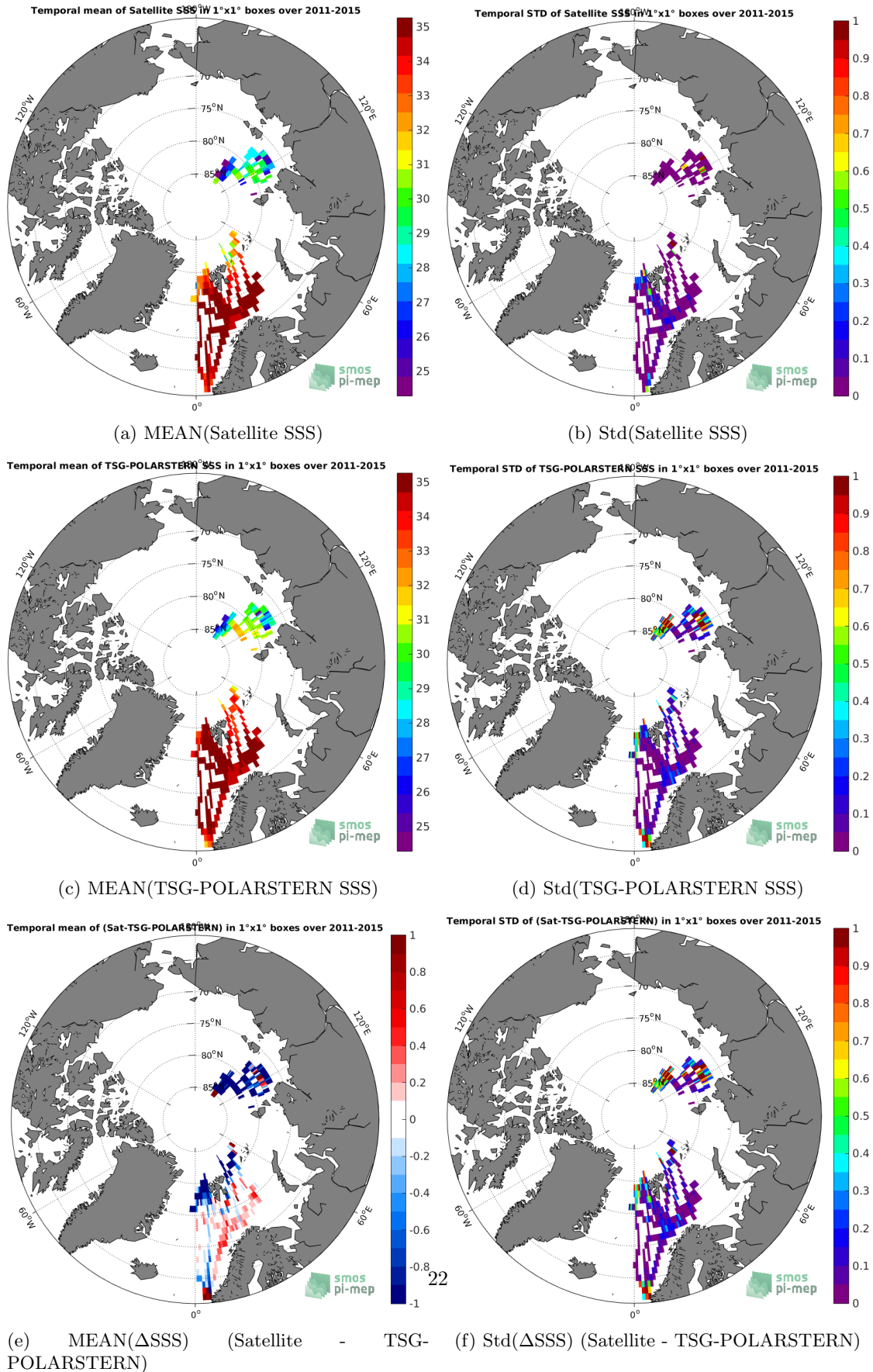
Figure 6: Temporal mean (left) and Std (right) of SSS from Aquarius-L3-OR-V5-MONTHLY-RAIN-MASK-IDEQ (top), TSG-POLARSTERN (middle), and of \Delta SSS (Satellite - TSG-POLARSTERN). Only match-up pairs are used to generate these maps.
