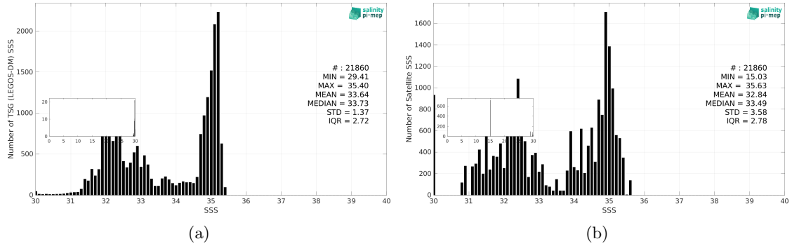
Figure 3: Histograms of SSS from TSG (LEGOS-DM) (a) and Aquarius SSS L3 OR v5 - Monthly - Rain mask (NASA-GSFC) (b) considering all match-up pairs per bins of 0.1 over the Arctic Ocean Pi-MEP region and for the full satellite product period.
