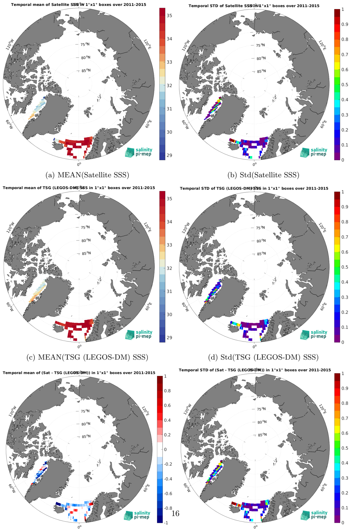
Figure 7: Temporal mean (left) and Std (right) of SSS from Aquarius SSS L3 OR v5 - Monthly - Rain mask (NASA-GSFC) (top), TSG (LEGOS-DM) (middle), and of \Delta SSS (Satellite - TSG (LEGOS-DM)). Only match-up pairs are used to generate these maps.
