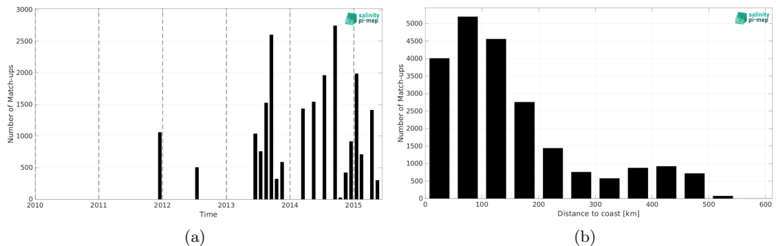
Figure 2: Number of match-ups between TSG (LEGOS-DM) and Aquarius SSS L3 OR v5 - Monthly - Rain mask (NASA-GSFC) SSS as a function of time (a) and as function of the distance to coast (b) over the Arctic Ocean Pi-MEP region and for the full satellite product period.
