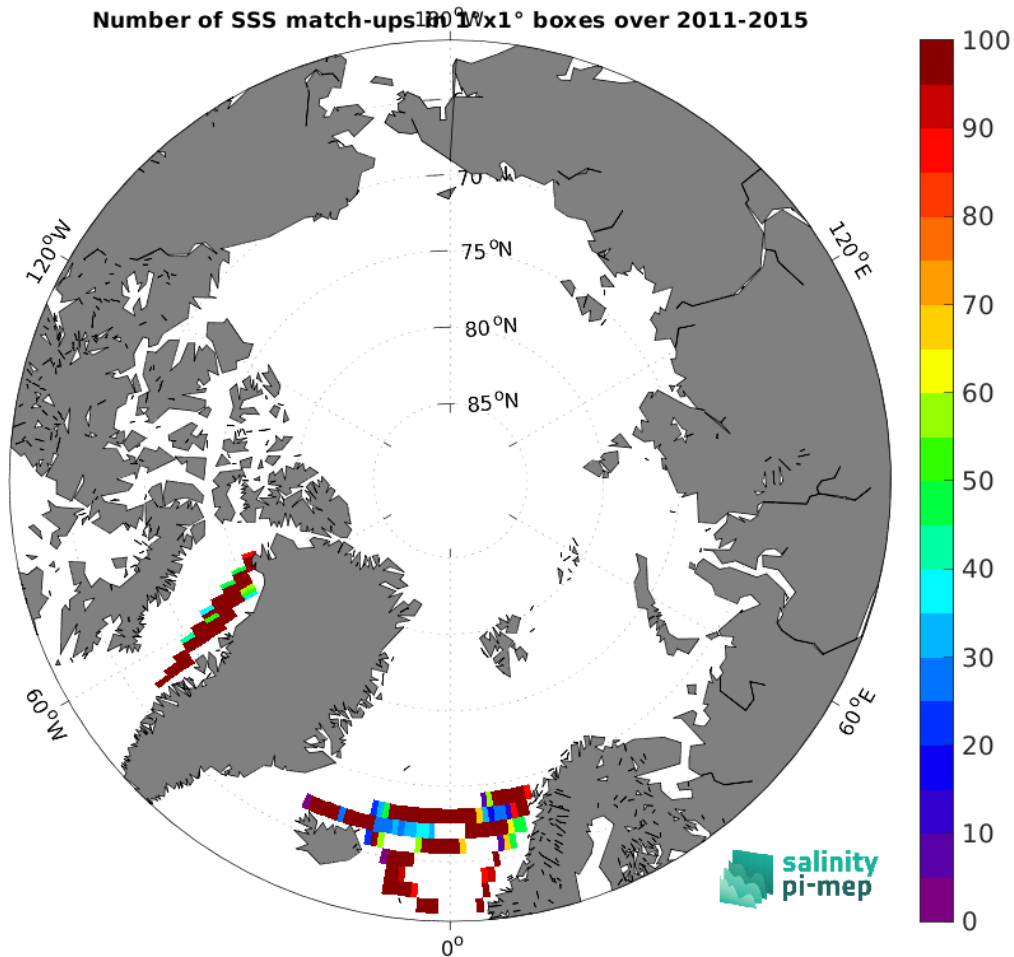
Figure 5: Number of SSS match-ups between TSG (LEGOS-DM) SSS and the Aquarius SSS L3 OR v5 - Monthly - Rain mask (NASA-GSFC) SSS product for the Arctic Ocean Pi-MEP region over 1^\circ \times 1^\circ boxes and for the full satellite product period.
