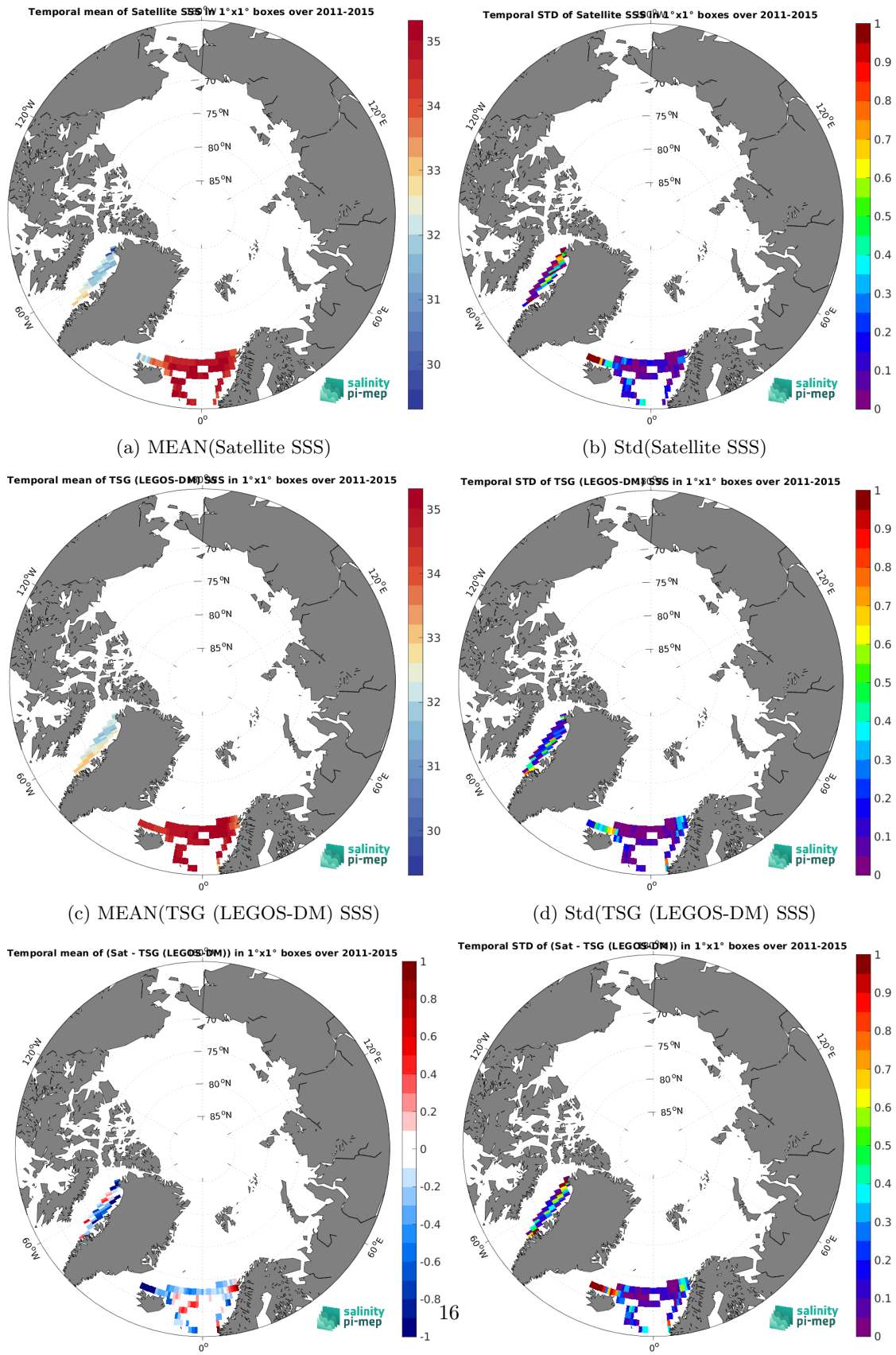
Figure 6: Temporal mean (left) and Std (right) of SSS from Aquarius SSS L3 OR v5 - Monthly - Rain mask (NASA-GSFC) (top), TSG (LEGOS-DM) (middle), and of \Delta SSS (Satellite - TSG (LEGOS-DM)). Only match-up pairs are used to generate these maps.
