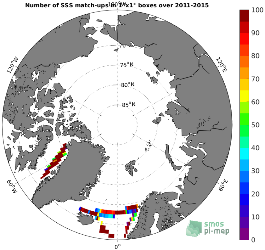
Figure 4: Number of SSS match-ups between TSG-LEGOS-DM SSS and the Aquarius-L3-OR-V5-MONTHLY-RAIN-MASK-1DEG SSS product for the Arctic Ocean Pi-MEP region over 1^\circ \times 1^\circ boxes and for the full satellite product period.
