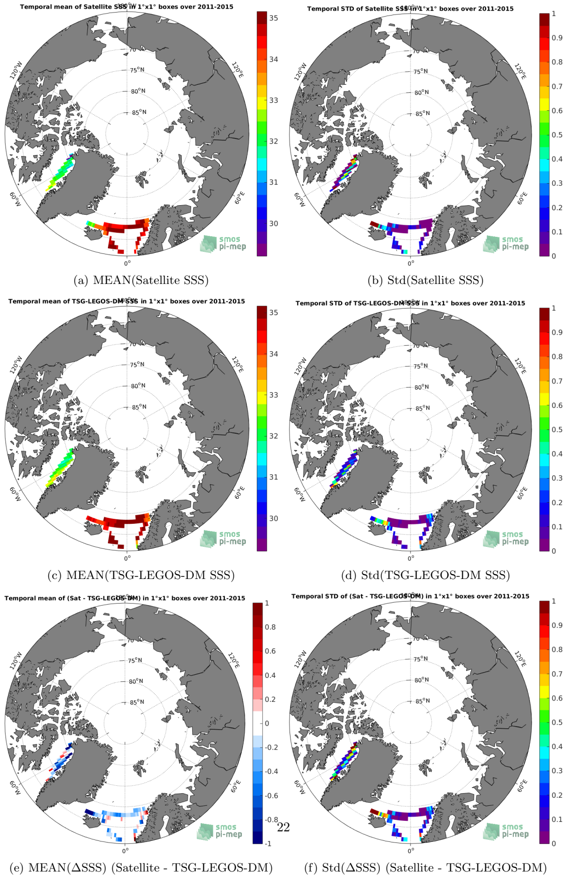
Figure 6: Temporal mean (left) and Std (right) of SSS from Aquarius-L3-OR-V5-MONTHLY-RAIN-MASK-1DEG (top), TSG-LEGOS-DM (middle), and of \Delta SSS (Satellite - TSG-LEGOS-DM). Only match-up pairs are used to generate these maps.
