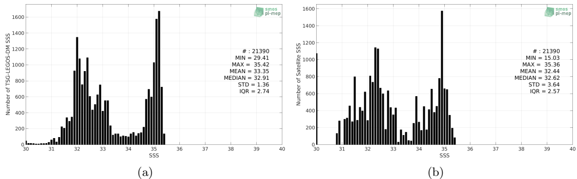
Figure 2: Histograms of SSS from TSG-LEGOS-DM (a) and Aquarius-L3-OR-V5-MONTHLY-RAIN-MASK-1DEG (b) considering all match-up pairs per bins of 0.1 over the Arctic Ocean Pi-MEP region and for the full satellite product period.
