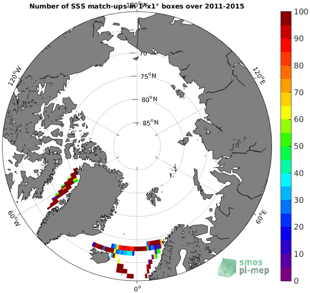
Figure 4: Number of SSS match-ups between TSG-LEGOS-DM SSS and the Aquarius-L3-OR-V5-MONTHLY-RAIN-MASK-1DEG SSS product for the Arctic Ocean Pi-MEP region over 1°x1° boxes and for the full satellite product period.
