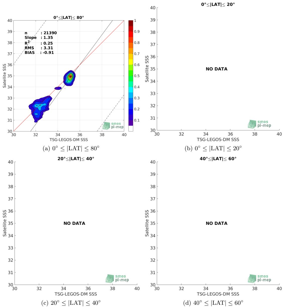
Figure 9: Contour maps of the concentration of Aquarius-L3-OR-V5-MONTHLY-RAIN-MASK-1DEG SSS (y-axis) versus TSG-LEGOS-DM SSS (x-axis) at match-up pairs for different latitude bands. For each plot, the red line shows x=y . The black thin and dashed lines indicate a linear fit through the data cloud and the \pm 95\% confidence levels, respectively. The number match-up pairs n , the slope and R^2 coefficient of the linear fit, the root mean square (RMS) and the mean bias between satellite and in situ data are indicated for each latitude band in each plots.
