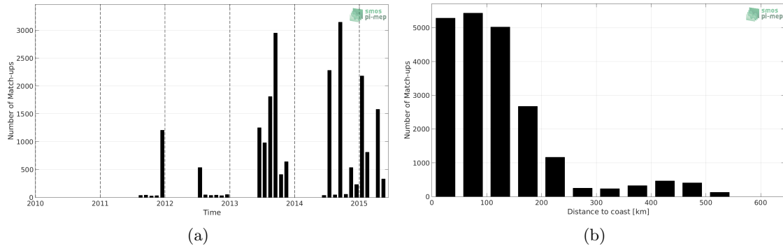
Figure 1: Number of match-ups between TSG-LEGOS-DM and Aquarius-L3-OR-V5-MONTHLY-RAIN-MASK-1DEG SSS as a function of time (a) and as function of the distance to coast (b) over the Arctic Ocean Pi-MEP region and for the full satellite product period.
