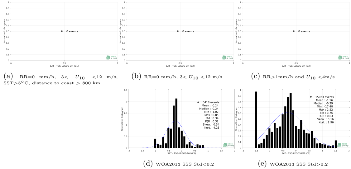
Figure 13: Normalized histogram of \Delta\text{SSS} (Aquarius-L3-OR-V5-MONTHLY-RAIN-MASK-1DEG - TSG-LEGOS-DM) for 5 different subdatasets corresponding to: RR=0 mm/h, 3 < U_{10} < 12 m/s, SST>5°C, distance to coast > 800 km (a), RR=0 mm/h, 3 < U_{10} < 12 m/s (b), RR>1mm/h and U_{10} < 4 m/s (c), WOA2013 SSS Std<0.2 (d), WOA2013 SSS Std>0.2 (e).
