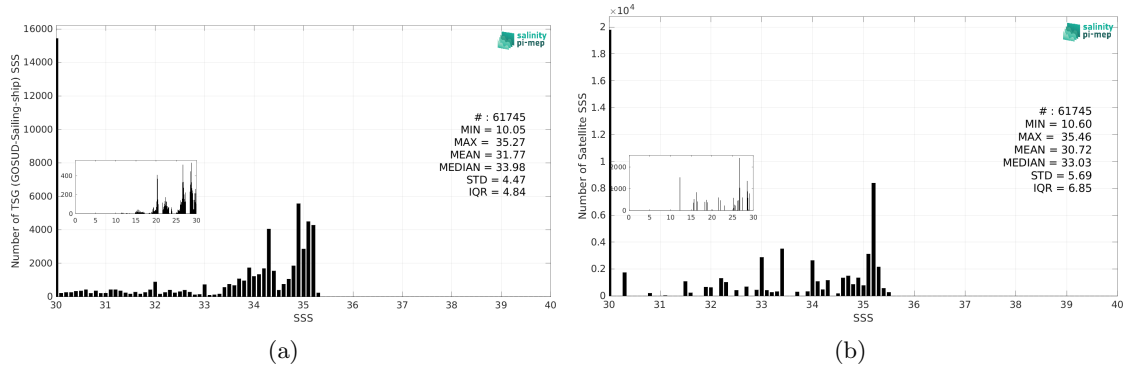
Figure 3: Histograms of SSS from TSG (GOSUD-Sailing-ship) (a) and Aquarius SSS L3 OR v5 - Monthly - Rain mask (NASA-GSFC) (b) considering all match-up pairs per bins of 0.1 over the Arctic Ocean Pi-MEP region and for the full satellite product period.
