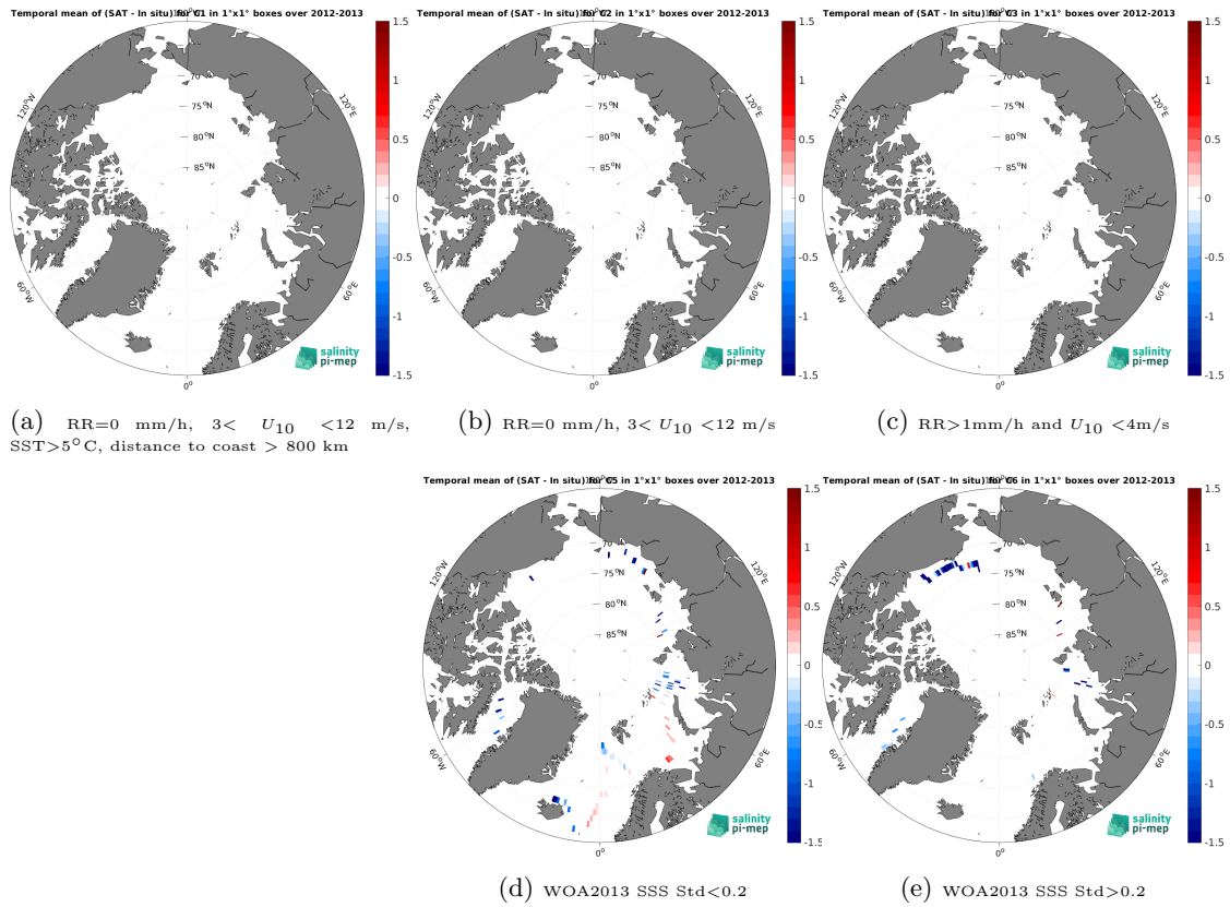
Figure 12: Temporal mean gridded over spatial boxes of size 1^\circ \times 1^\circ of \Delta\text{SSS} (Aquarius SSS L3 OR v5 - Monthly - Rain mask (NASA-GSFC) - TSG (GOSUD-Sailing-ship)) for 5 different subdatasets corresponding to: RR=0 mm/h, 3 < U_{10} < 12 m/s, SST > 5^\circ\text{C} , distance to coast > 800 km (a), RR=0 mm/h, 3 < U_{10} < 12 m/s (b), RR > 1 mm/h and U_{10} < 4 m/s (c), WOA2013 SSS Std < 0.2 (d), WOA2013 SSS Std > 0.2 (e).
