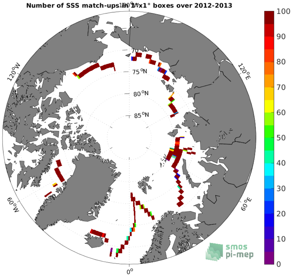
Figure 4: Number of SSS match-ups between TSG (GOSUD-Sailing-ship) SSS and the Aquarius SSS L3 OR v5 - Monthly - Rain mask (NASA-GSFC) SSS product for the Arctic Ocean Pi-MEP region over 1^{\circ} \times 1^{\circ} boxes and for the full satellite product period.
