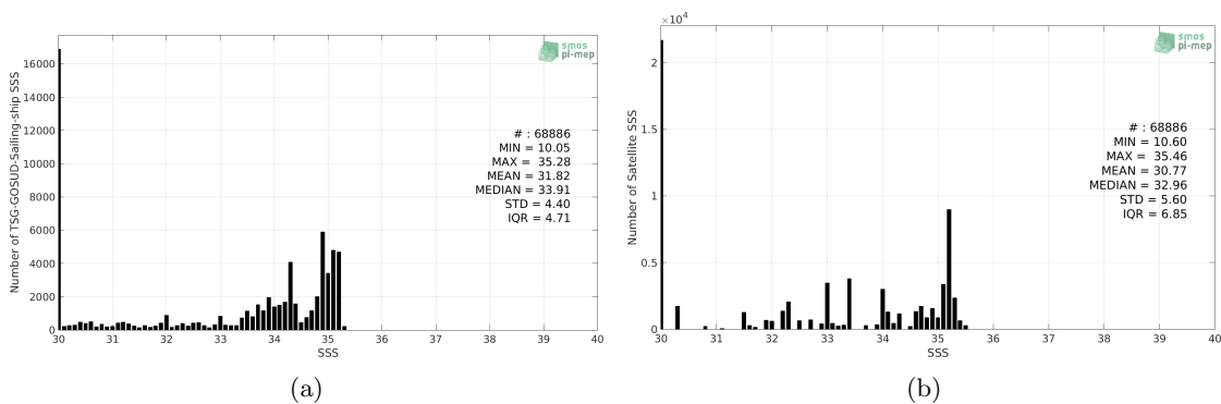
Figure 2: Histograms of SSS from TSG-GOSUD-Sailing-ship (a) and Aquarius-L3-OR-V5-MONTHLY-RAIN-MASK-1DEG (b) considering all match-up pairs per bins of 0.1 over the Arctic Ocean Pi-MEP region and for the full satellite product period.
