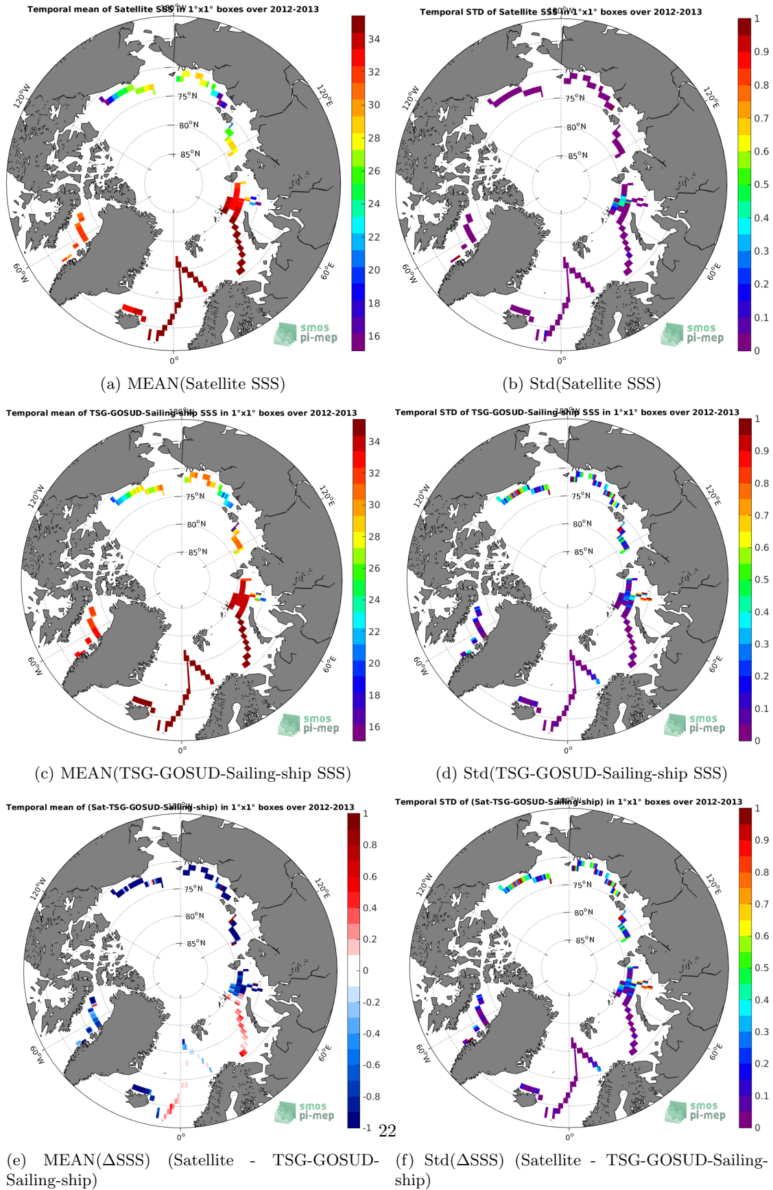
Figure 6: Temporal mean (left) and Std (right) of SSS from Aquarius-L3-OR-V5-MONTHLY-RAIN-MASK-1DEG (top), TSG-GOSUD-Sailing-ship (middle), and of \Delta SSS (Satellite - TSG-GOSUD-Sailing-ship). Only match-up pairs are used to generate these maps.
