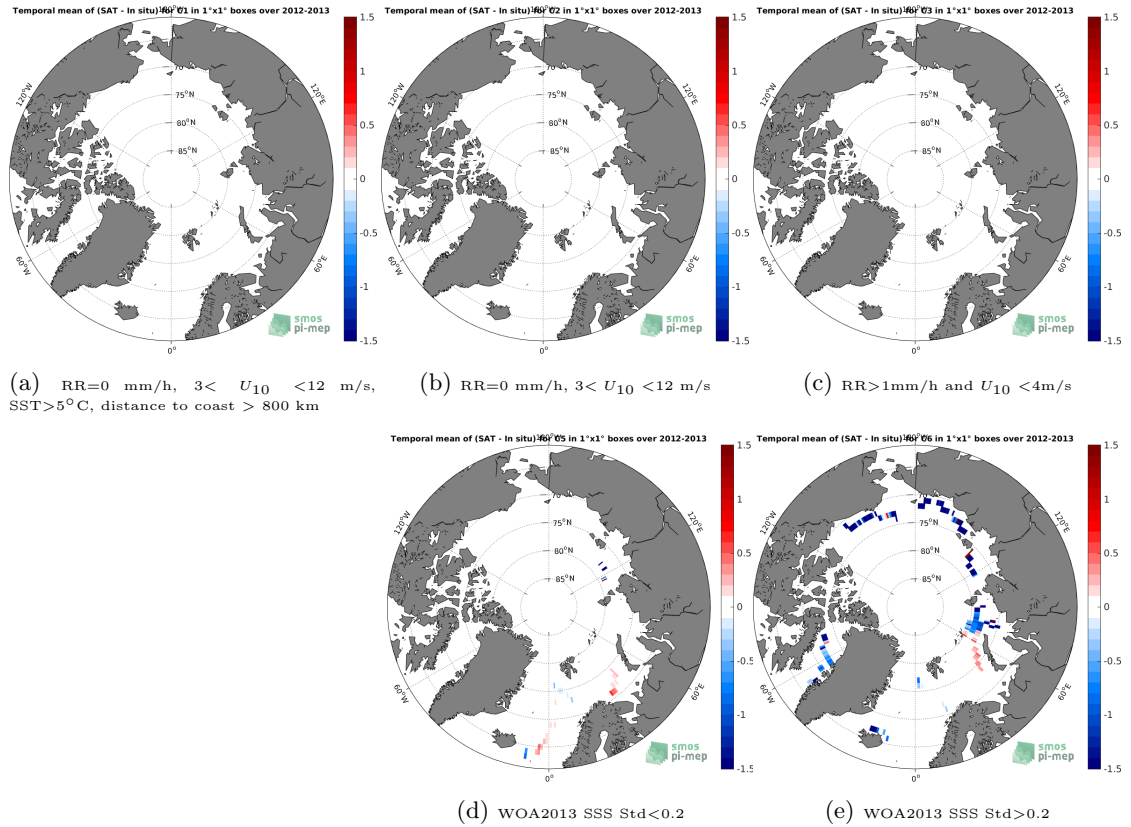
Figure 12: Temporal mean gridded over spatial boxes of size 1^\circ \times 1^\circ of \Delta SSS (Aquarius-L3-OR-V5-MONTHLY-RAIN-MASK-1DEG - TSG-GOSUD-Sailing-ship) for 5 different subdatasets corresponding to: RR=0 mm/h, 3 < U_{10} < 12 m/s, SST > 5^\circ\text{C} , distance to coast > 800 km (a), RR=0 mm/h, 3 < U_{10} < 12 m/s (b), RR > 1 mm/h and U_{10} < 4 m/s (c), WOA2013 SSS Std < 0.2 (d), WOA2013 SSS Std > 0.2 (e).
