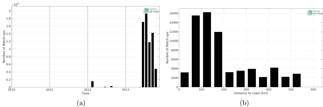
Figure 1: Number of match-ups between TSG-GOSUD-Sailing-ship and Aquarius-L3-OR-V5-MONTHLY-RAIN-MASK-1DEG SSS as a function of time (a) and as function of the distance to coast (b) over the Arctic Ocean Pi-MEP region and for the full satellite product period.
