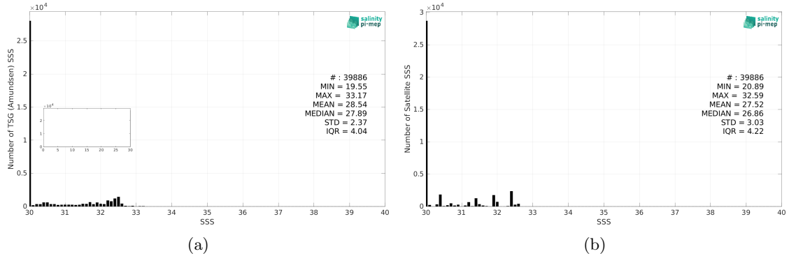
Figure 2: Histograms of SSS from TSG (Amundsen) (a) and Aquarius SSS L3 OR v5 - Monthly - Rain mask (NASA-GSFC) (b) considering all match-up pairs per bins of 0.1 over the Arctic Ocean Pi-MEP region and for the full satellite product period.
