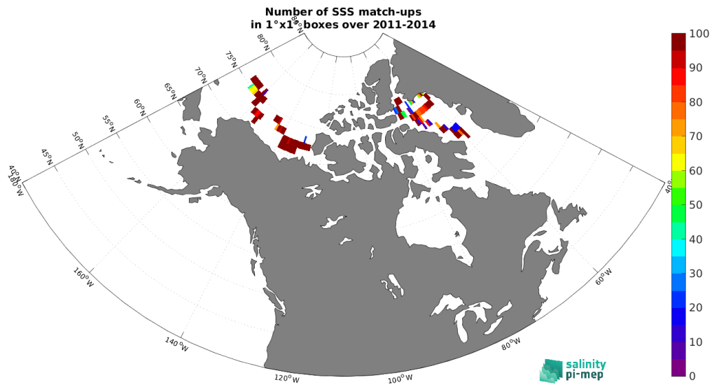
Figure 4: Number of SSS match-ups between TSG (Amundsen) SSS and the Aquarius SSS L3 OR v5 - Monthly - Rain mask (NASA-GSFC) SSS product for the Arctic Ocean Pi-MEP region over 1°x1° boxes and for the full satellite product period.
