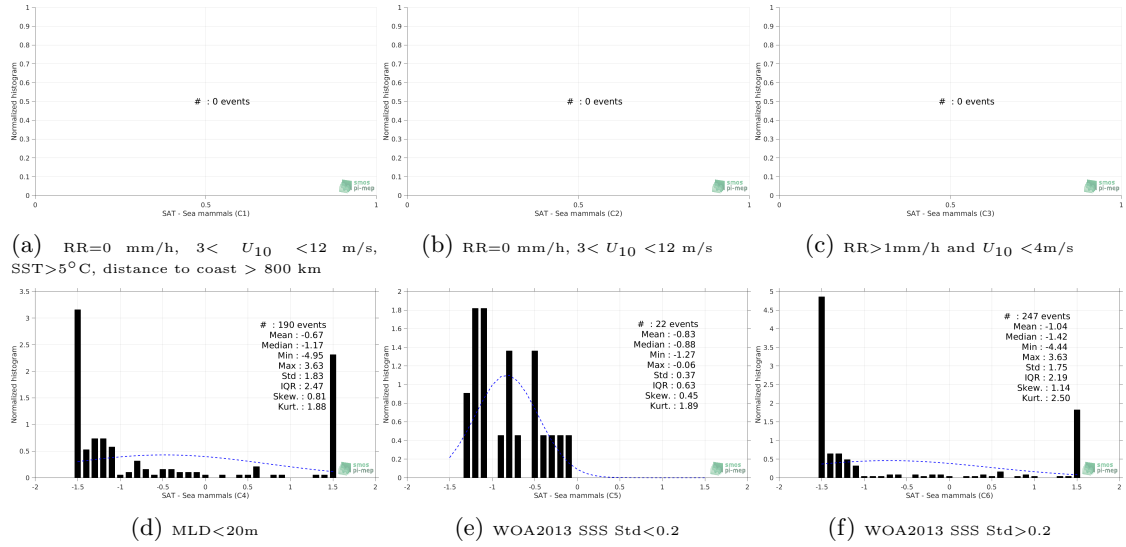
Figure 13: Normalized histogram of \Delta\text{SSS} (Aquarius-L3-OR-V5-MONTHLY-RAIN-MASK-1DEG - Sea mammals) for 6 different subdatasets corresponding to: RR=0 mm/h, 3 < U_{10} < 12 m/s, SST > 5^\circ\text{C} , distance to coast > 800 km (a), RR=0 mm/h, 3 < U_{10} < 12 m/s (b), RR > 1 mm/h and U_{10} < 4 m/s (c), MLD < 20 m (d), WOA2013 SSS Std < 0.2 (e), WOA2013 SSS Std > 0.2 (f).
