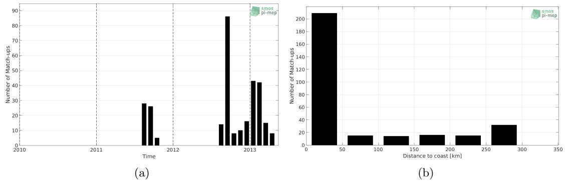
Figure 1: Number of match-ups between Sea mammals and Aquarius-L3-OR-V5-MONTHLY-RAIN-MASK-1DEG SSS as a function of time (a) and as function of the distance to coast (b) over the Arctic Ocean Pi-MEP region and for the full satellite product period.
