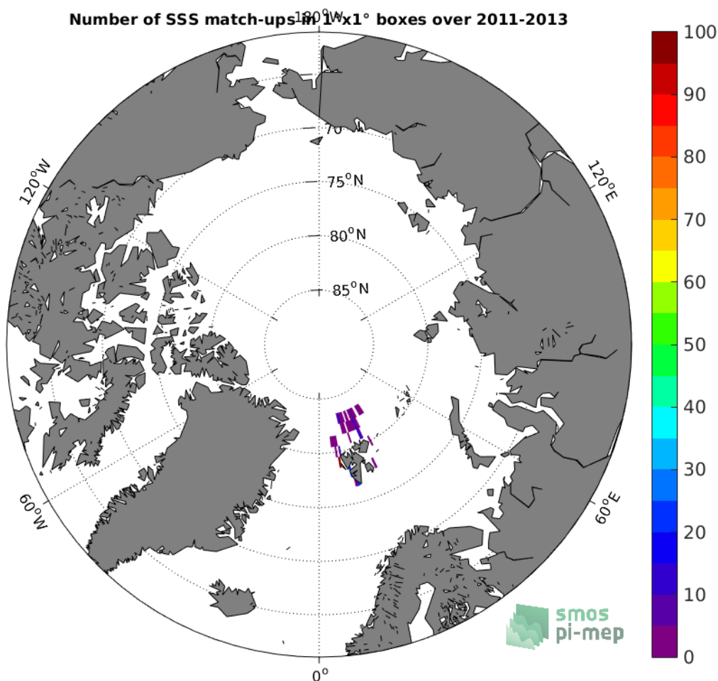
Figure 4: Number of SSS match-ups between Sea mammals SSS and the Aquarius-L3-OR-V5-MONTHLY-RAIN-MASK-1DEG SSS product for the Arctic Ocean Pi-MEP region over 1°x1° boxes and for the full satellite product period.
