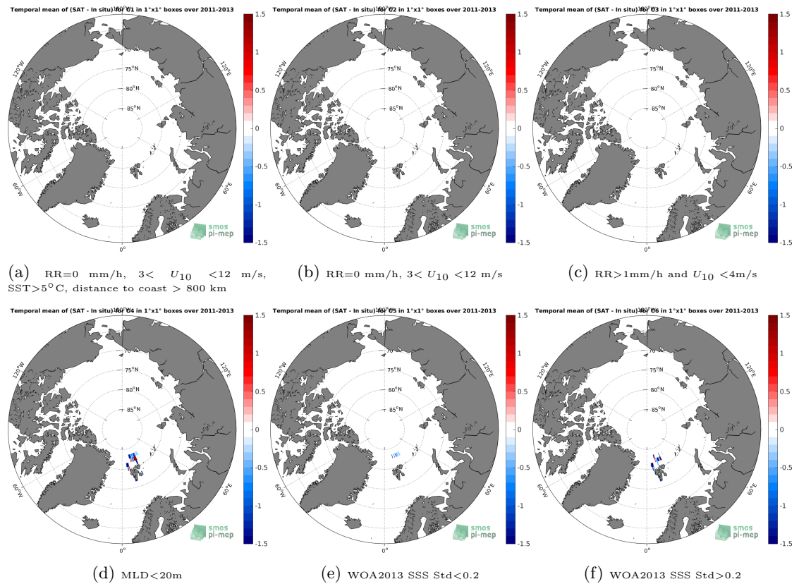
Figure 12: Temporal mean gridded over spatial boxes of size 1^\circ \times 1^\circ of \Delta SSS (Aquarius-L3-OR-V5-MONTHLY-RAIN-MASK-1DEG - Sea mammals) for 6 different subdatasets corresponding to:RR=0 mm/h, 3 < U_{10} < 12 m/s, SST >5^\circ C, distance to coast > 800 km (a), RR=0 mm/h, 3 < U_{10} < 12 m/s (b), RR >1 mm/h and U_{10} < 4 m/s (c),MLD <20 m (d),WOA2013 SSS Std <0.2 (e),WOA2013 SSS Std >0.2 (f).
