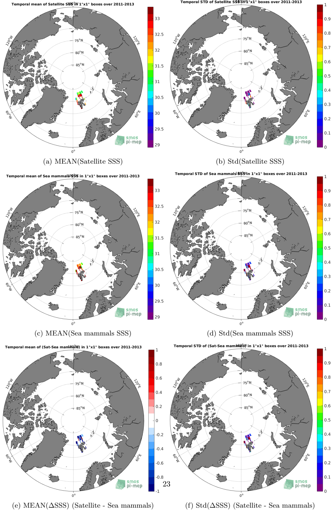
Figure 6: Temporal mean (left) and Std (right) of SSS from Aquarius-L3-OR-V5-MONTHLY-RAIN-MASK-1DEG (top), Sea mammals (middle), and of \Delta SSS (Satellite - Sea mammals). Only match-up pairs are used to generate these maps.
