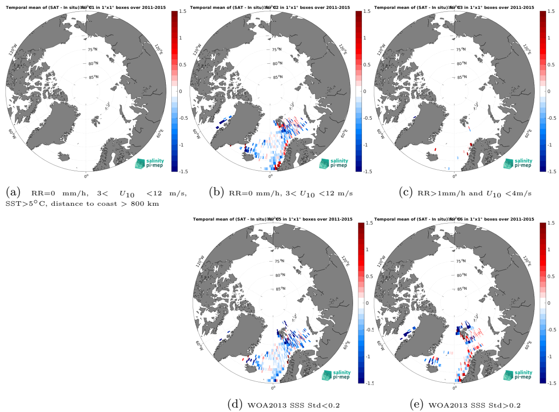
Figure 14: Temporal mean gridded over spatial boxes of size 1^\circ \times 1^\circ of \Delta\text{SSS} (Aquarius SSS L3 OR v5 - Monthly - Rain mask (NASA-GSFC) - ICES) for 5 different subdatasets corresponding to: RR=0 mm/h, 3 < U_{10} < 12 m/s, SST > 5°C, distance to coast > 800 km (a), RR=0 mm/h, 3 < U_{10} < 12 m/s (b), RR > 1mm/h and U_{10} < 4 m/s (c), WOA2013 SSS Std < 0.2 (d), WOA2013 SSS Std > 0.2 (e).
