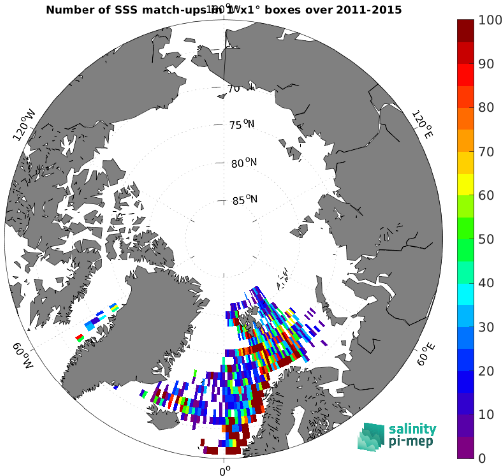
Figure 5: Number of SSS match-ups between ICES SSS and the Aquarius SSS L3 OR v5 - Monthly - Rain mask (NASA-GSFC) SSS product for the Arctic Ocean Pi-MEP region over 1^\circ \times 1^\circ boxes and for the full satellite product period.
