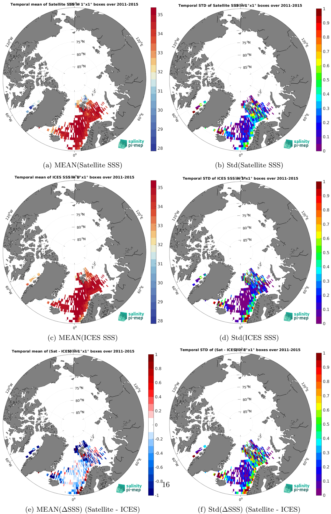
Figure 7: Temporal mean (left) and Std (right) of SSS from Aquarius SSS L3 OR v5 - Monthly - Rain mask (NASA-GSFC) (top), ICES (middle), and of \Delta SSS (Satellite - ICES). Only match-up pairs are used to generate these maps.
