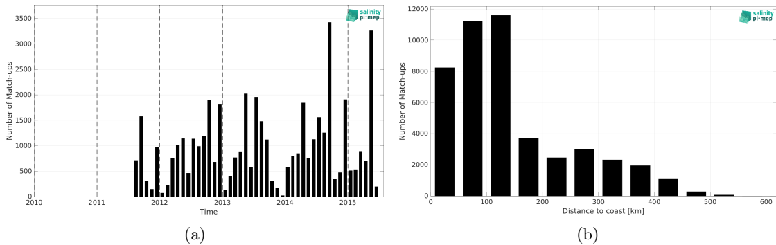
Figure 2: Number of match-ups between ICES and Aquarius SSS L3 OR v5 - Monthly - Rain mask (NASA-GSFC) SSS as a function of time (a) and as function of the distance to coast (b) over the Arctic Ocean Pi-MEP region and for the full satellite product period.
