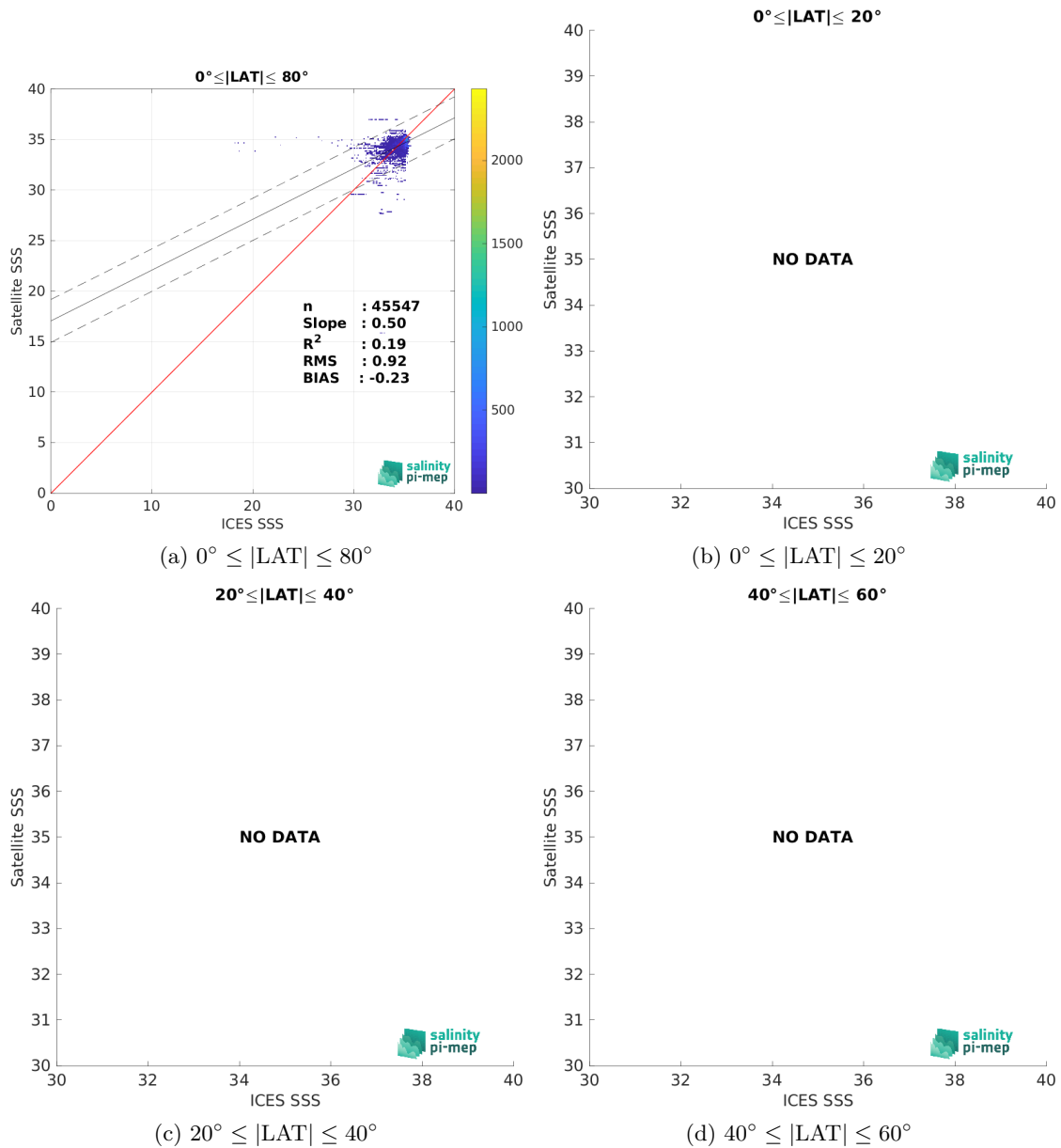
Figure 10: Contour maps of the concentration of Aquarius SSS L3 OR v5 - Monthly - Rain mask (NASA-GSFC) SSS (y-axis) versus ICES SSS (x-axis) at match-up pairs for different latitude bands. For each plot, the red line shows x=y . The black thin and dashed lines indicate a linear fit through the data cloud and the \pm 95\% confidence levels, respectively. The number match-up pairs n , the slope and R^2 coefficient of the linear fit, the root mean square (RMS) and the mean bias between satellite and in situ data are indicated for each latitude band in each plots.
