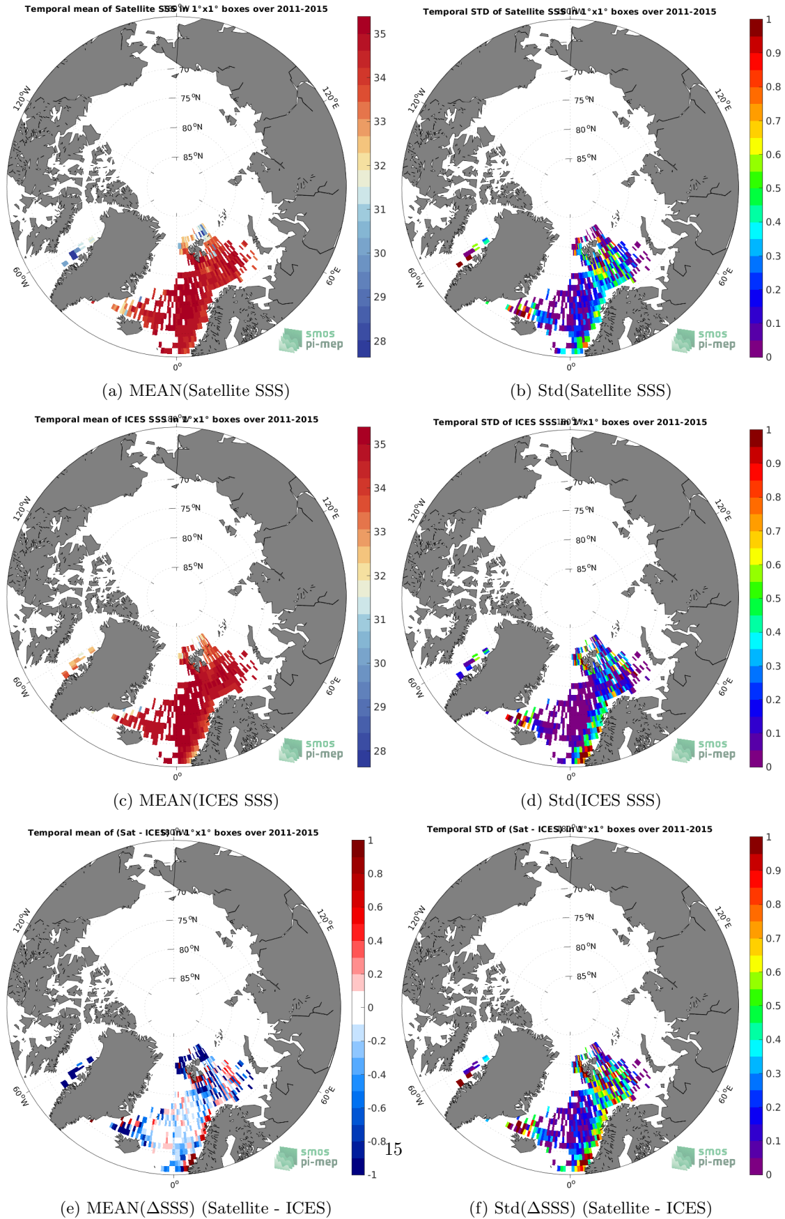
Figure 6: Temporal mean (left) and Std (right) of SSS from Aquarius SSS L3 OR v5 - Monthly - Rain mask (NASA-GSFC) (top), ICES (middle), and of \Delta SSS (Satellite - ICES). Only match-up pairs are used to generate these maps.
