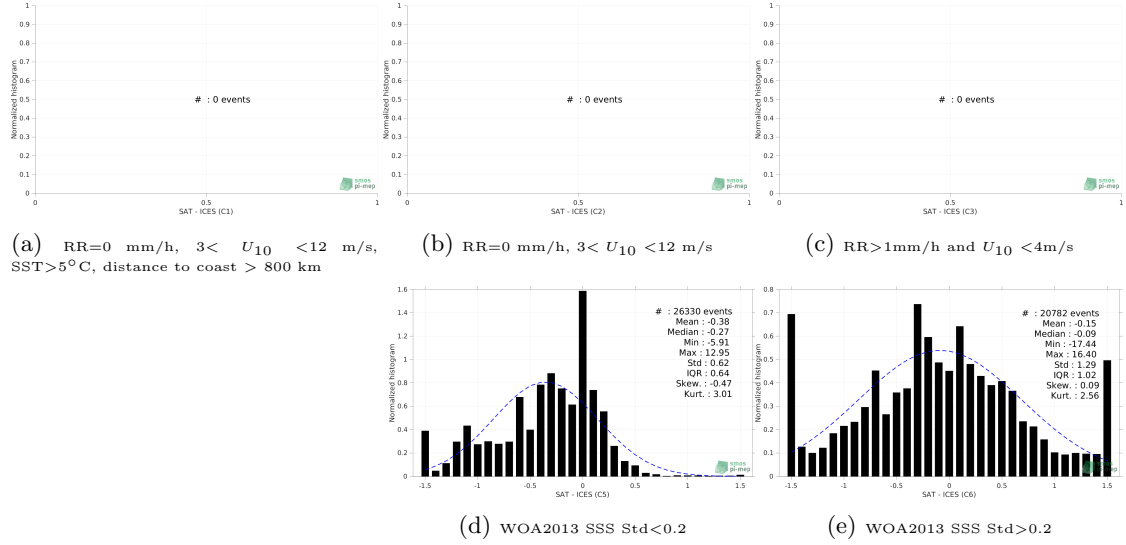
Figure 13: Normalized histogram of \Delta SSS (Aquarius SSS L3 OR v5 - Monthly - Rain mask (NASA-GSFC) - ICES) for 5 different subdatasets corresponding to: RR=0 mm/h, 3 < U_{10} < 12 m/s, SST>5°C, distance to coast > 800 km (a), RR=0 mm/h, 3 < U_{10} < 12 m/s (b), RR>1mm/h and U_{10} < 4 m/s (c), WOA2013 SSS Std<0.2 (d), WOA2013 SSS Std>0.2 (e).
