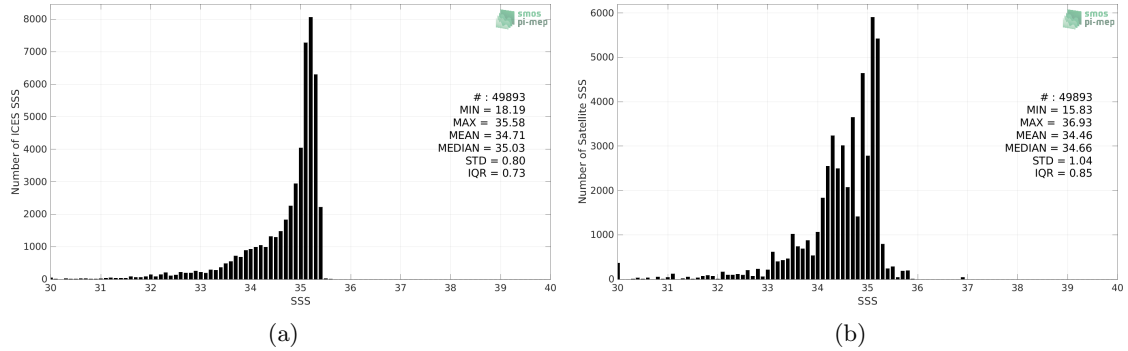
Figure 2: Histograms of SSS from ICES (a) and Aquarius SSS L3 OR v5 - Monthly - Rain mask (NASA-GSFC) (b) considering all match-up pairs per bins of 0.1 over the Arctic Ocean Pi-MEP region and for the full satellite product period.
