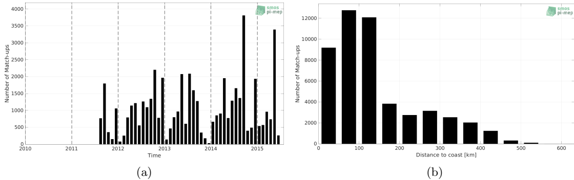
Figure 1: Number of match-ups between ICES and Aquarius SSS L3 OR v5 - Monthly - Rain mask (NASA-GSFC) SSS as a function of time (a) and as function of the distance to coast (b) over the Arctic Ocean Pi-MEP region and for the full satellite product period.
