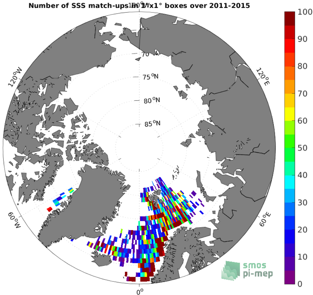
Figure 4: Number of SSS match-ups between ICES SSS and the Aquarius SSS L3 OR v5 - Monthly - Rain mask (NASA-GSFC) SSS product for the Arctic Ocean Pi-MEP region over 1^\circ \times 1^\circ boxes and for the full satellite product period.
