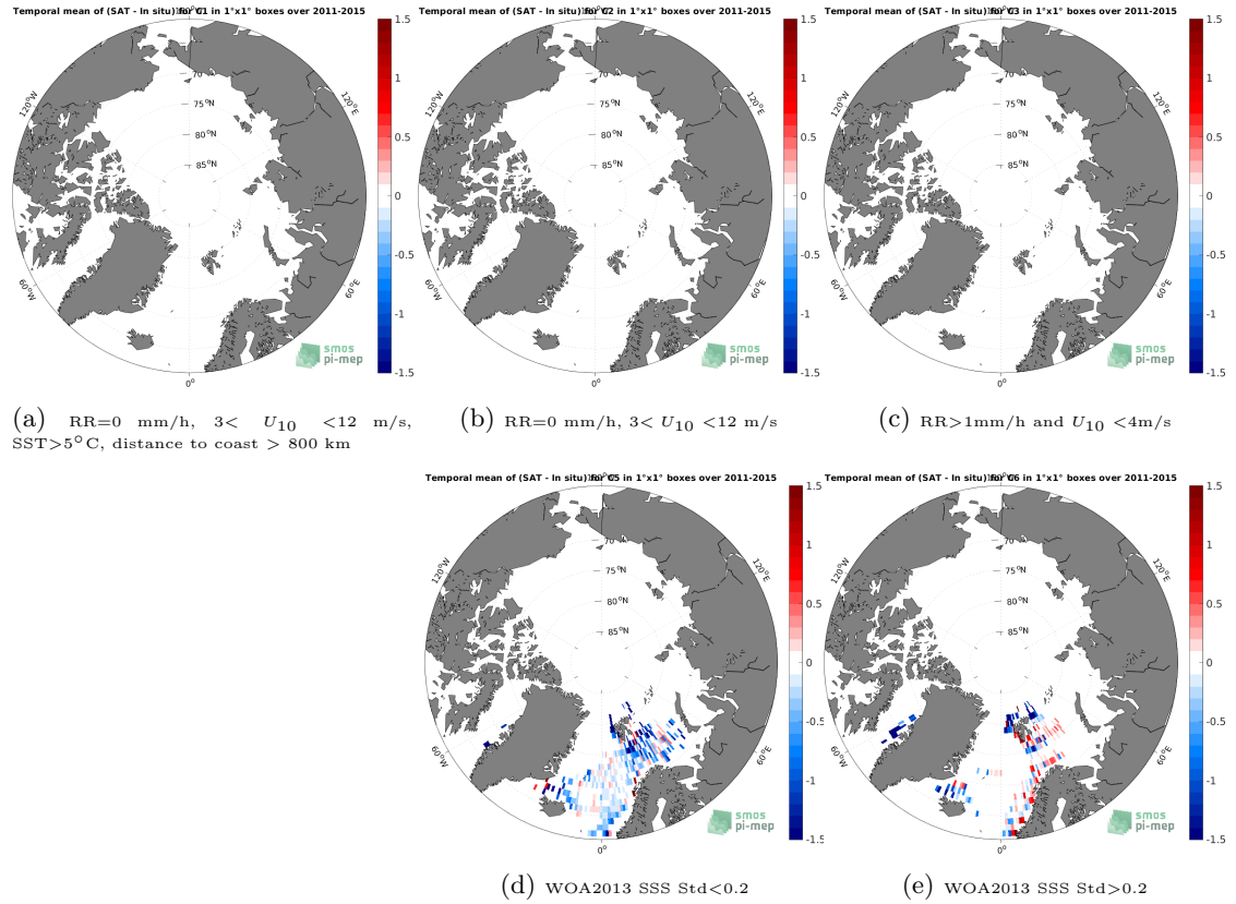
Figure 12: Temporal mean gridded over spatial boxes of size 1^{\circ}\times 1^{\circ} of \Delta\text{SSS} (Aquarius SSS L3 OR v5 - Monthly - Rain mask (NASA-GSFC) - ICES) for 5 different subdatasets corresponding to: RR=0 mm/h, 3 < U_{10} < 12 m/s, SST > 5^{\circ}\text{C} , distance to coast > 800 km (a), RR=0 mm/h, 3 < U_{10} < 12 m/s (b), RR > 1 mm/h and U_{10} < 4 m/s (c), WOA2013 SSS Std < 0.2 (d), WOA2013 SSS Std > 0.2 (e).
