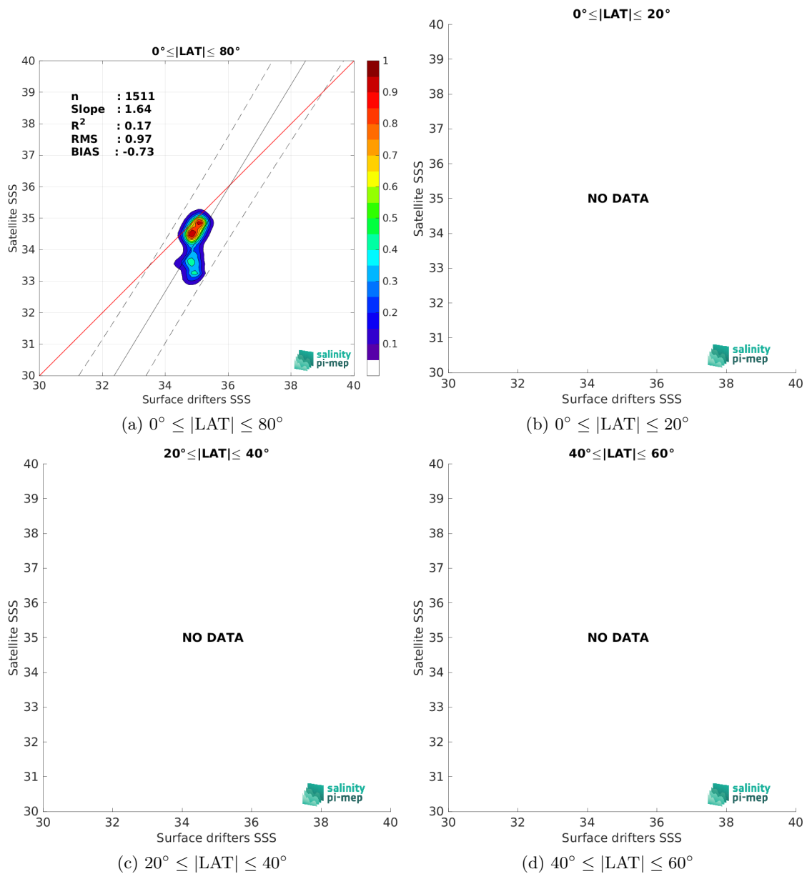
Figure 8: Contour maps of the concentration of Aquarius SSS L3 OR v5 - Monthly - Rain mask (NASA-GSFC) SSS (y-axis) versus Surface drifters SSS (x-axis) at match-up pairs for different latitude bands. For each plot, the red line shows x=y . The black thin and dashed lines indicate a linear fit through the data cloud and the \pm 95\% confidence levels, respectively. The number match-up pairs n , the slope and R^2 coefficient of the linear fit, the root mean square (RMS) and the mean bias between satellite and in situ data are indicated for each latitude band in each plots.
