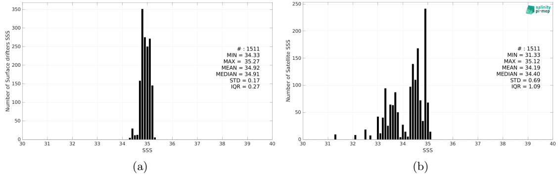
Figure 2: Histograms of SSS from Surface drifters (a) and Aquarius SSS L3 OR v5 - Monthly - Rain mask (NASA-GSFC) (b) considering all match-up pairs per bins of 0.1 over the Arctic Ocean Pi-MEP region and for the full satellite product period.
