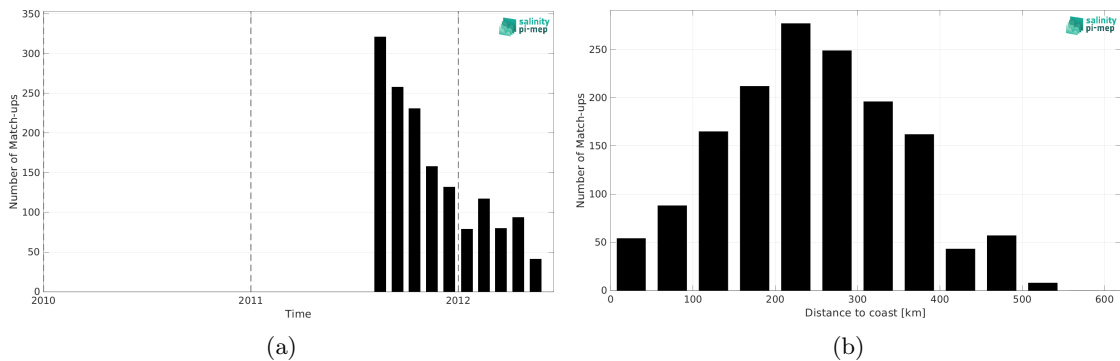
Figure 1: Number of match-ups between Surface drifters and Aquarius SSS L3 OR v5 - Monthly - Rain mask (NASA-GSFC) SSS as a function of time (a) and as function of the distance to coast (b) over the Arctic Ocean Pi-MEP region and for the full satellite product period.
