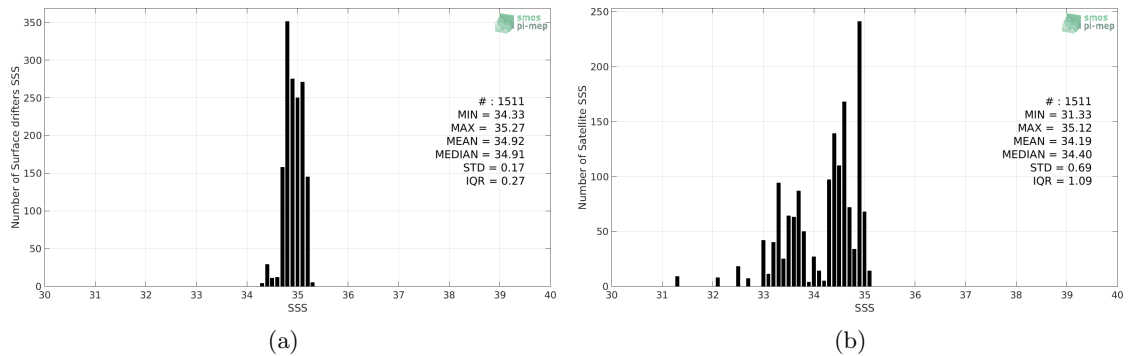
Figure 2: Histograms of SSS from Surface drifters (a) and Aquarius-L3-OR-V5-MONTHLY-RAIN-MASK-1DEG (b) considering all match-up pairs per bins of 0.1 over the Arctic Ocean Pi-MEP region and for the full satellite product period.
