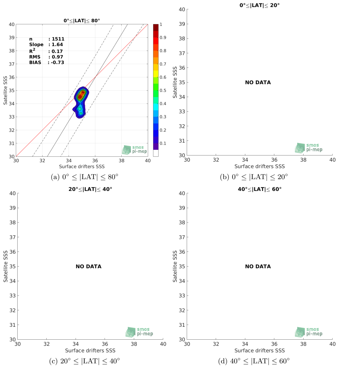
Figure 8: Contour maps of the concentration of Aquarius-L3-OR-V5-MONTHLY-RAIN-MASK-1DEG SSS (y-axis) versus Surface drifters SSS (x-axis) at match-up pairs for different latitude bands. For each plot, the red line shows x=y . The black thin and dashed lines indicate a linear fit through the data cloud and the \pm 95\% confidence levels, respectively. The number match-up pairs n , the slope and R^2 coefficient of the linear fit, the root mean square (RMS) and the mean bias between satellite and in situ data are indicated for each latitude band in each plots.
