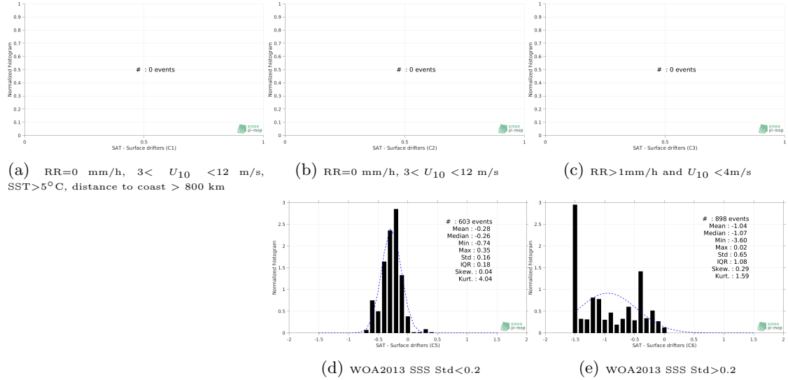
Figure 12: Normalized histogram of \Delta\text{SSS} (Aquarius-L3-OR-V5-MONTHLY-RAIN-MASK-1DEG - Surface drifters) for 5 different subdatasets corresponding to: RR=0 mm/h, 3 < U_{10} < 12 m/s, SST > 5^\circ\text{C} , distance to coast > 800 km (a), RR=0 mm/h, 3 < U_{10} < 12 m/s (b), RR > 1\text{mm/h} and U_{10} < 4\text{m/s} (c), WOA2013 SSS Std < 0.2 (d), WOA2013 SSS Std > 0.2 (e).
