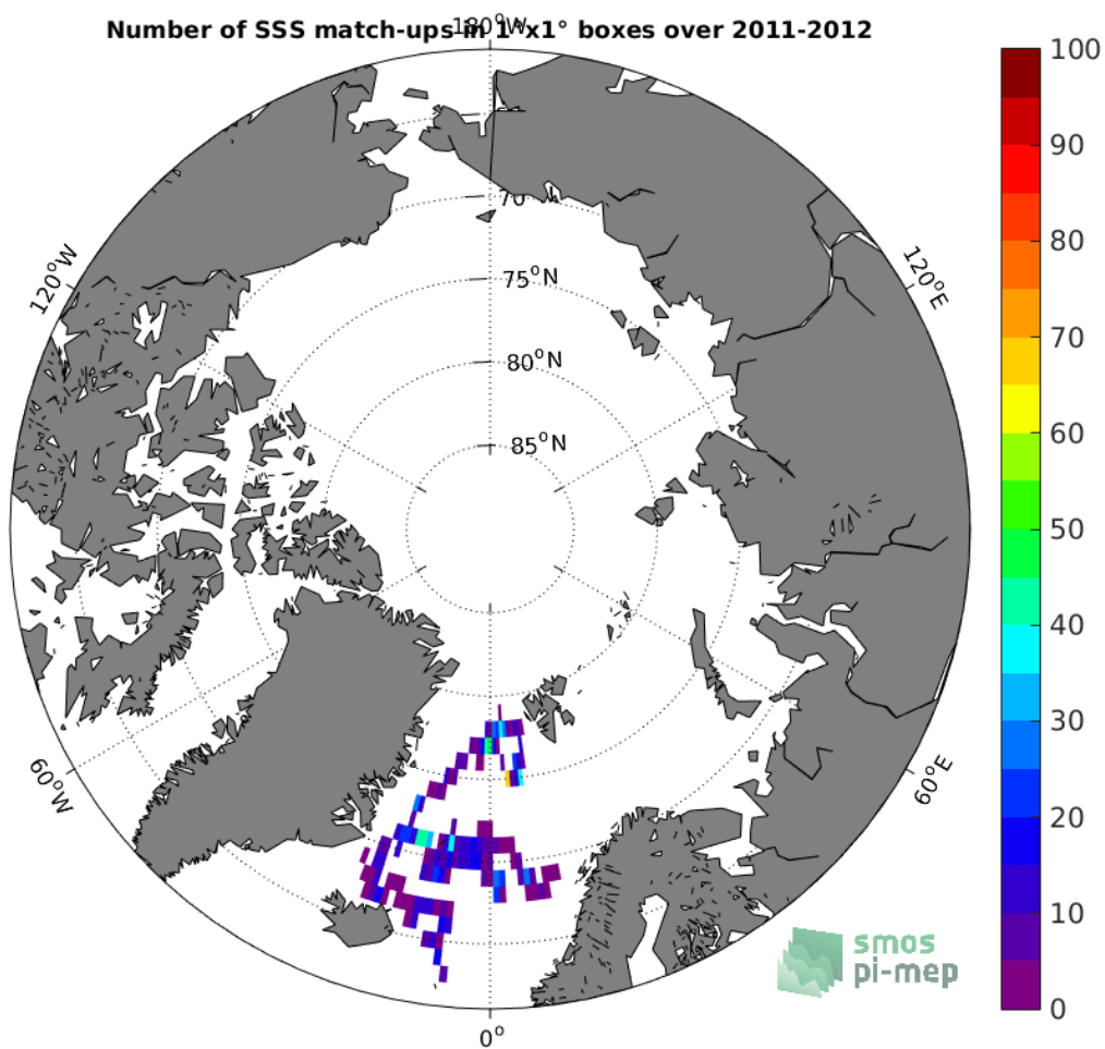
Figure 3: Number of SSS match-ups between Surface drifters SSS and the Aquarius-L3-OR-V5-MONTHLY-RAIN-MASK-1DEG SSS product for the Arctic Ocean Pi-MEP region over 1^\circ \times 1^\circ boxes and for the full satellite product period.
