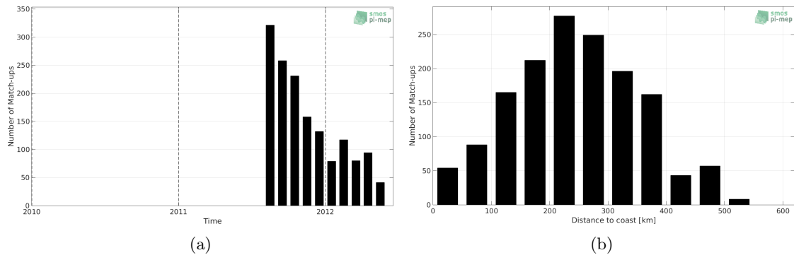
Figure 1: Number of match-ups between Surface drifters and Aquarius-L3-OR-V5-MONTHLY-RAIN-MASK-1DEG SSS as a function of time (a) and as function of the distance to coast (b) over the Arctic Ocean Pi-MEP region and for the full satellite product period.
