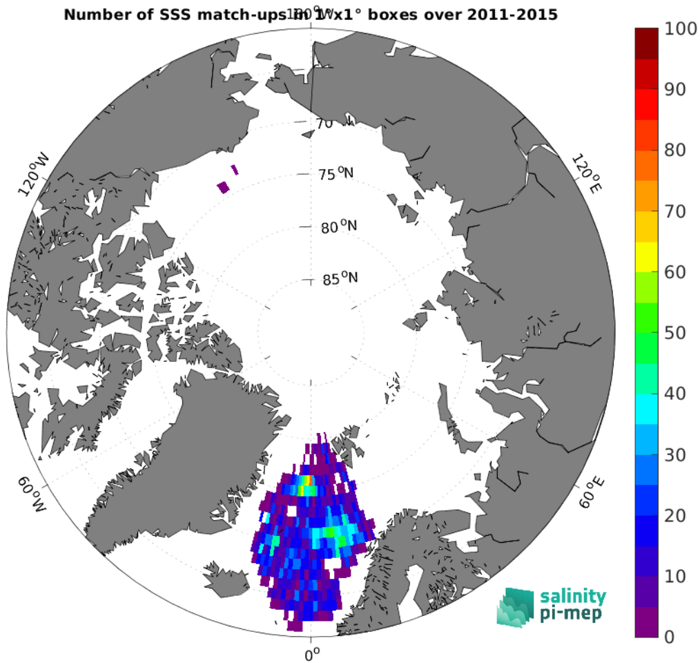
Figure 5: Number of SSS match-ups between Argo SSS and the Aquarius SSS L3 OR v5 - Monthly - Rain mask (NASA-GSFC) SSS product for the Arctic Ocean Pi-MEP region over 1^{\circ} \times 1^{\circ} boxes and for the full satellite product period.
