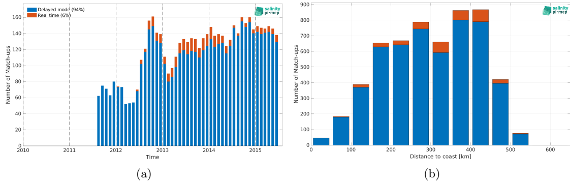
Figure 2: Number of match-ups between Argo and Aquarius SSS L3 OR v5 - Monthly - Rain mask (NASA-GSFC) SSS as a function of time (a) and as function of the distance to coast (b) over the Arctic Ocean Pi-MEP region and for the full satellite product period.
