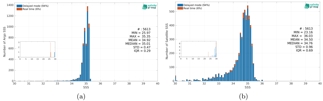
Figure 3: Histograms of SSS from Argo (a) and Aquarius SSS L3 OR v5 - Monthly - Rain mask (NASA-GSFC) (b) considering all match-up pairs per bins of 0.1 over the Arctic Ocean Pi-MEP region and for the full satellite product period.
