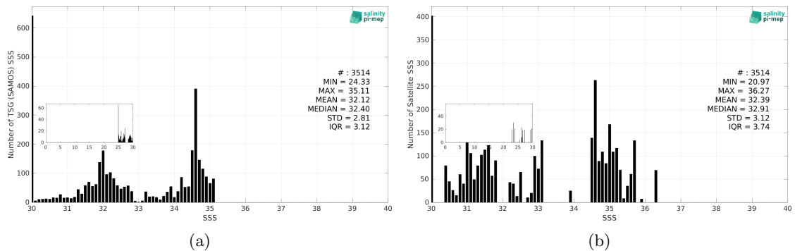
Figure 3: Histograms of SSS from TSG (SAMOS) (a) and Aquarius SSS L3 CAP v5 - 7-Day running (JPL) (b) considering all match-up pairs per bins of 0.1 over the Arctic Ocean Pi-MEP region and for the full satellite product period.
