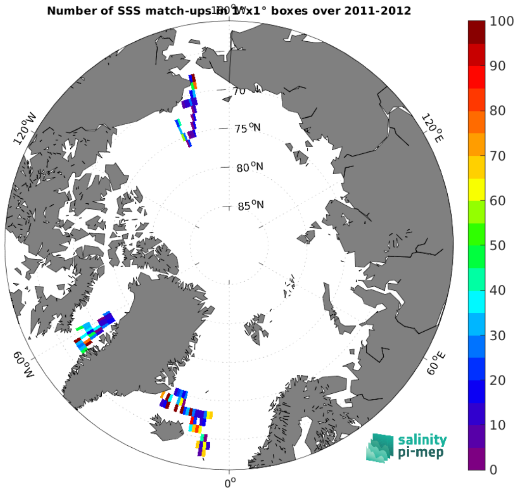
Figure 5: Number of SSS match-ups between TSG (SAMOS) SSS and the Aquarius SSS L3 CAP v5 - 7-Day running (JPL) SSS product for the Arctic Ocean Pi-MEP region over 1^\circ \times 1^\circ boxes and for the full satellite product period.
