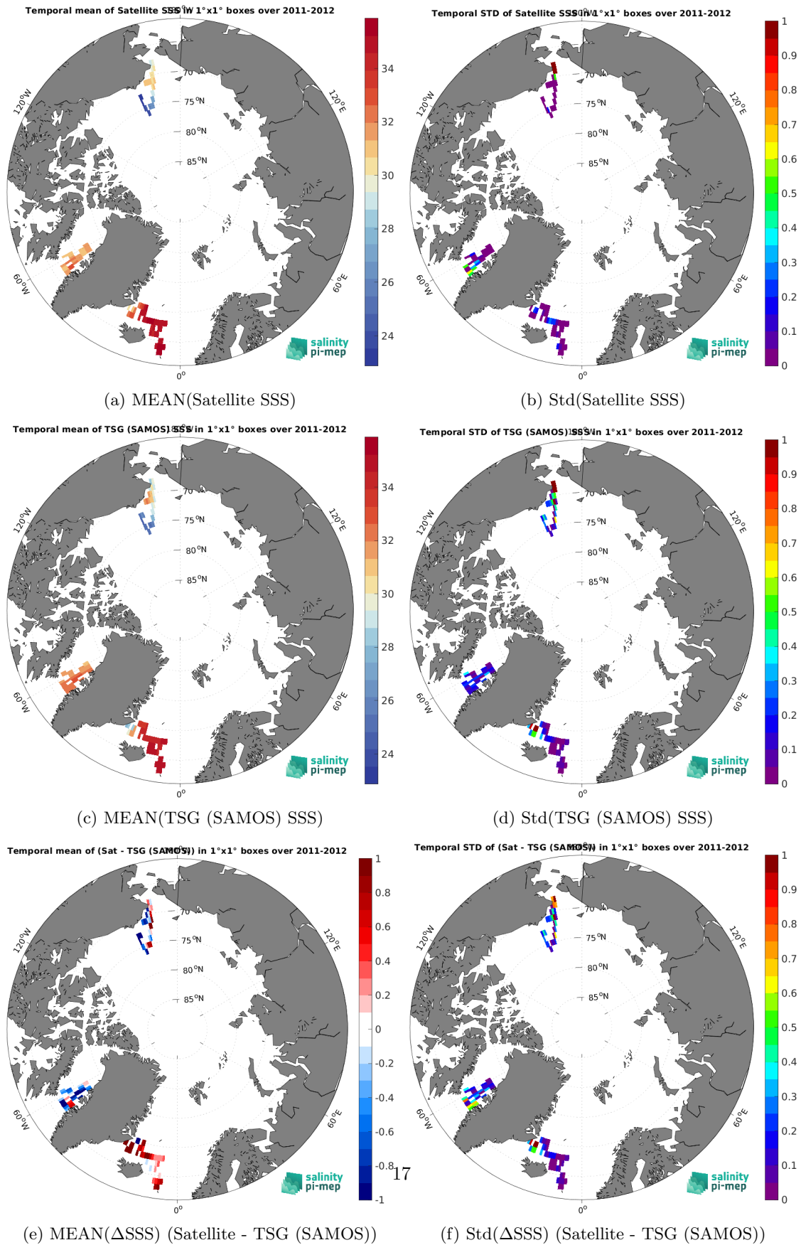
Figure 7: Temporal mean (left) and Std (right) of SSS from Aquarius SSS L3 CAP v5 - 7-Day running (JPL) (top), TSG (SAMOS) (middle), and of \Delta SSS (Satellite - TSG (SAMOS)). Only match-up pairs are used to generate these maps.
