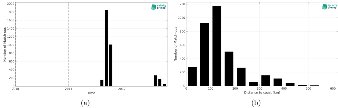
Figure 2: Number of match-ups between TSG (SAMOS) and Aquarius SSS L3 CAP v5 - 7-Day running (JPL) SSS as a function of time (a) and as function of the distance to coast (b) over the Arctic Ocean Pi-MEP region and for the full satellite product period.
