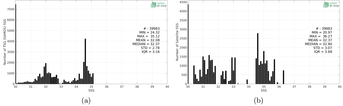
Figure 2: Histograms of SSS from TSG (SAMOS) (a) and Aquarius SSS L3 CAP v5 - 7-Day running (JPL) (b) considering all match-up pairs per bins of 0.1 over the Arctic Ocean Pi-MEP region and for the full satellite product period.
