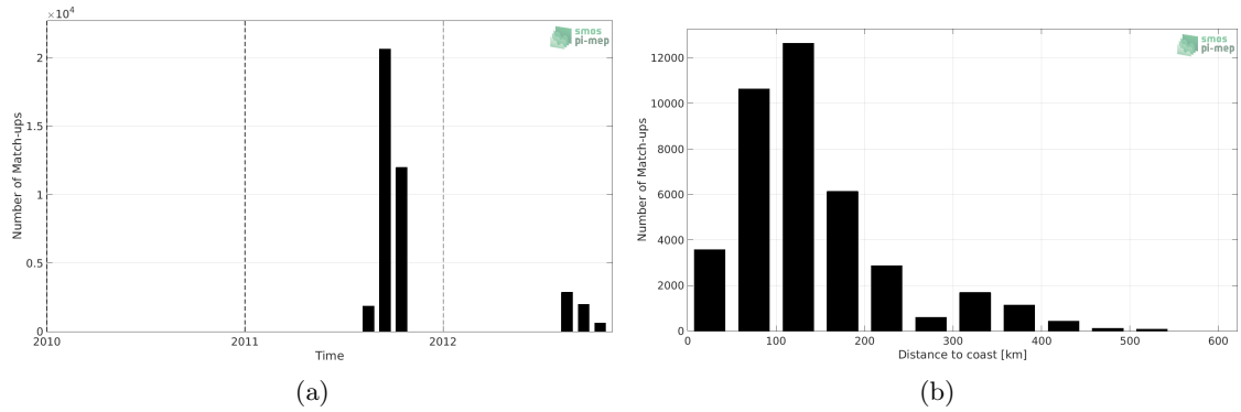
Figure 1: Number of match-ups between TSG (SAMOS) and Aquarius SSS L3 CAP v5 - 7-Day running (JPL) SSS as a function of time (a) and as function of the distance to coast (b) over the Arctic Ocean Pi-MEP region and for the full satellite product period.
