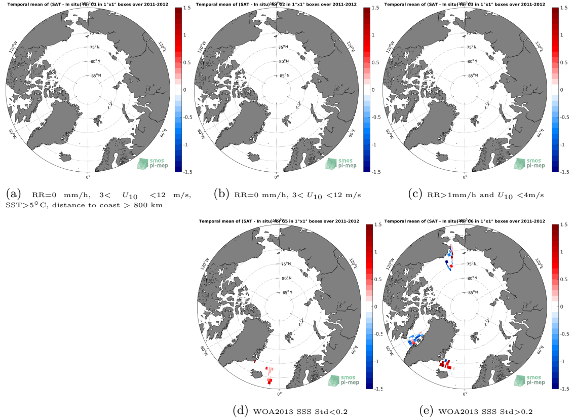
Figure 12: Temporal mean gridded over spatial boxes of size 1^{\circ}\times 1^{\circ} of \Delta\text{SSS} (Aquarius-L3-JPL-V5-7DAY-RUNNING - TSG-SAMOS) for 5 different subdatasets corresponding to: RR=0 mm/h, 3 < U_{10} < 12 m/s, SST >5^{\circ}\text{C} , distance to coast > 800 km (a), RR=0 mm/h, 3 < U_{10} < 12 m/s (b), RR >1 mm/h and U_{10} < 4 m/s (c), WOA2013 SSS Std <0.2 (d), WOA2013 SSS Std >0.2 (e).
