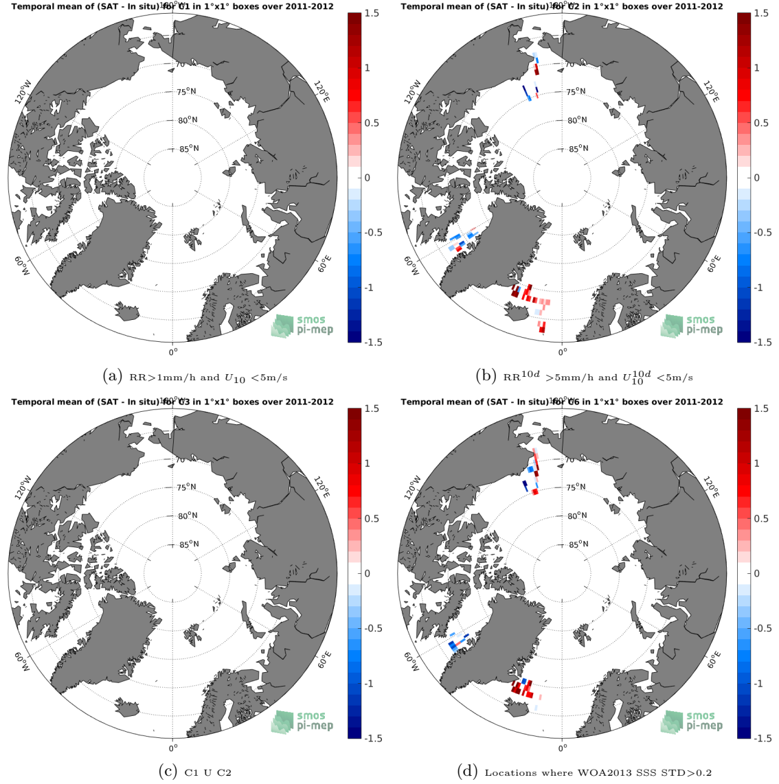
Figure 12: Temporal mean gridded over spatial boxes of size 1^\circ \times 1^\circ of \Delta SSS (Aquarius-L3-JPL-V5-7DAY-RUNNING - TSG-SAMOS) for 4 different subdatasets corresponding to: RR > 1\text{mm/h} and U_{10} < 5\text{m/s} (a), RR^{10d} > 5\text{mm/h} and U_{10}^{10d} < 5\text{m/s} (b), C1 U C2 (c), Locations where WOA2013 SSS STD > 0.2 (d).
