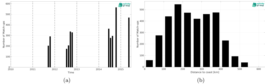
Figure 2: Number of match-ups between TSG (Polarstern) and Aquarius SSS L3 CAP v5 - 7-Day running (JPL) SSS as a function of time (a) and as function of the distance to coast (b) over the Arctic Ocean Pi-MEP region and for the full satellite product period.
