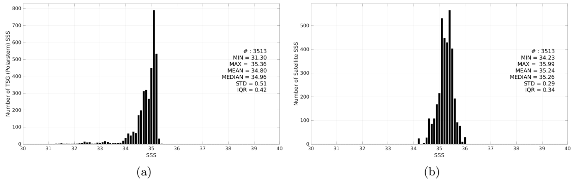
Figure 3: Histograms of SSS from TSG (Polarstern) (a) and Aquarius SSS L3 CAP v5 - 7-Day running (JPL) (b) considering all match-up pairs per bins of 0.1 over the Arctic Ocean Pi-MEP region and for the full satellite product period.
