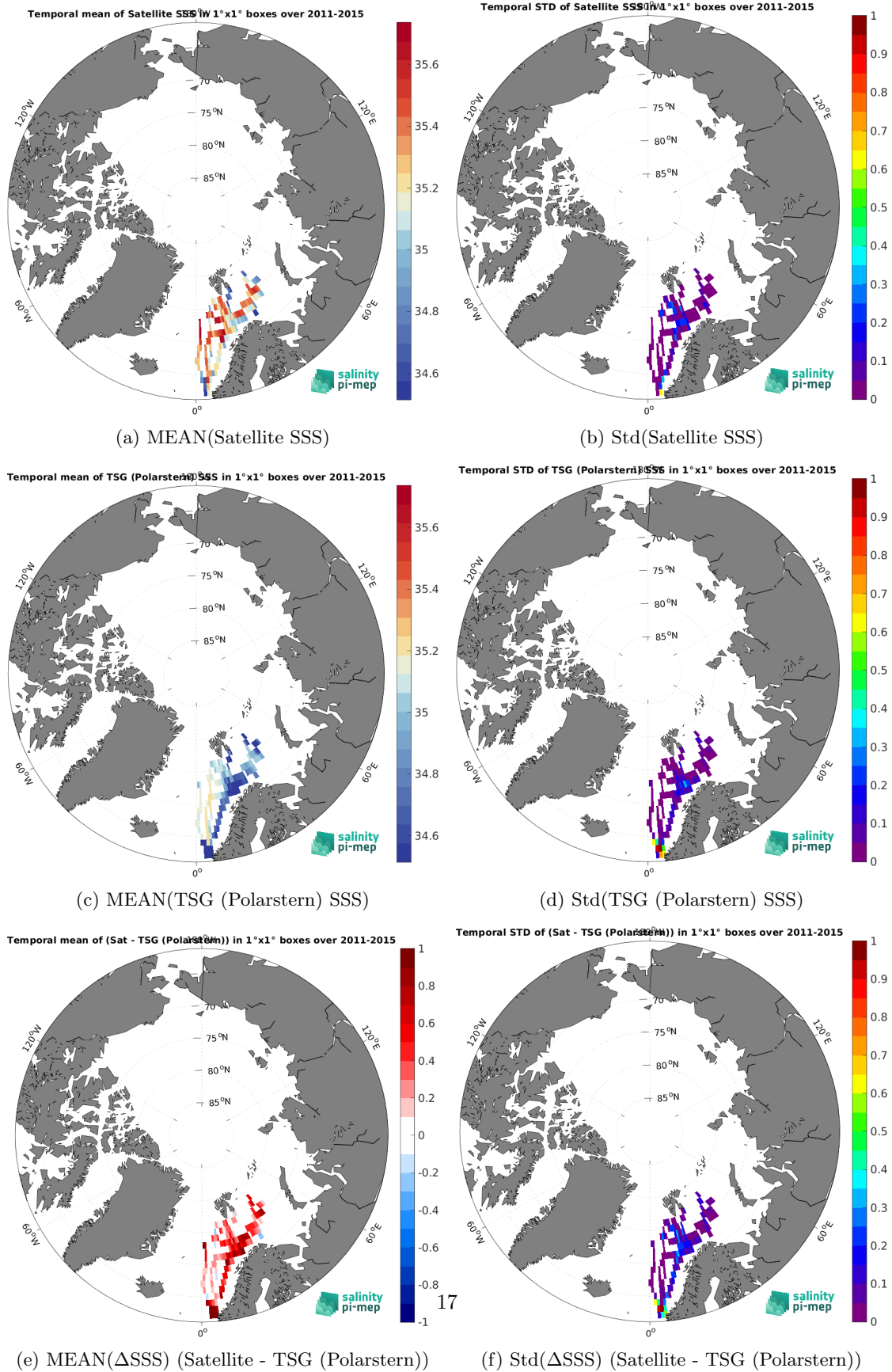
Figure 7: Temporal mean (left) and Std (right) of SSS from Aquarius SSS L3 CAP v5 - 7-Day running (JPL) (top), TSG (Polarstern) (middle), and of \Delta SSS (Satellite - TSG (Polarstern)). Only match-up pairs are used to generate these maps.
