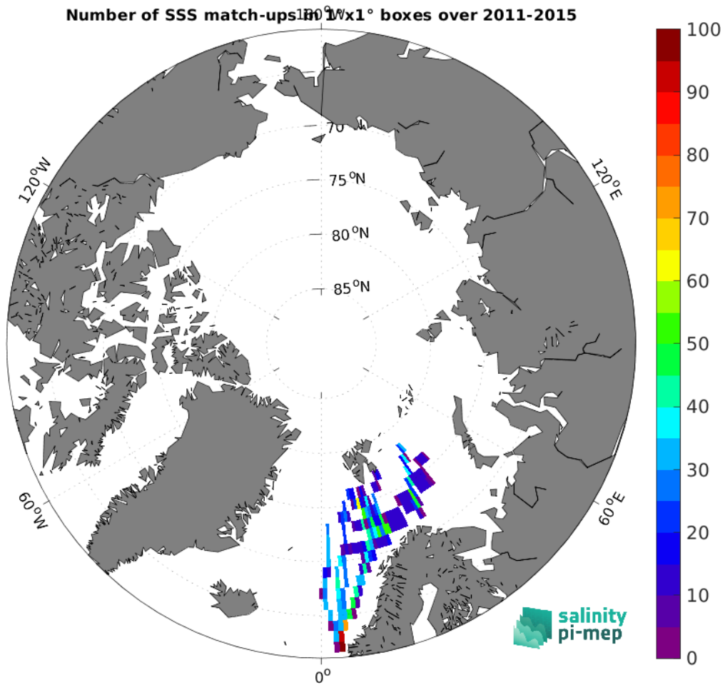
Figure 5: Number of SSS match-ups between TSG (Polarstern) SSS and the Aquarius SSS L3 CAP v5 - 7-Day running (JPL) SSS product for the Arctic Ocean Pi-MEP region over 1^\circ \times 1^\circ boxes and for the full satellite product period.
