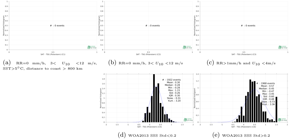
Figure 13: Normalized histogram of \Delta\text{SSS} (Aquarius SSS L3 CAP v5 - 7-Day running (JPL) - TSG (Polarstern)) for 5 different subdatasets corresponding to: RR=0 mm/h, 3 < U_{10} < 12 m/s, SST > 5^\circ\text{C} , distance to coast > 800 km (a), RR=0 mm/h, 3 < U_{10} < 12 m/s (b), RR > 1 mm/h and U_{10} < 4 m/s (c), WOA2013 SSS Std < 0.2 (d), WOA2013 SSS Std > 0.2 (e).
