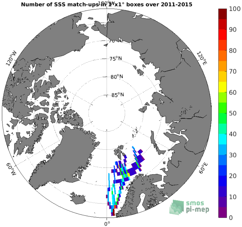
Figure 4: Number of SSS match-ups between TSG (Polarstern) SSS and the Aquarius SSS L3 CAP v5 - 7-Day running (JPL) SSS product for the Arctic Ocean Pi-MEP region over 1°x1° boxes and for the full satellite product period.
