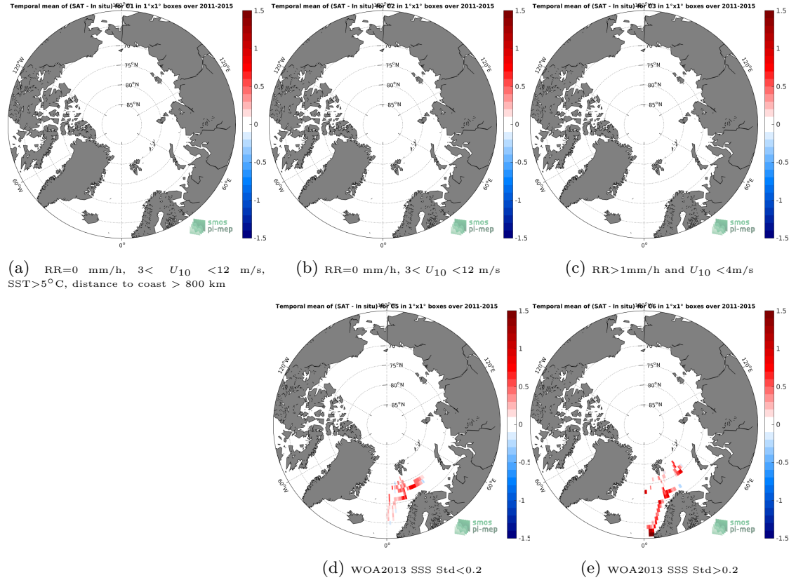
Figure 12: Temporal mean gridded over spatial boxes of size 1^{\circ}\times 1^{\circ} of \Delta\text{SSS} (Aquarius-L3-JPL-V5-7DAY-RUNNING - TSG-POLARSTERN) for 5 different subdatasets corresponding to:RR=0 mm/h, 3 < U_{10} < 12 m/s, SST >5^{\circ}\text{C} , distance to coast > 800 km (a), RR=0 mm/h, 3 < U_{10} < 12 m/s (b), RR >1 mm/h and U_{10} < 4 m/s (c), WOA2013 SSS Std <0.2 (d), WOA2013 SSS Std >0.2 (e).
