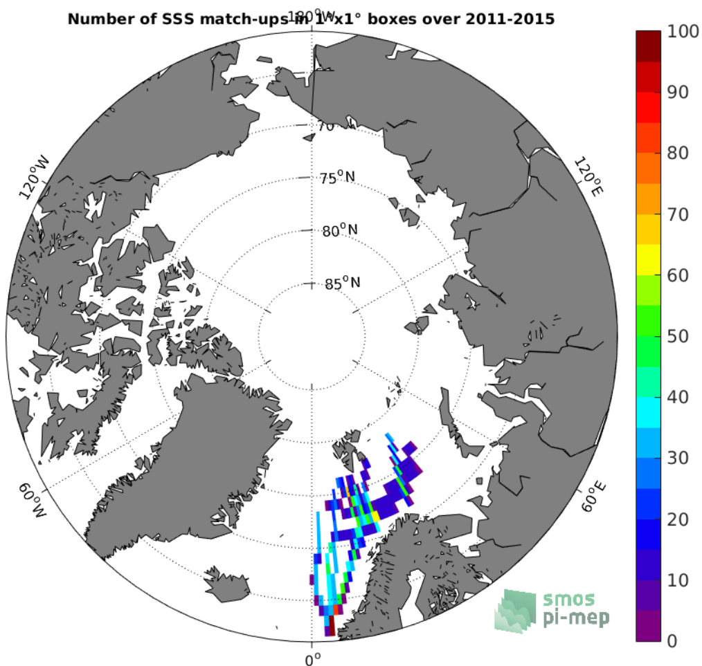
Figure 4: Number of SSS match-ups between TSG-POLARSTERN SSS and the Aquarius-L3-JPL-V5-7DAY-RUNNING SSS product for the Arctic Ocean Pi-MEP region over 1^\circ \times 1^\circ boxes and for the full satellite product period.
