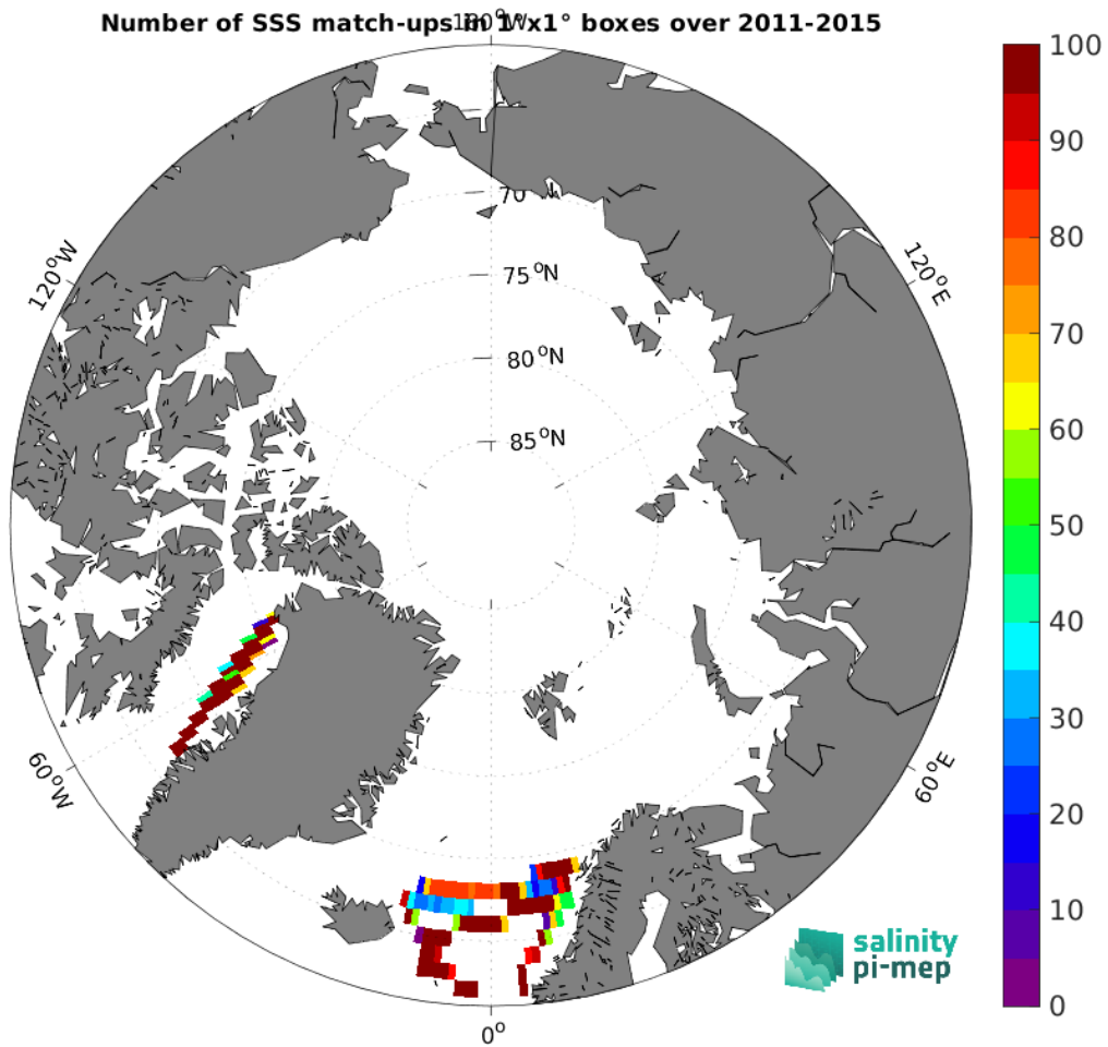
Figure 5: Number of SSS match-ups between TSG (LEGOS-DM) SSS and the Aquarius SSS L3 CAP v5 - 7-Day running (JPL) SSS product for the Arctic Ocean Pi-MEP region over 1^\circ \times 1^\circ boxes and for the full satellite product period.
