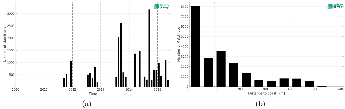
Figure 2: Number of match-ups between TSG (LEGOS-DM) and Aquarius SSS L3 CAP v5 - 7-Day running (JPL) SSS as a function of time (a) and as function of the distance to coast (b) over the Arctic Ocean Pi-MEP region and for the full satellite product period.
