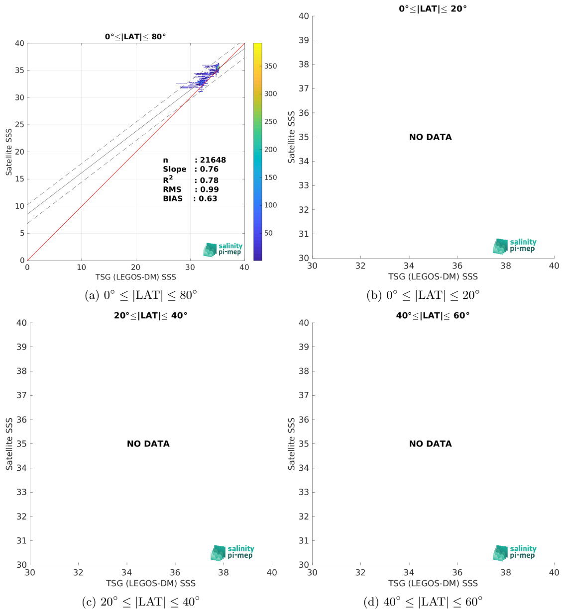
Figure 10: Contour maps of the concentration of Aquarius SSS L3 CAP v5 - 7-Day running (JPL) SSS (y-axis) versus TSG (LEGOS-DM) SSS (x-axis) at match-up pairs for different latitude bands. For each plot, the red line shows x=y . The black thin and dashed lines indicate a linear fit through the data cloud and the \pm 95\% confidence levels, respectively. The number match-up pairs n , the slope and R^2 coefficient of the linear fit, the root mean square (RMS) and the mean bias between satellite and in situ data are indicated for each latitude band in each plots.
