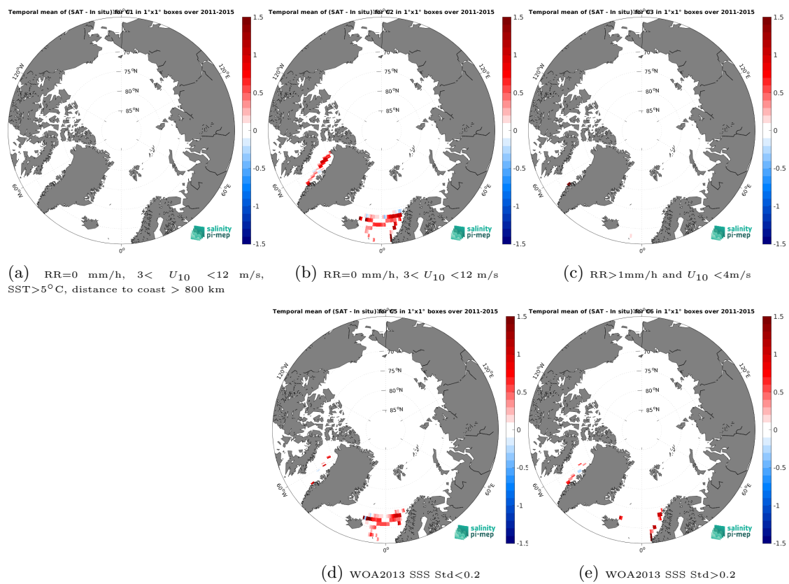
Figure 14: Temporal mean gridded over spatial boxes of size 1^\circ \times 1^\circ of \Delta\text{SSS} (Aquarius SSS L3 CAP v5 - 7-Day running (JPL) - TSG (LEGOS-DM)) for 5 different subdatasets corresponding to: RR=0 mm/h, 3 < U_{10} < 12 m/s, SST > 5°C, distance to coast > 800 km (a), RR=0 mm/h, 3 < U_{10} < 12 m/s (b), RR > 1mm/h and U_{10} < 4 m/s (c), WOA2013 SSS Std < 0.2 (d), WOA2013 SSS Std > 0.2 (e).
