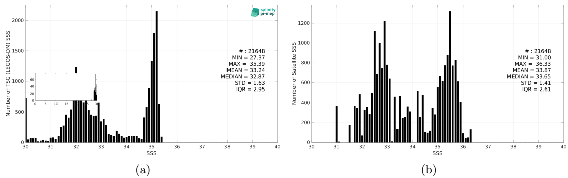
Figure 3: Histograms of SSS from TSG (LEGOS-DM) (a) and Aquarius SSS L3 CAP v5 - 7-Day running (JPL) (b) considering all match-up pairs per bins of 0.1 over the Arctic Ocean Pi-MEP region and for the full satellite product period.
