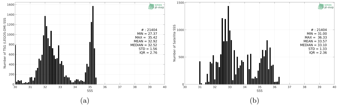
Figure 2: Histograms of SSS from TSG (LEGOS-DM) (a) and Aquarius SSS L3 CAP v5 - 7-Day running (JPL) (b) considering all match-up pairs per bins of 0.1 over the Arctic Ocean Pi-MEP region and for the full satellite product period.
