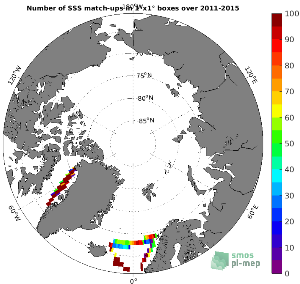
Figure 4: Number of SSS match-ups between TSG (LEGOS-DM) SSS and the Aquarius SSS L3 CAP v5 - 7-Day running (JPL) SSS product for the Arctic Ocean Pi-MEP region over 1°x1° boxes and for the full satellite product period.
