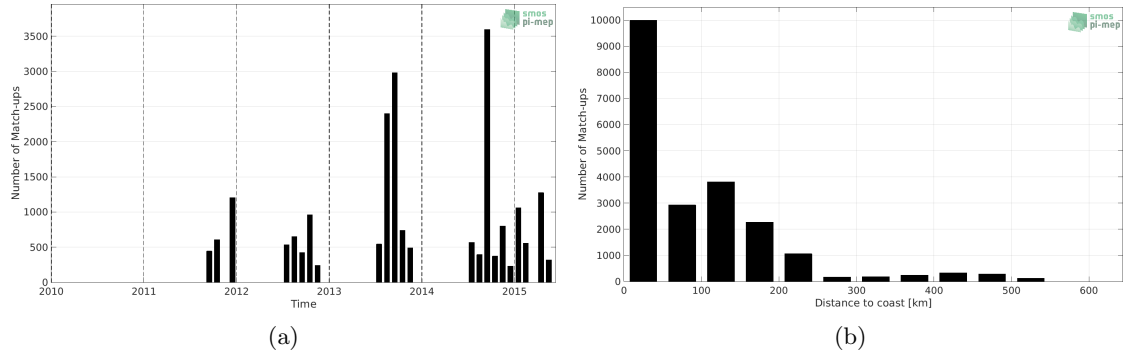
Figure 1: Number of match-ups between TSG (LEGOS-DM) and Aquarius SSS L3 CAP v5 - 7-Day running (JPL) SSS as a function of time (a) and as function of the distance to coast (b) over the Arctic Ocean Pi-MEP region and for the full satellite product period.
