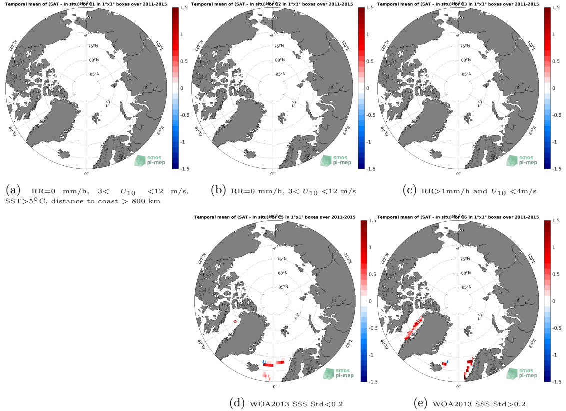
Figure 12: Temporal mean gridded over spatial boxes of size 1^{\circ}\times 1^{\circ} of \Delta\text{SSS} (Aquarius SSS L3 CAP v5 - 7-Day running (JPL) - TSG (LEGOS-DM)) for 5 different subdatasets corresponding to: RR=0 mm/h, 3 < U_{10} < 12 m/s, SST > 5^{\circ}\text{C} , distance to coast > 800 km (a), RR=0 mm/h, 3 < U_{10} < 12 m/s (b), RR > 1 mm/h and U_{10} < 4 m/s (c), WOA2013 SSS Std < 0.2 (d), WOA2013 SSS Std > 0.2 (e).
