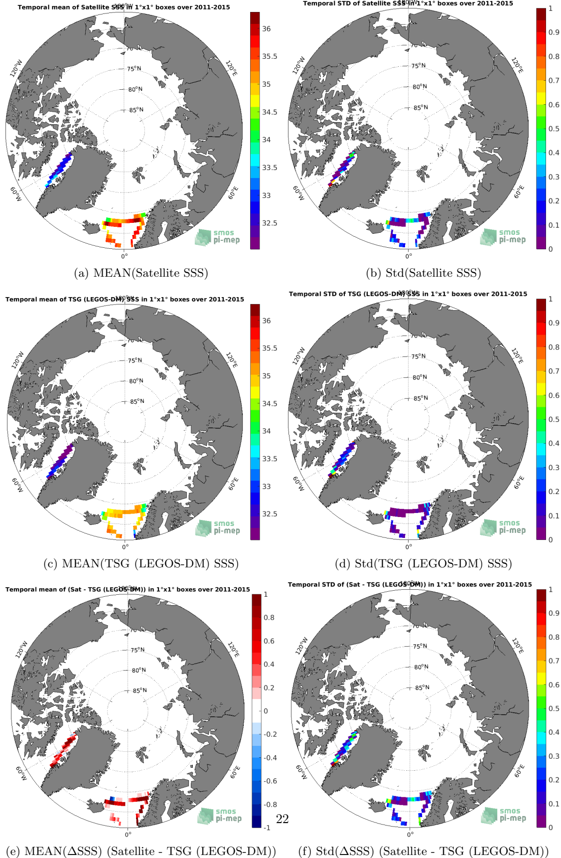
Figure 6: Temporal mean (left) and Std (right) of SSS from Aquarius SSS L3 CAP v5 - 7-Day running (JPL) (top), TSG (LEGOS-DM) (middle), and of \Delta SSS (Satellite - TSG (LEGOS-DM)). Only match-up pairs are used to generate these maps.
