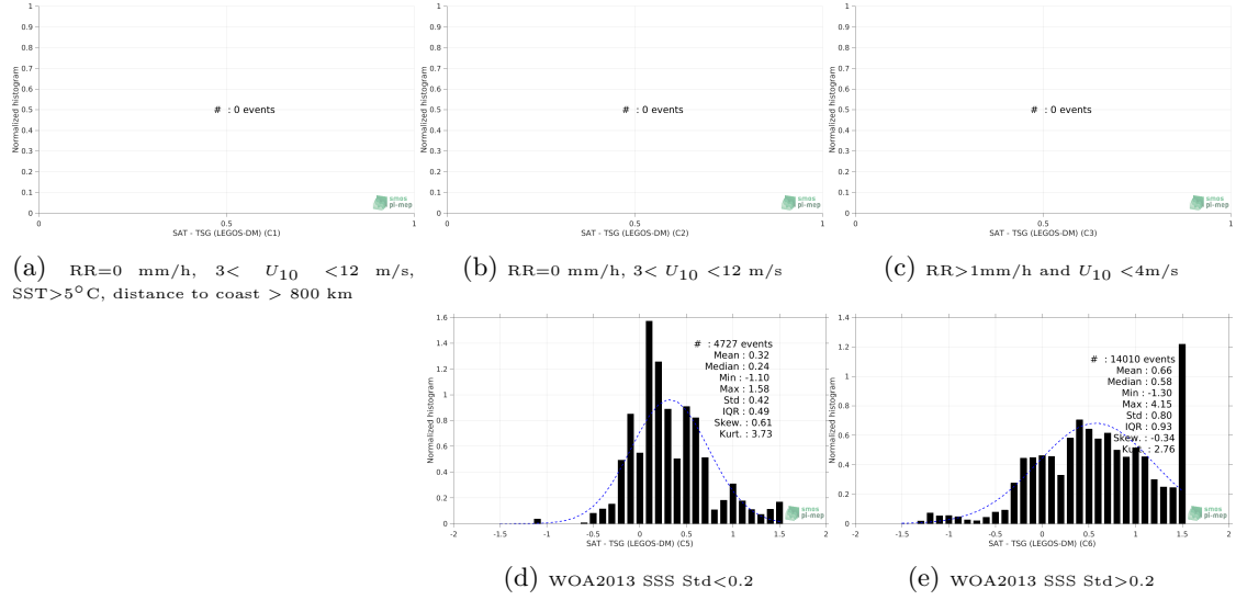
Figure 13: Normalized histogram of \Delta\text{SSS} (Aquarius SSS L3 CAP v5 - 7-Day running (JPL) - TSG (LEGOS-DM)) for 5 different subdatasets corresponding to: RR=0 mm/h, 3 < U_{10} < 12 m/s, SST > 5^\circ\text{C} , distance to coast > 800 km (a), RR=0 mm/h, 3 < U_{10} < 12 m/s (b), RR > 1 mm/h and U_{10} < 4 m/s (c), WOA2013 SSS Std < 0.2 (d), WOA2013 SSS Std > 0.2 (e).
