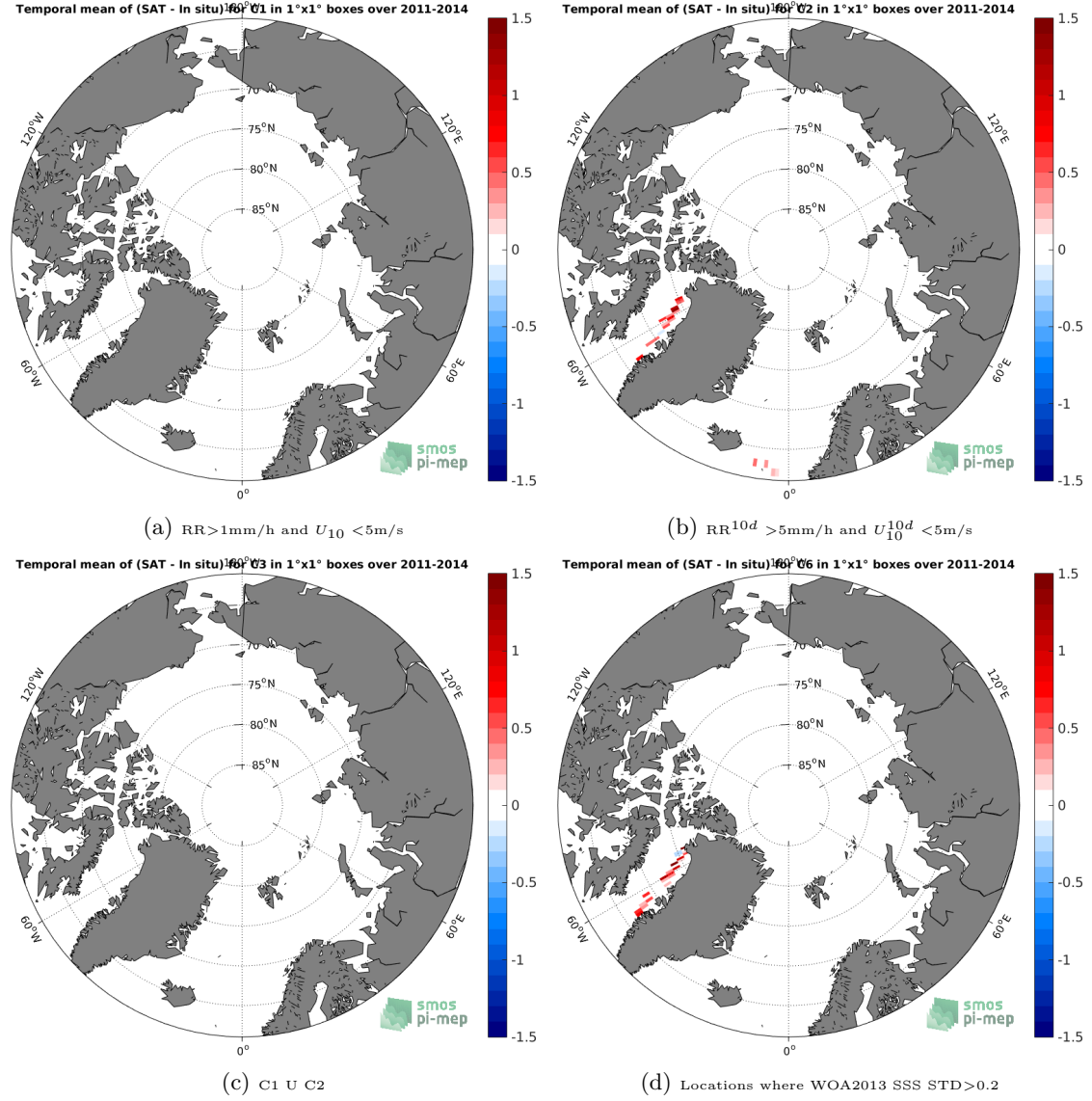
Figure 12: Temporal mean gridded over spatial boxes of size 1^\circ \times 1^\circ of \Delta SSS (Aquarius-L3-JPL-V5-7DAY-RUNNING - TSG-LEGOS-DM) for 4 different subdatasets corresponding to: RR > 1\text{mm/h} and U_{10} < 5\text{m/s} (a), RR^{10d} > 5\text{mm/h} and U_{10}^{10d} < 5\text{m/s} (b), C1 U C2 (c), Locations where WOA2013 SSS STD > 0.2 (d).
