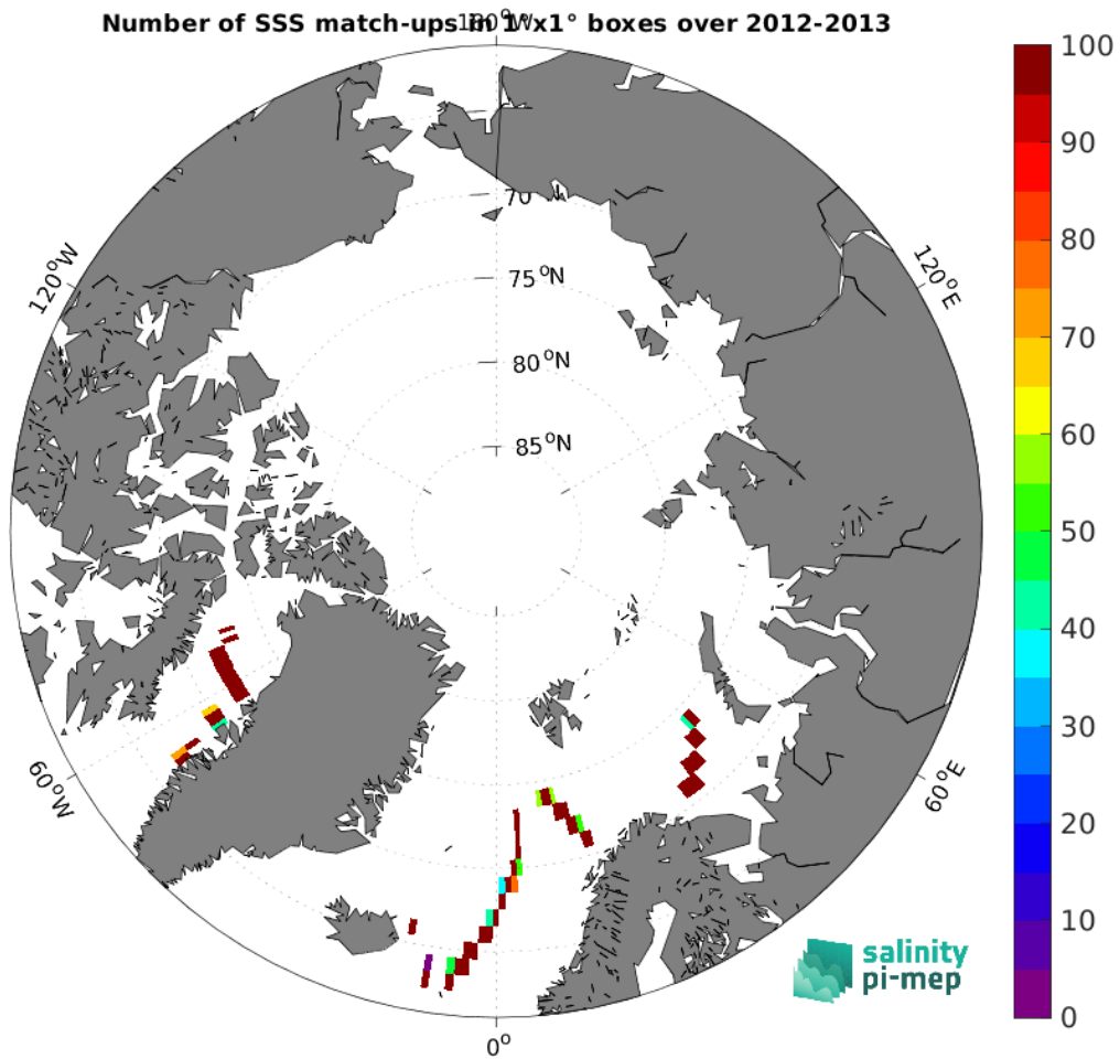
Figure 4: Number of SSS match-ups between TSG (GOSUD-Sailing-ship) SSS and the Aquarius SSS L3 CAP v5 - 7-Day running (JPL) SSS product for the Arctic Ocean Pi-MEP region over 1^{\circ} \times 1^{\circ} boxes and for the full satellite product period.
