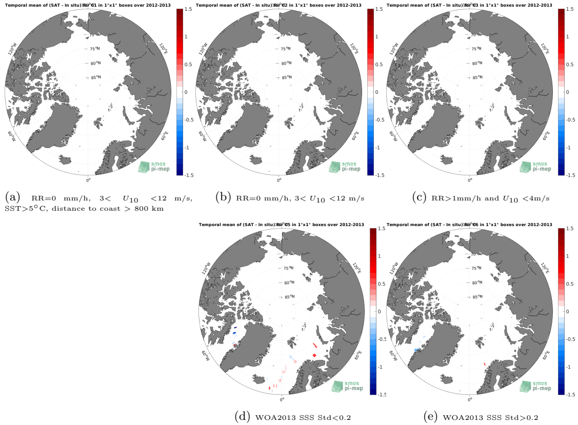
Figure 12: Temporal mean gridded over spatial boxes of size 1^\circ \times 1^\circ of \Delta SSS (Aquarius SSS L3 CAP v5 - 7-Day running (JPL) - TSG (GOSUD-Sailing-ship)) for 5 different subdatasets corresponding to: RR=0 mm/h, 3 < U_{10} < 12 m/s, SST>5°C, distance to coast > 800 km (a), RR=0 mm/h, 3 < U_{10} < 12 m/s (b), RR>1mm/h and U_{10} < 4 m/s (c), WOA2013 SSS Std<0.2 (d), WOA2013 SSS Std>0.2 (e).
