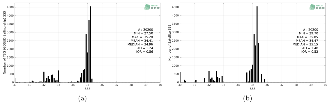
Figure 2: Histograms of SSS from TSG (GOSUD-Sailing-ship) (a) and Aquarius SSS L3 CAP v5 - 7-Day running (JPL) (b) considering all match-up pairs per bins of 0.1 over the Arctic Ocean Pi-MEP region and for the full satellite product period.
