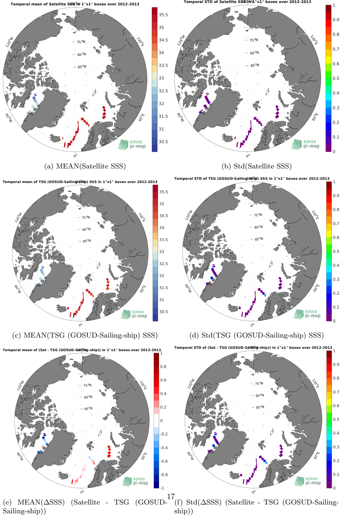
Figure 6: Temporal mean (left) and Std (right) of SSS from Aquarius SSS L3 CAP v5 - 7-Day running (JPL) (top), TSG (GOSUD-Sailing-ship) (middle), and of \Delta SSS (Satellite - TSG (GOSUD-Sailing-ship)). Only match-up pairs are used to generate these maps.
