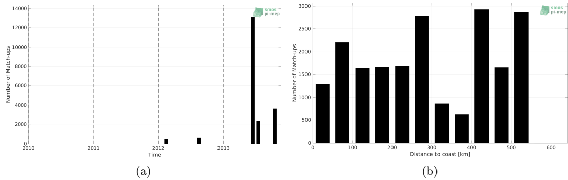
Figure 1: Number of match-ups between TSG (GOSUD-Sailing-ship) and Aquarius SSS L3 CAP v5 - 7-Day running (JPL) SSS as a function of time (a) and as function of the distance to coast (b) over the Arctic Ocean Pi-MEP region and for the full satellite product period.
