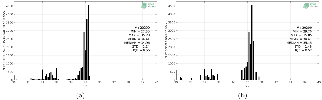
Figure 2: Histograms of SSS from TSG-GOSUD-Sailing-ship (a) and Aquarius-L3-JPL-V5-7DAY-RUNNING (b) considering all match-up pairs per bins of 0.1 over the Arctic Ocean Pi-MEP region and for the full satellite product period.
