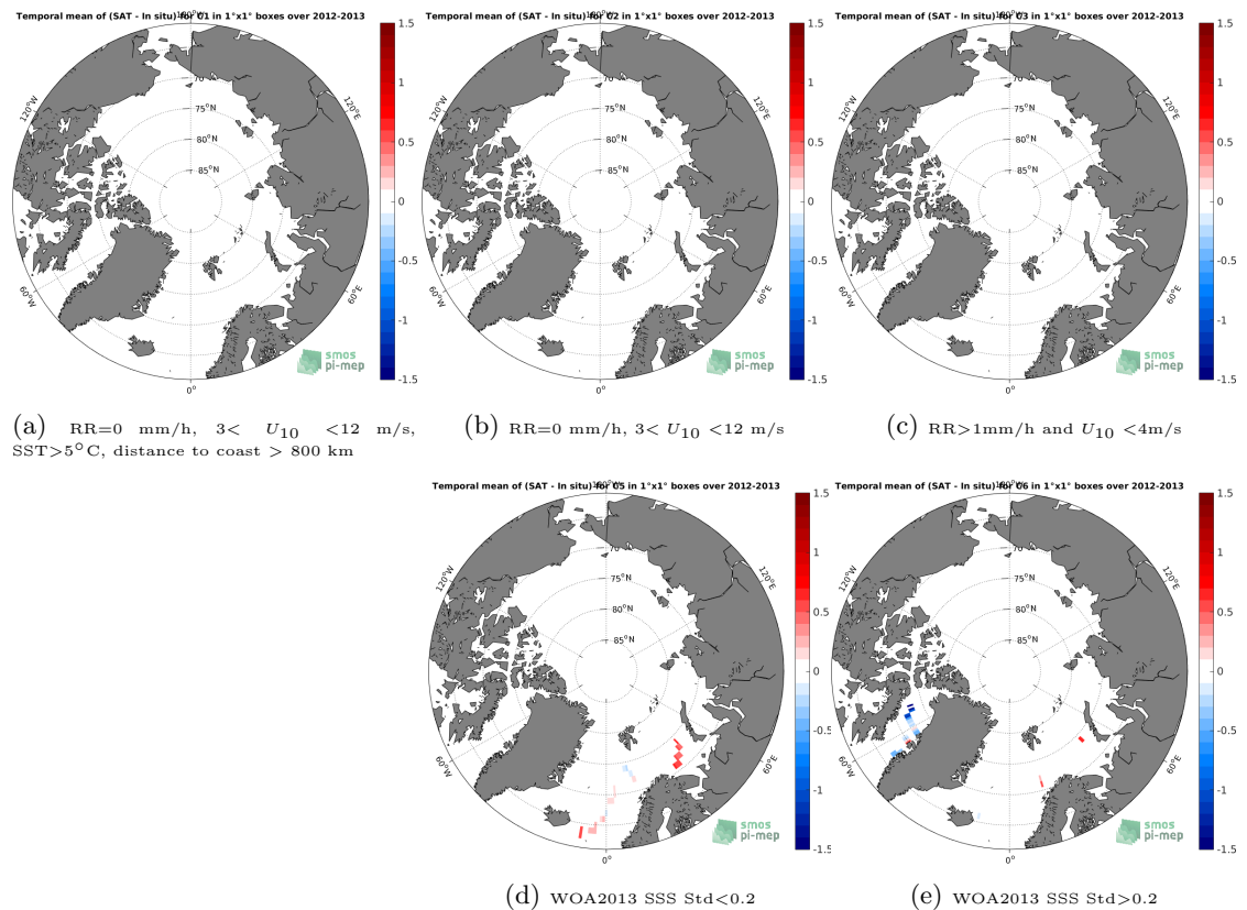
Figure 12: Temporal mean gridded over spatial boxes of size 1^\circ \times 1^\circ of \Delta SSS (Aquarius-L3-JPL-V5-7DAY-RUNNING - TSG-GOSUD-Sailing-ship) for 5 different subdatasets corresponding to:RR=0 mm/h, 3 < U_{10} < 12 m/s, SST >5^\circ C, distance to coast > 800 km (a), RR=0 mm/h, 3 < U_{10} < 12 m/s (b), RR >1 mm/h and U_{10} < 4 m/s (c), WOA2013 SSS Std <0.2 (d), WOA2013 SSS Std >0.2 (e).
