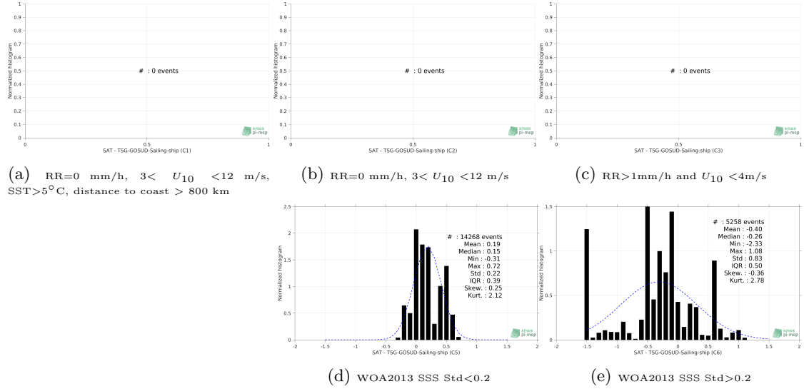
Figure 13: Normalized histogram of \Delta\text{SSS} (Aquarius-L3-JPL-V5-7DAY-RUNNING - TSG-GOSUD-Sailing-ship) for 5 different subdatasets corresponding to: RR=0 mm/h, 3 < U_{10} < 12 m/s, SST > 5^\circ\text{C} , distance to coast > 800 km (a), RR=0 mm/h, 3 < U_{10} < 12 m/s (b), RR > 1\text{mm/h} and U_{10} < 4\text{m/s} (c), WOA2013 SSS Std < 0.2 (d), WOA2013 SSS Std > 0.2 (e).
