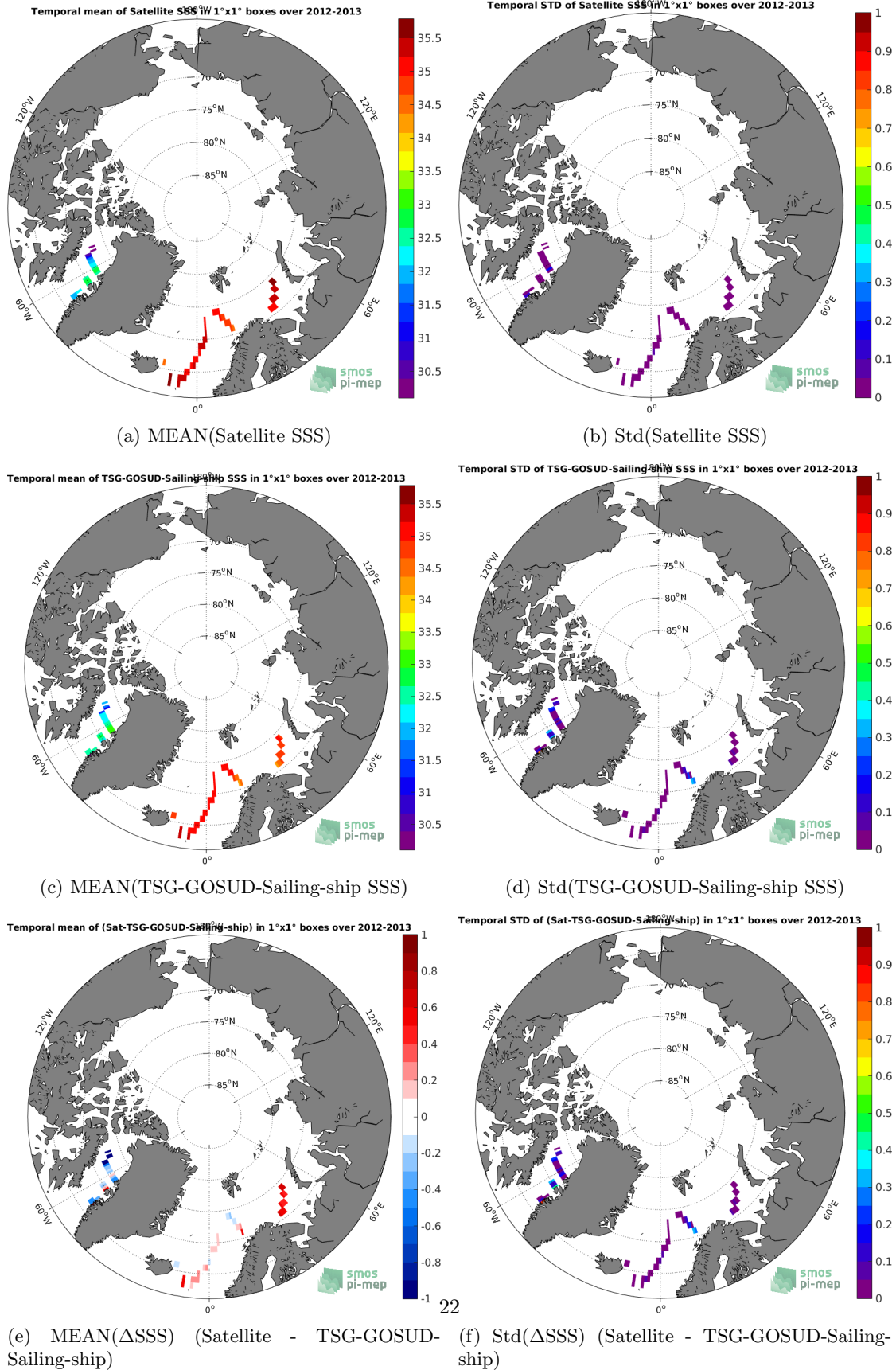
Figure 6: Temporal mean (left) and Std (right) of SSS from Aquarius-L3-JPL-V5-7DAY-RUNNING (top), TSG-GOSUD-Sailing-ship (middle), and of \Delta SSS (Satellite - TSG-GOSUD-Sailing-ship). Only match-up pairs are used to generate these maps.
