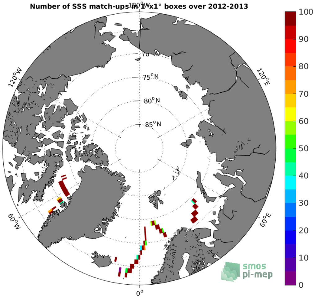
Figure 4: Number of SSS match-ups between TSG-GOSUD-Sailing-ship SSS and the Aquarius-L3-JPL-V5-7DAY-RUNNING SSS product for the Arctic Ocean Pi-MEP region over 1^\circ \times 1^\circ boxes and for the full satellite product period.
