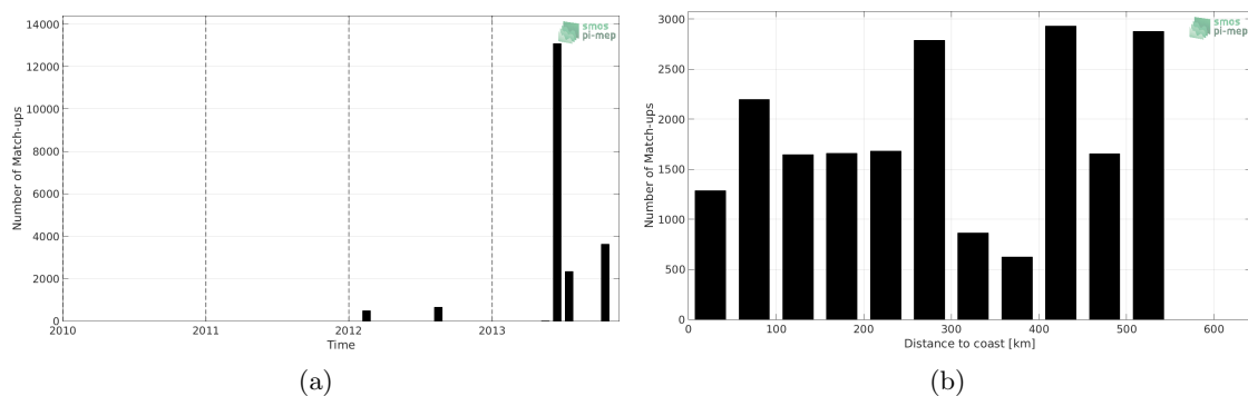
Figure 1: Number of match-ups between TSG-GOSUD-Sailing-ship and Aquarius-L3-JPL-V5-7DAY-RUNNING SSS as a function of time (a) and as function of the distance to coast (b) over the Arctic Ocean Pi-MEP region and for the full satellite product period.
