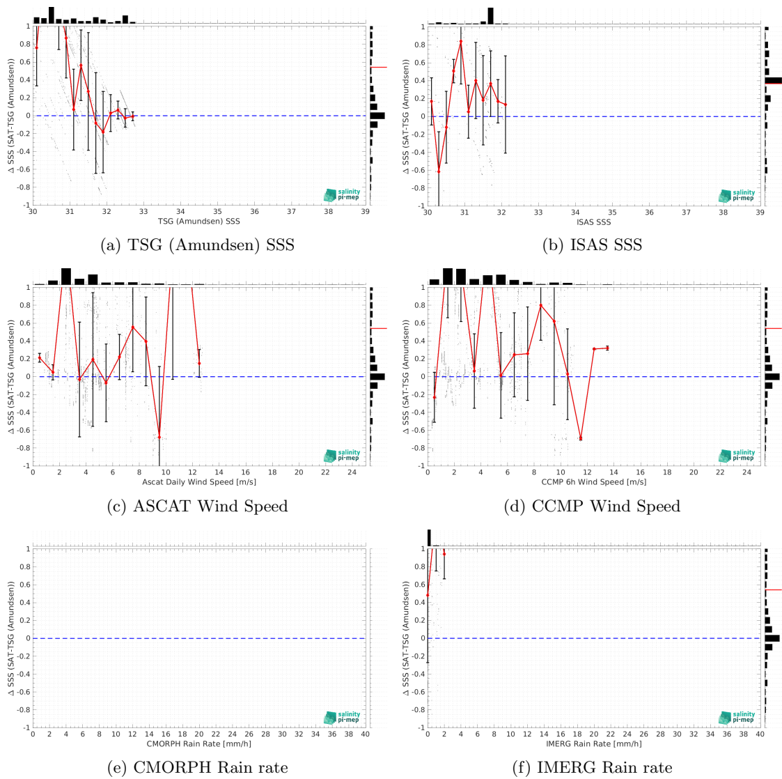
Figure 12: \Delta \text{SSS} (Satellite - TSG (Amundsen)) sorted as function of TSG (Amundsen) SSS values (a), ISAS SSS (b), ASCAT Wind speed (c), CCMP Wind speed (d), CMORPH rain rate (e) and IMERG rain rate (f). In all plots the median and Std of \Delta \text{SSS} for each bin is indicated by the red curves and black vertical thick bars ( \pm 1 Std).
