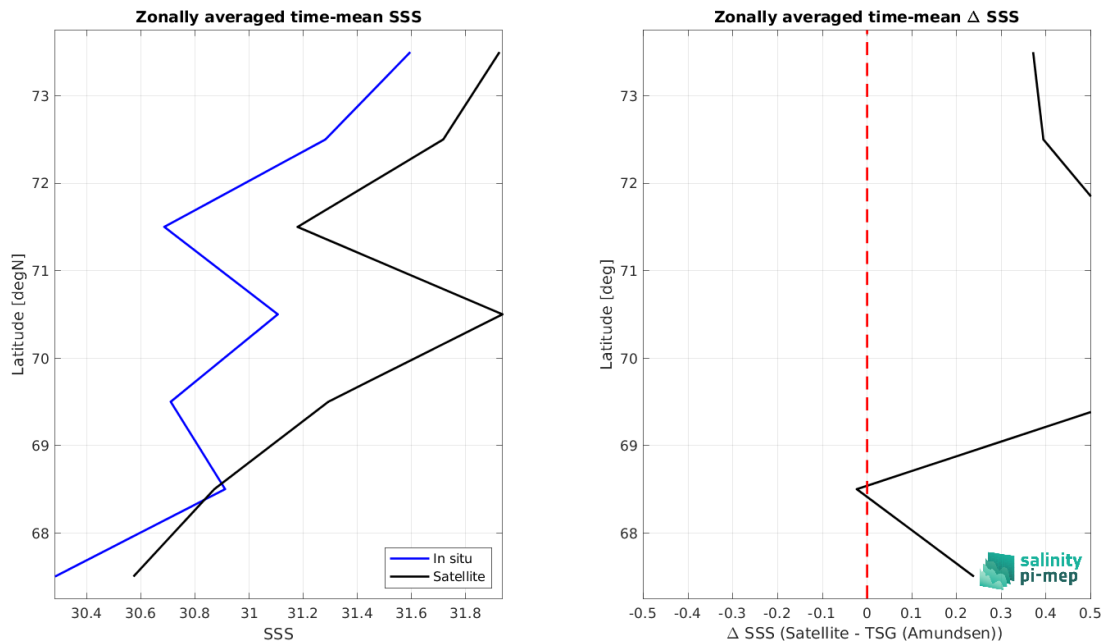
Figure 9: Left panel: Zonal mean SSS from Aquarius SSS L3 CAP v5 - 7-Day running (JPL) satellite product (black) and from TSG (Amundsen) (blue). Right panel: Zonal mean of \Delta SSS (Satellite - TSG (Amundsen)) for all the collected Pi-MEP match-up pairs estimated over the full satellite product period.
