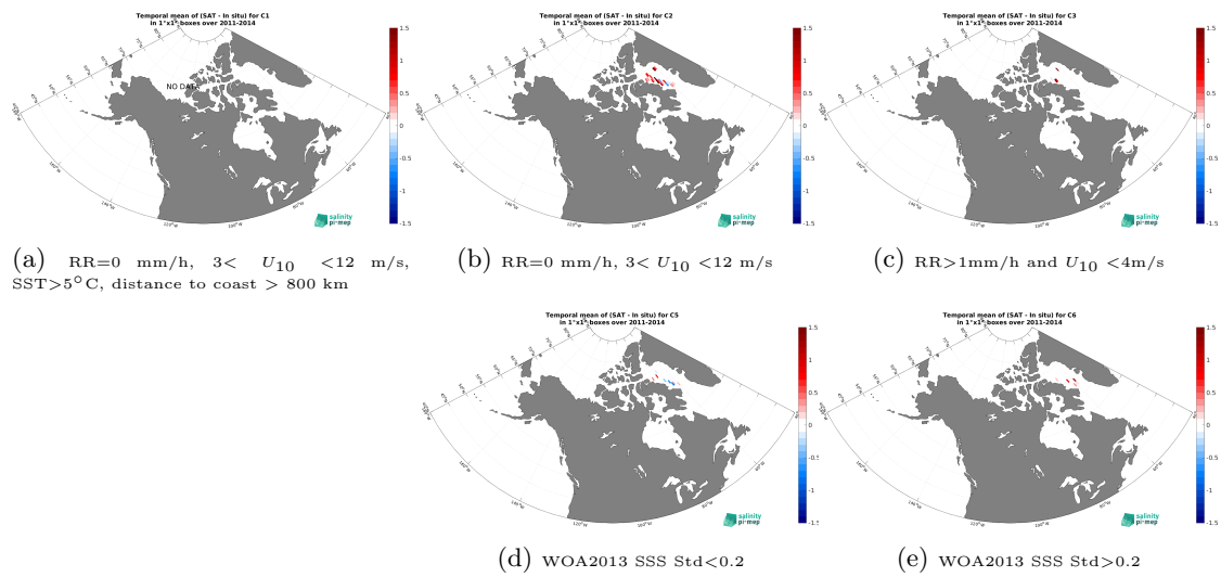
Figure 14: Temporal mean gridded over spatial boxes of size 1^\circ \times 1^\circ of \Delta SSS (Aquarius SSS L3 CAP v5 - 7-Day running (JPL) - TSG (Amundsen)) for 5 different subdatasets corresponding to:RR=0 mm/h, 3 < U_{10} < 12 m/s, SST > 5°C, distance to coast > 800 km (a), RR=0 mm/h, 3 < U_{10} < 12 m/s (b), RR > 1mm/h and U_{10} < 4 m/s (c), WOA2013 SSS Std < 0.2 (d), WOA2013 SSS Std > 0.2 (e).
