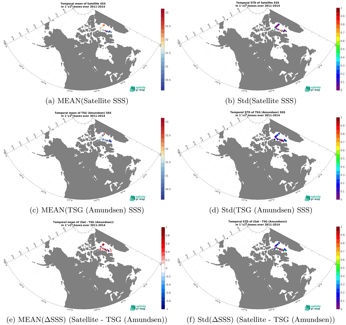
Figure 7: Temporal mean (left) and Std (right) of SSS from Aquarius SSS L3 CAP v5 - 7-Day running (JPL) (top), TSG (Amundsen) (middle), and of \Delta SSS (Satellite - TSG (Amundsen)). Only match-up pairs are used to generate these maps.
