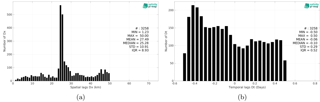
Figure 6: Histograms of the spatial (a) and temporal (b) lags between the location/time of the TSG (Amundsen) measurement and the date of the corresponding Aquarius SSS L3 CAP v5 - 7-Day running (JPL) SSS pixel.
