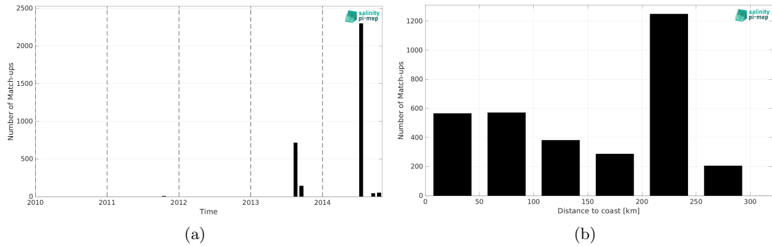
Figure 2: Number of match-ups between TSG (Amundsen) and Aquarius SSS L3 CAP v5 - 7-Day running (JPL) SSS as a function of time (a) and as function of the distance to coast (b) over the Arctic Ocean Pi-MEP region and for the full satellite product period.
