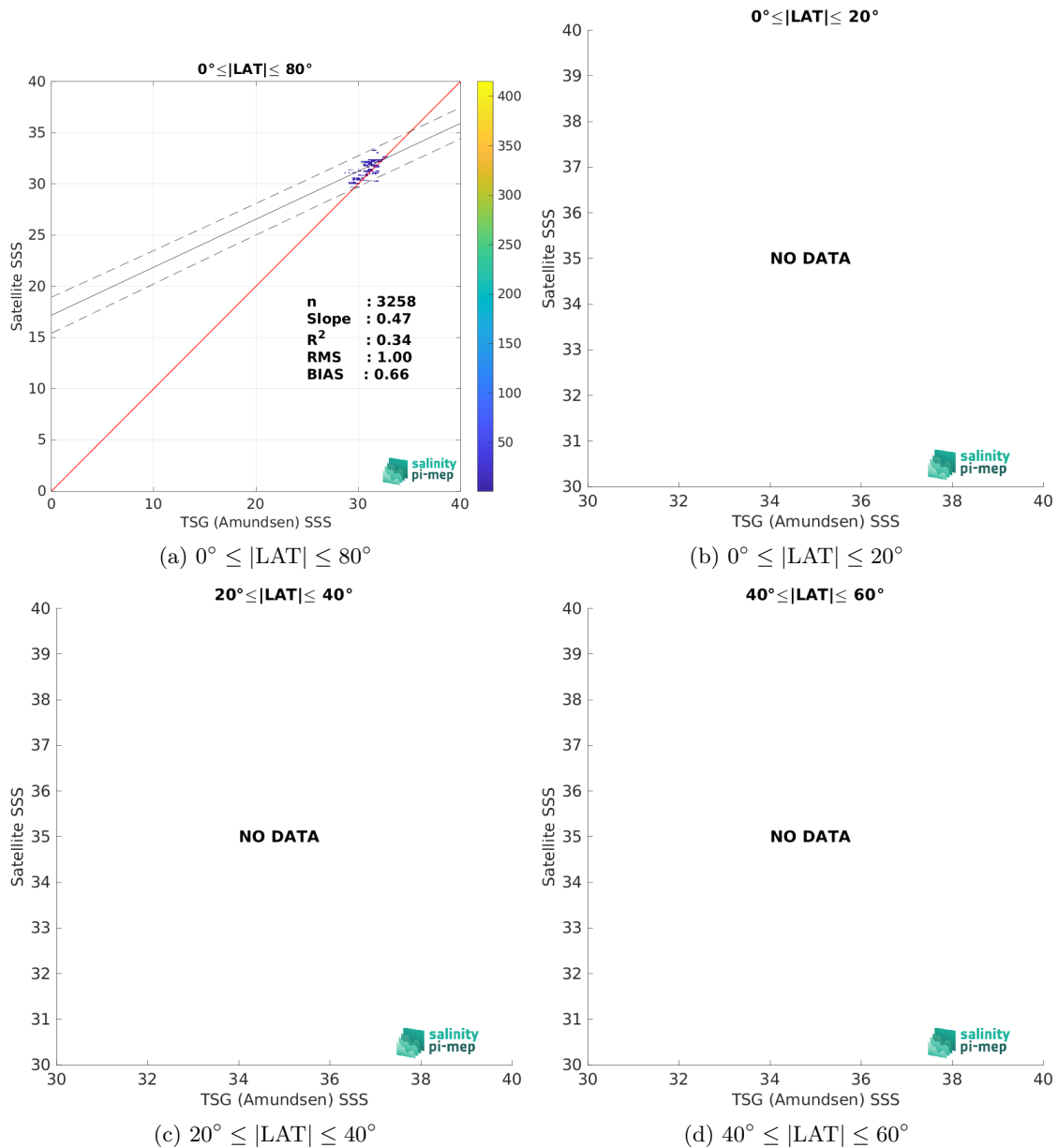
Figure 10: Contour maps of the concentration of Aquarius SSS L3 CAP v5 - 7-Day running (JPL) SSS (y-axis) versus TSG (Amundsen) SSS (x-axis) at match-up pairs for different latitude bands. For each plot, the red line shows x=y . The black thin and dashed lines indicate a linear fit through the data cloud and the \pm 95\% confidence levels, respectively. The number match-up pairs n , the slope and R^2 coefficient of the linear fit, the root mean square (RMS) and the mean bias between satellite and in situ data are indicated for each latitude band in each plots.
