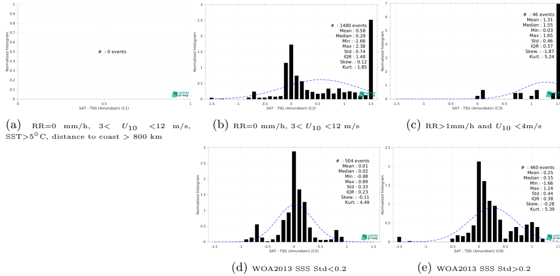
Figure 15: Normalized histogram of \Delta SSS (Aquarius SSS L3 CAP v5 - 7-Day running (JPL) - TSG (Amundsen)) for 5 different subdatasets corresponding to: RR=0 mm/h, 3 < U_{10} < 12 m/s, SST>5°C, distance to coast > 800 km (a), RR=0 mm/h, 3 < U_{10} < 12 m/s (b), RR>1mm/h and U_{10} < 4 m/s (c), WOA2013 SSS Std<0.2 (d), WOA2013 SSS Std>0.2 (e).
