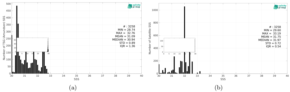
Figure 3: Histograms of SSS from TSG (Amundsen) (a) and Aquarius SSS L3 CAP v5 - 7-Day running (JPL) (b) considering all match-up pairs per bins of 0.1 over the Arctic Ocean Pi-MEP region and for the full satellite product period.
