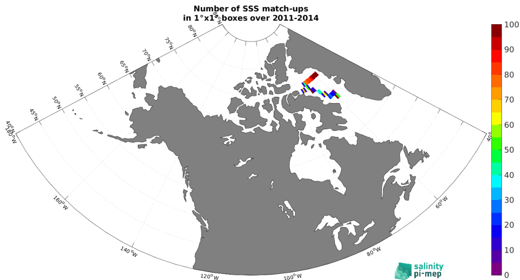
Figure 5: Number of SSS match-ups between TSG (Amundsen) SSS and the Aquarius SSS L3 CAP v5 - 7-Day running (JPL) SSS product for the Arctic Ocean Pi-MEP region over 1^\circ \times 1^\circ boxes and for the full satellite product period.
