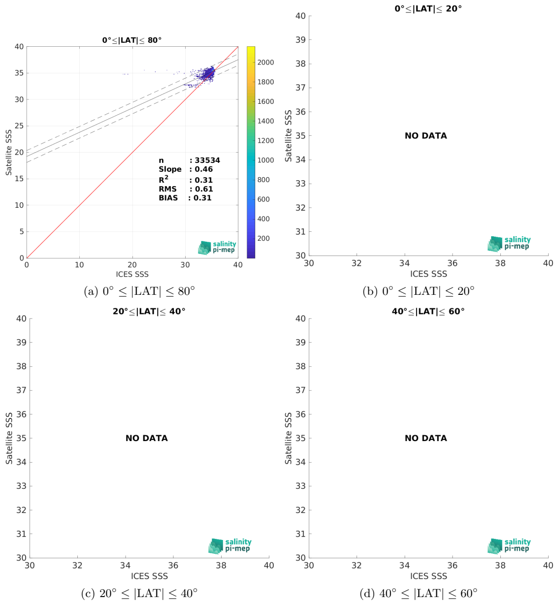
Figure 10: Contour maps of the concentration of Aquarius SSS L3 CAP v5 - 7-Day running (JPL) SSS (y-axis) versus ICES SSS (x-axis) at match-up pairs for different latitude bands. For each plot, the red line shows x=y . The black thin and dashed lines indicate a linear fit through the data cloud and the \pm 95\% confidence levels, respectively. The number match-up pairs n , the slope and R^2 coefficient of the linear fit, the root mean square (RMS) and the mean bias between satellite and in situ data are indicated for each latitude band in each plots.
