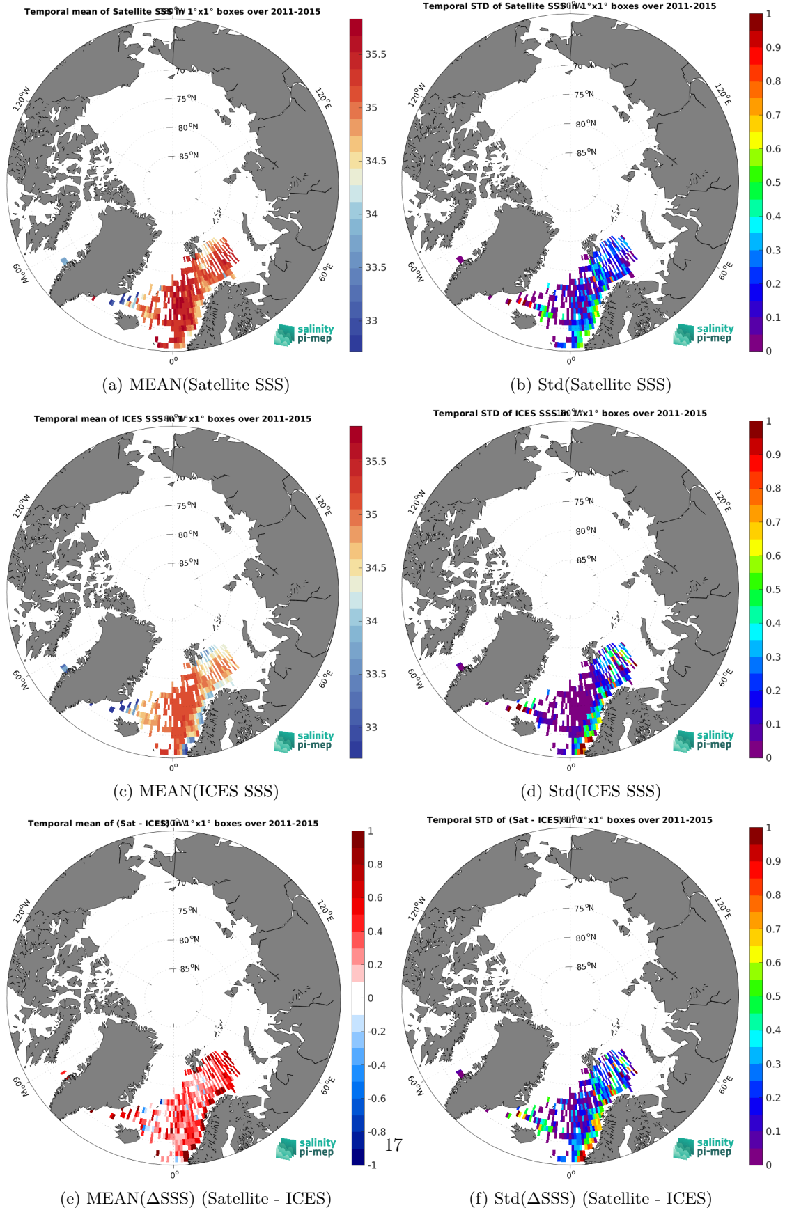
Figure 7: Temporal mean (left) and Std (right) of SSS from Aquarius SSS L3 CAP v5 - 7-Day running (JPL) (top), ICES (middle), and of \Delta SSS (Satellite - ICES). Only match-up pairs are used to generate these maps.
