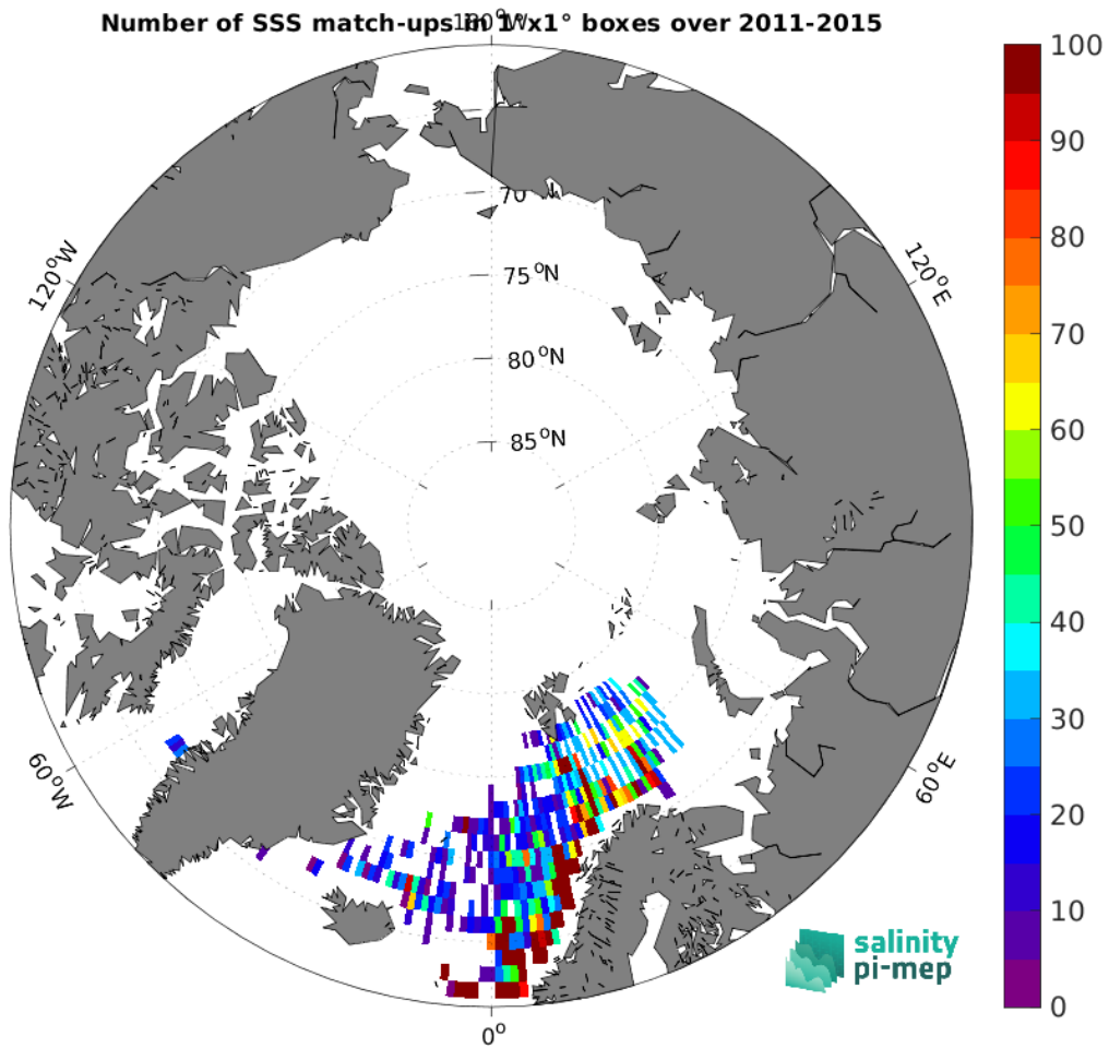
Figure 5: Number of SSS match-ups between ICES SSS and the Aquarius SSS L3 CAP v5 - 7-Day running (JPL) SSS product for the Arctic Ocean Pi-MEP region over 1^\circ \times 1^\circ boxes and for the full satellite product period.
