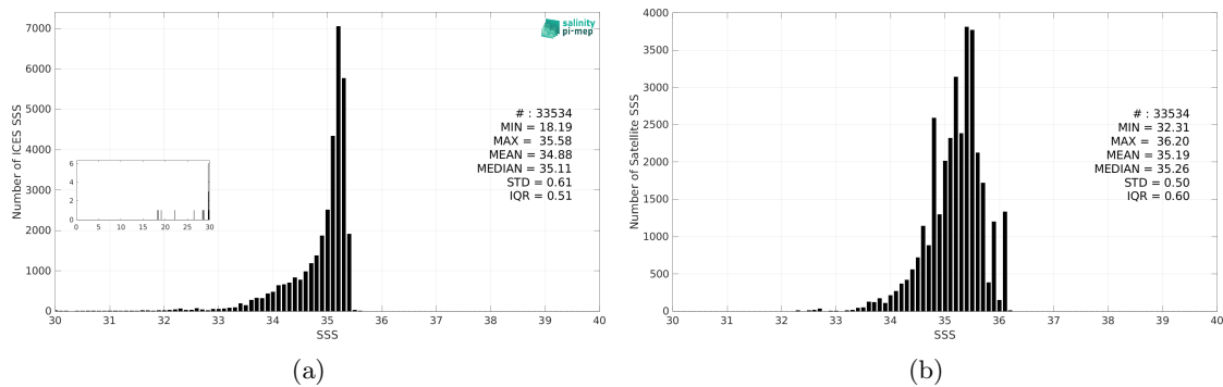
Figure 3: Histograms of SSS from ICES (a) and Aquarius SSS L3 CAP v5 - 7-Day running (JPL) (b) considering all match-up pairs per bins of 0.1 over the Arctic Ocean Pi-MEP region and for the full satellite product period.
