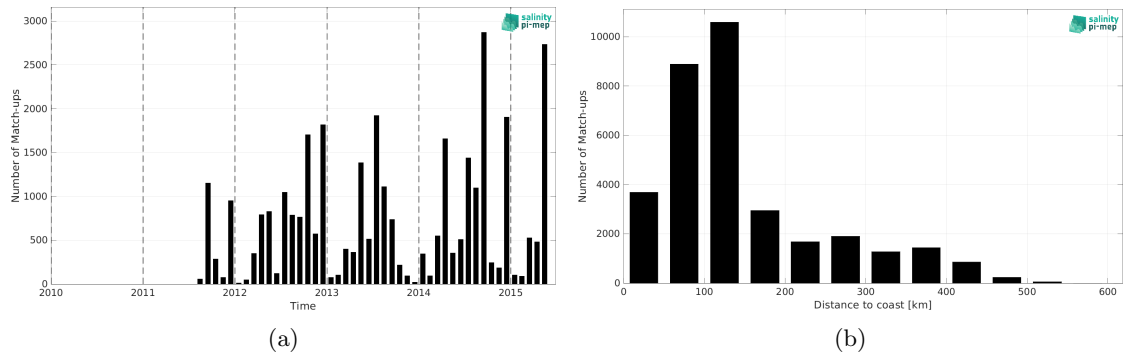
Figure 2: Number of match-ups between ICES and Aquarius SSS L3 CAP v5 - 7-Day running (JPL) SSS as a function of time (a) and as function of the distance to coast (b) over the Arctic Ocean Pi-MEP region and for the full satellite product period.
