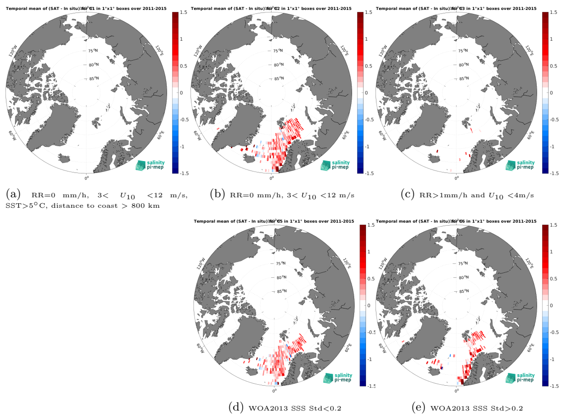
Figure 14: Temporal mean gridded over spatial boxes of size 1^\circ \times 1^\circ of \Delta SSS (Aquarius SSS L3 CAP v5 - 7-Day running (JPL) - ICES) for 5 different subdatasets corresponding to: RR=0 mm/h, 3 < U_{10} < 12 m/s, SST > 5°C, distance to coast > 800 km (a), RR=0 mm/h, 3 < U_{10} < 12 m/s (b), RR > 1mm/h and U_{10} < 4 m/s (c), WOA2013 SSS Std < 0.2 (d), WOA2013 SSS Std > 0.2 (e).
