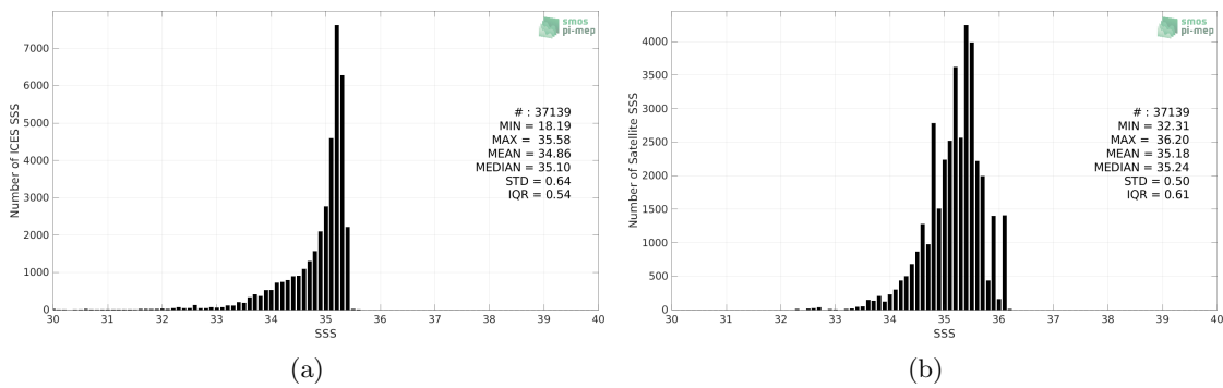
Figure 2: Histograms of SSS from ICES (a) and Aquarius SSS L3 CAP v5 - 7-Day running (JPL) (b) considering all match-up pairs per bins of 0.1 over the Arctic Ocean Pi-MEP region and for the full satellite product period.
