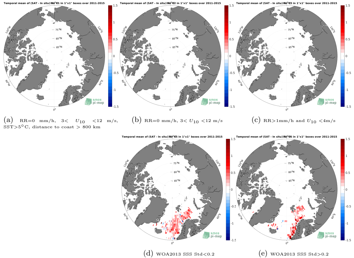
Figure 12: Temporal mean gridded over spatial boxes of size 1^{\circ}\times 1^{\circ} of \Delta\text{SSS} (Aquarius SSS L3 CAP v5 - 7-Day running (JPL) - ICES) for 5 different subdatasets corresponding to:RR=0 mm/h, 3 < U_{10} < 12 m/s, SST >5^{\circ}\text{C} , distance to coast > 800 km (a), RR=0 mm/h, 3 < U_{10} < 12 m/s (b), RR >1 mm/h and U_{10} < 4 m/s (c), WOA2013 SSS Std <0.2 (d), WOA2013 SSS Std >0.2 (e).
