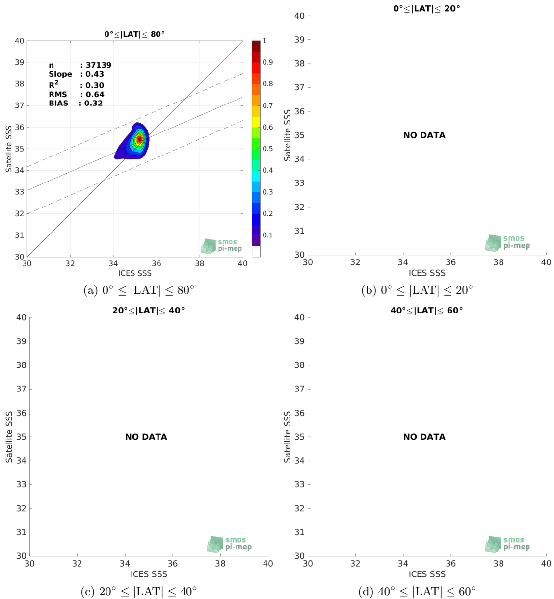
Figure 9: Contour maps of the concentration of Aquarius SSS L3 CAP v5 - 7-Day running (JPL) SSS (y-axis) versus ICES SSS (x-axis) at match-up pairs for different latitude bands. For each plot, the red line shows x=y . The black thin and dashed lines indicate a linear fit through the data cloud and the \pm 95\% confidence levels, respectively. The number match-up pairs n , the slope and R^2 coefficient of the linear fit, the root mean square (RMS) and the mean bias between satellite and in situ data are indicated for each latitude band in each plots.
