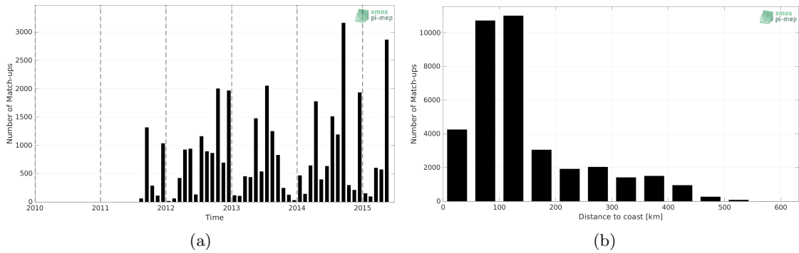
Figure 1: Number of match-ups between ICES and Aquarius SSS L3 CAP v5 - 7-Day running (JPL) SSS as a function of time (a) and as function of the distance to coast (b) over the Arctic Ocean Pi-MEP region and for the full satellite product period.
