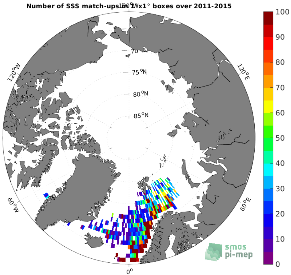
Figure 4: Number of SSS match-ups between ICES SSS and the Aquarius SSS L3 CAP v5 - 7-Day running (JPL) SSS product for the Arctic Ocean Pi-MEP region over 1^\circ \times 1^\circ boxes and for the full satellite product period.
