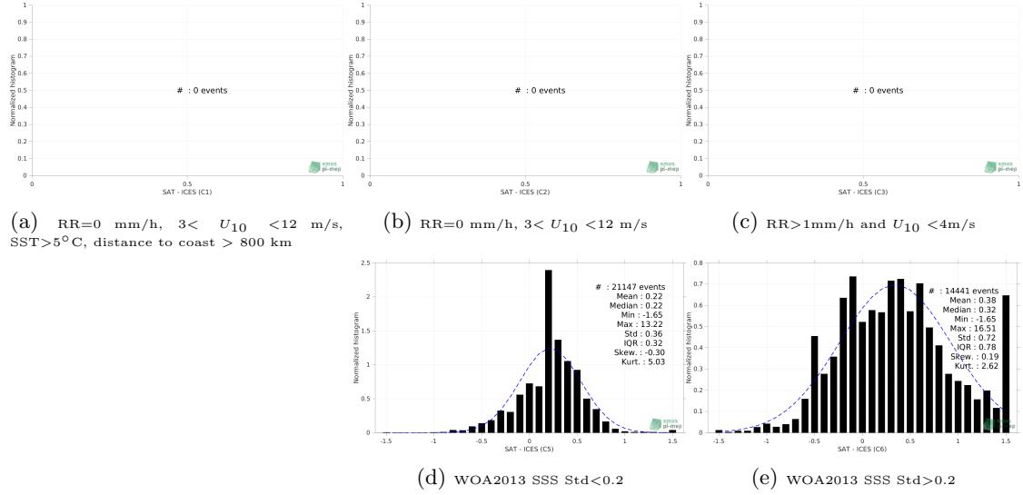
Figure 13: Normalized histogram of \Delta SSS (Aquarius SSS L3 CAP v5 - 7-Day running (JPL) - ICES) for 5 different subdatasets corresponding to: RR=0 mm/h, 3 < U_{10} < 12 m/s, SST>5°C, distance to coast > 800 km (a), RR=0 mm/h, 3 < U_{10} < 12 m/s (b), RR>1mm/h and U_{10} < 4 m/s (c), WOA2013 SSS Std<0.2 (d), WOA2013 SSS Std>0.2 (e).
