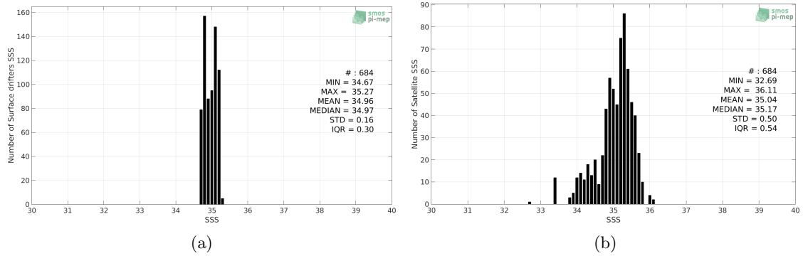
Figure 2: Histograms of SSS from Surface drifters (a) and Aquarius-L3-JPL-V5-7DAY-RUNNING (b) considering all match-up pairs per bins of 0.1 over the Arctic Ocean Pi-MEP region and for the full satellite product period.
