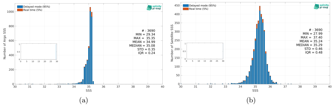
Figure 3: Histograms of SSS from Argo (a) and Aquarius SSS L3 CAP v5 - 7-Day running (JPL) (b) considering all match-up pairs per bins of 0.1 over the Arctic Ocean Pi-MEP region and for the full satellite product period.
