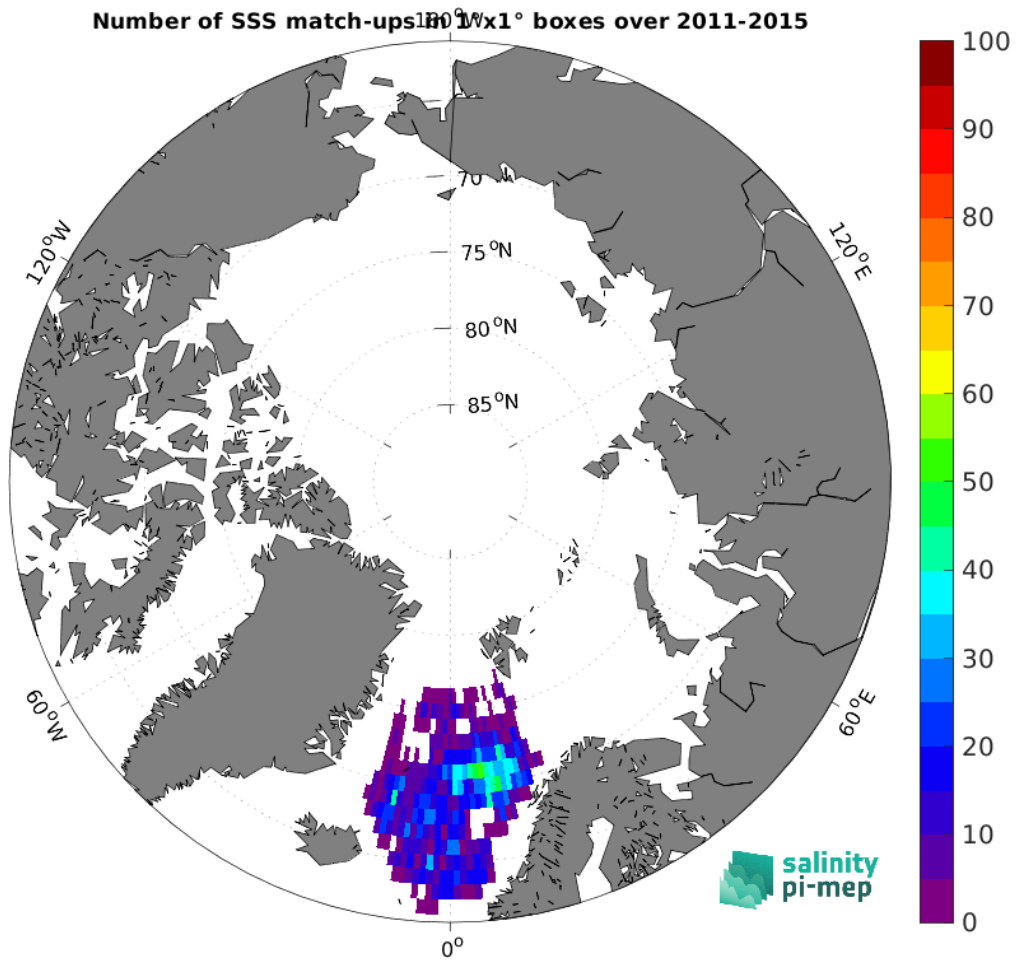
Figure 5: Number of SSS match-ups between Argo SSS and the Aquarius SSS L3 CAP v5 - 7-Day running (JPL) SSS product for the Arctic Ocean Pi-MEP region over 1^\circ \times 1^\circ boxes and for the full satellite product period.
