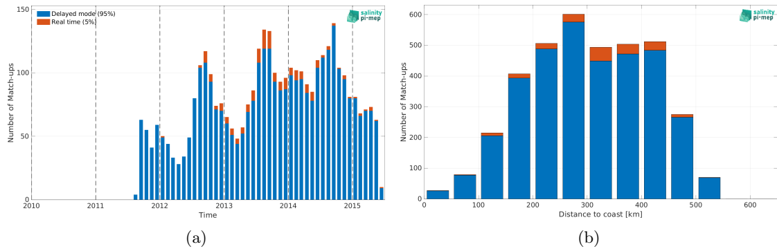
Figure 2: Number of match-ups between Argo and Aquarius SSS L3 CAP v5 - 7-Day running (JPL) SSS as a function of time (a) and as function of the distance to coast (b) over the Arctic Ocean Pi-MEP region and for the full satellite product period.
