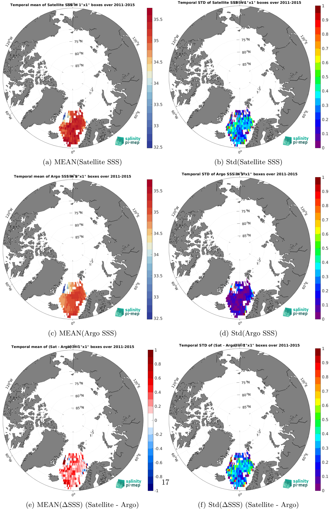
Figure 7: Temporal mean (left) and Std (right) of SSS from Aquarius SSS L3 CAP v5 - 7-Day running (JPL) (top), Argo (middle), and of \Delta SSS (Satellite - Argo). Only match-up pairs are used to generate these maps.
