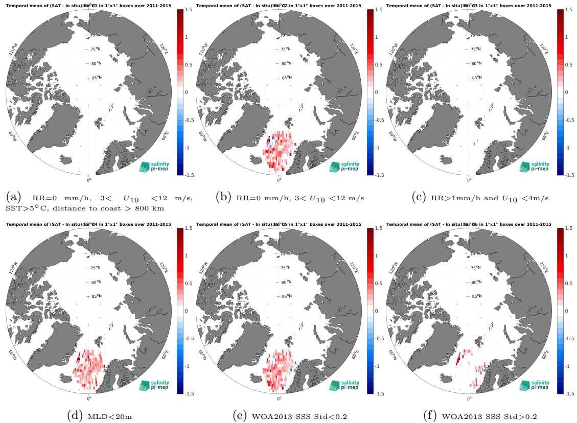
Figure 14: Temporal mean gridded over spatial boxes of size 1^\circ \times 1^\circ of \Delta SSS (Aquarius SSS L3 CAP v5 - 7-Day running (JPL) - Argo) for 6 different subdatasets corresponding to:RR=0 mm/h, 3 < U_{10} < 12 m/s, SST>5°C, distance to coast > 800 km (a), RR=0 mm/h, 3 < U_{10} < 12 m/s (b), RR>1mm/h and U_{10} < 4 m/s (c),MLD<20m (d),WOA2013 SSS Std<0.2 (e),WOA2013 SSS Std>0.2 (f).
