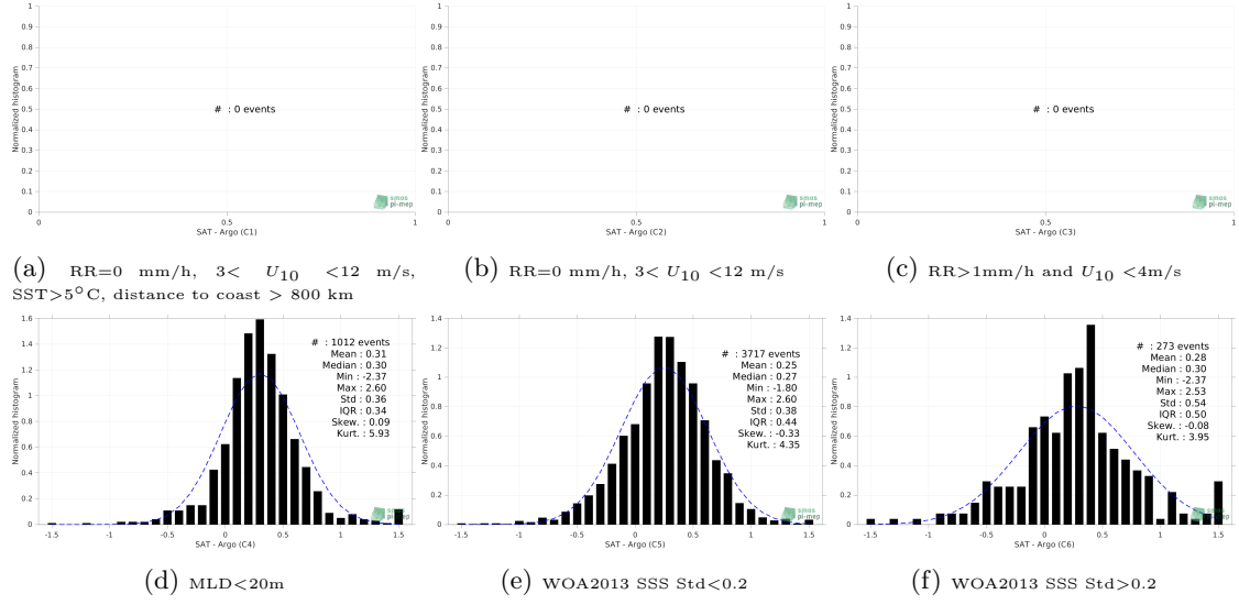
Figure 13: Normalized histogram of \Delta\text{SSS} (Aquarius SSS L3 CAP v5 - 7-Day running (JPL) - Argo) for 6 different subdatasets corresponding to: RR=0 mm/h, 3 < U_{10} < 12 m/s, SST > 5^{\circ}\text{C} , distance to coast > 800 km (a), RR=0 mm/h, 3 < U_{10} < 12 m/s (b), RR > 1\text{mm/h} and U_{10} < 4\text{m/s} (c), MLD < 20\text{m} (d), WOA2013 SSS Std < 0.2 (e), WOA2013 SSS Std > 0.2 (f).
