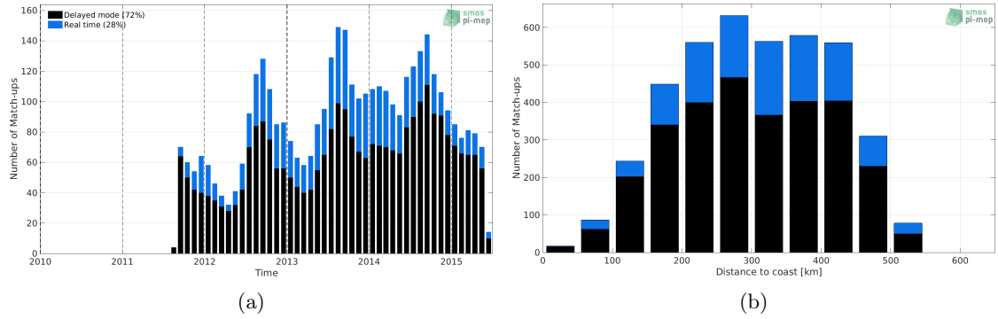
Figure 1: Number of match-ups between Argo and Aquarius SSS L3 CAP v5 - 7-Day running (JPL) SSS as a function of time (a) and as function of the distance to coast (b) over the Arctic Ocean Pi-MEP region and for the full satellite product period.
