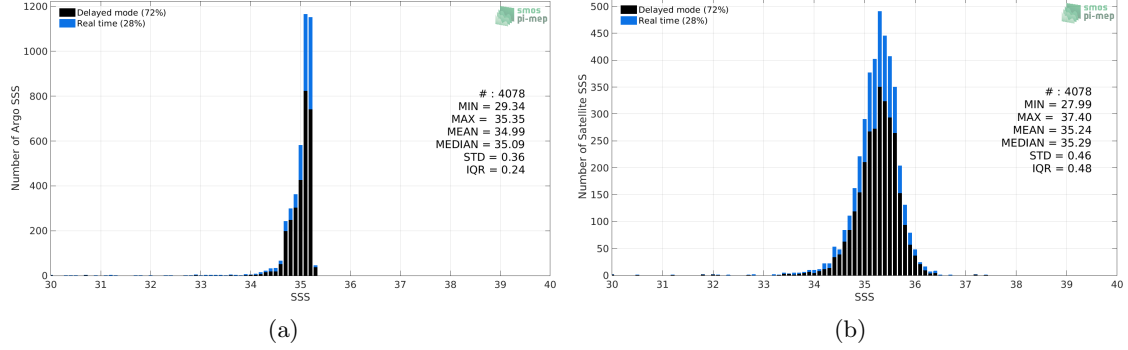
Figure 2: Histograms of SSS from Argo (a) and Aquarius SSS L3 CAP v5 - 7-Day running (JPL) (b) considering all match-up pairs per bins of 0.1 over the Arctic Ocean Pi-MEP region and for the full satellite product period.
