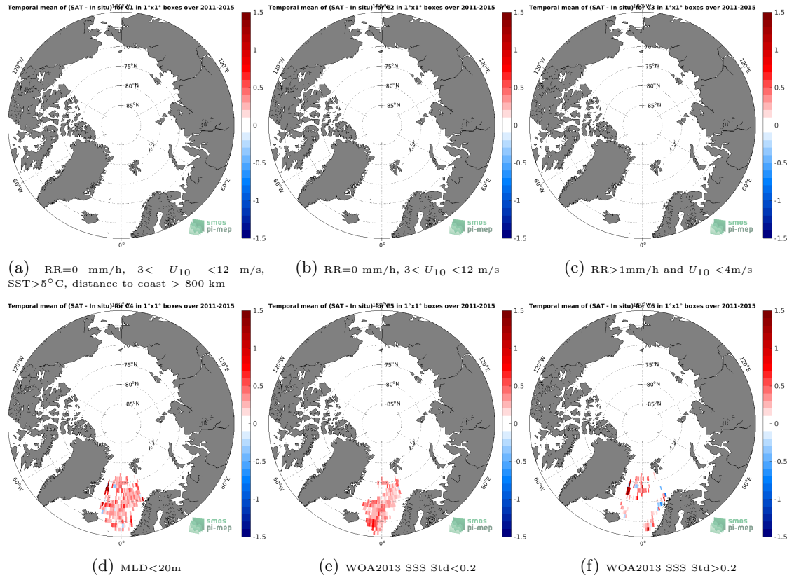
Figure 12: Temporal mean gridded over spatial boxes of size 1^{\circ}\times 1^{\circ} of \Delta\text{SSS} (Aquarius SSS L3 CAP v5 - 7-Day running (JPL) - Argo) for 6 different subdatasets corresponding to: RR=0 mm/h, 3 < U_{10} < 12 m/s, SST > 5^{\circ}\text{C} , distance to coast > 800 km (a), RR=0 mm/h, 3 < U_{10} < 12 m/s (b), RR > 1 mm/h and U_{10} < 4 m/s (c), MLD < 20\text{m} (d), WOA2013 SSS Std < 0.2 (e), WOA2013 SSS Std > 0.2 (f).
