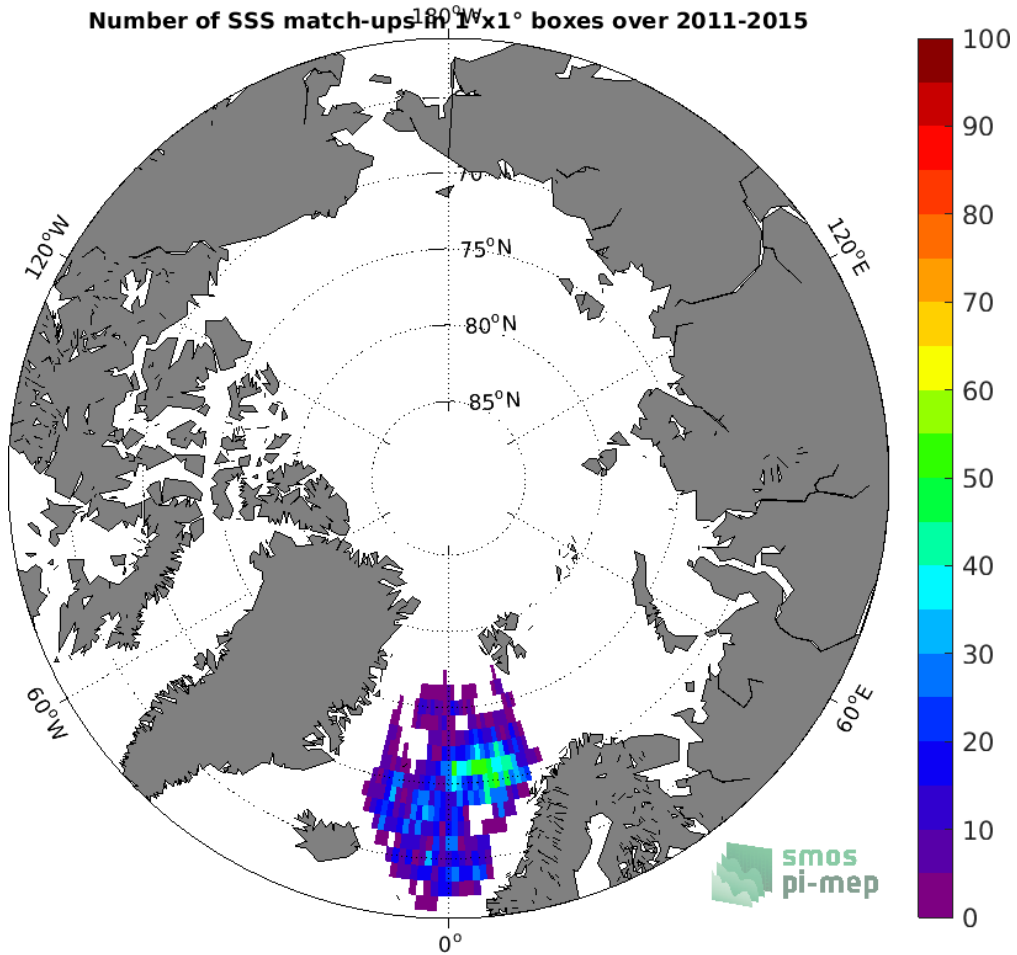
Figure 4: Number of SSS match-ups between Argo SSS and the Aquarius SSS L3 CAP v5 - 7-Day running (JPL) SSS product for the Arctic Ocean Pi-MEP region over 1^\circ \times 1^\circ boxes and for the full satellite product period.
