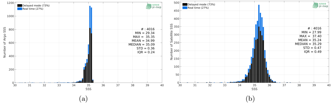
Figure 2: Histograms of SSS from Argo (a) and Aquarius-L3-JPL-V5-7DAY-RUNNING (b) considering all match-up pairs per bins of 0.1 over the Arctic Ocean Pi-MEP region and for the full satellite product period.
