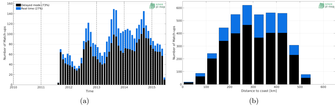
Figure 1: Number of match-ups between Argo and Aquarius-L3-JPL-V5-7DAY-RUNNING SSS as a function of time (a) and as function of the distance to coast (b) over the Arctic Ocean Pi-MEP region and for the full satellite product period.
