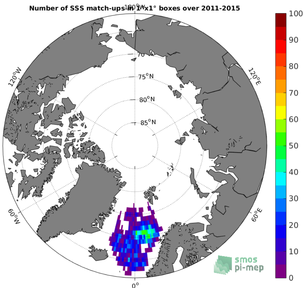
Figure 4: Number of SSS match-ups between Argo SSS and the Aquarius-L3-JPL-V5-7DAY-RUNNING SSS product for the Arctic Ocean Pi-MEP region over 1^\circ \times 1^\circ boxes and for the full satellite product period.
