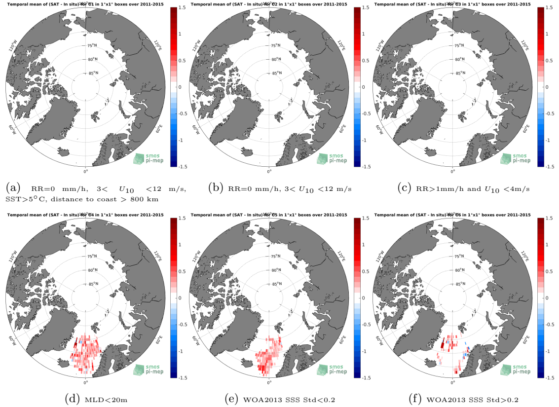
Figure 12: Temporal mean gridded over spatial boxes of size 1^{\circ}\times 1^{\circ} of \Delta\text{SSS} (Aquarius-L3-JPL-V5-7DAY-RUNNING - Argo) for 6 different subdatasets corresponding to: RR=0 mm/h, 3 < U_{10} < 12 m/s, SST >5^{\circ}\text{C} , distance to coast > 800 km (a), RR=0 mm/h, 3 < U_{10} < 12 m/s (b), RR >1\text{mm/h} and U_{10} < 4\text{m/s} (c), MLD <20\text{m} (d), WOA2013 SSS Std <0.2 (e), WOA2013 SSS Std >0.2 (f).
