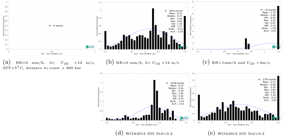
Figure 15: Normalized histogram of \Delta\text{SSS} (Aquarius SSS L3 CAP v5 - Monthly (JPL) - TSG (SAMOS)) for 5 different subdatasets corresponding to: RR=0 mm/h, 3 < U_{10} < 12 m/s, SST > 5^{\circ}\text{C} , distance to coast > 800 km (a), RR=0 mm/h, 3 < U_{10} < 12 m/s (b), RR > 1\text{mm/h} and U_{10} < 4\text{m/s} (c), WOA2013 SSS Std < 0.2 (d), WOA2013 SSS Std > 0.2 (e).
