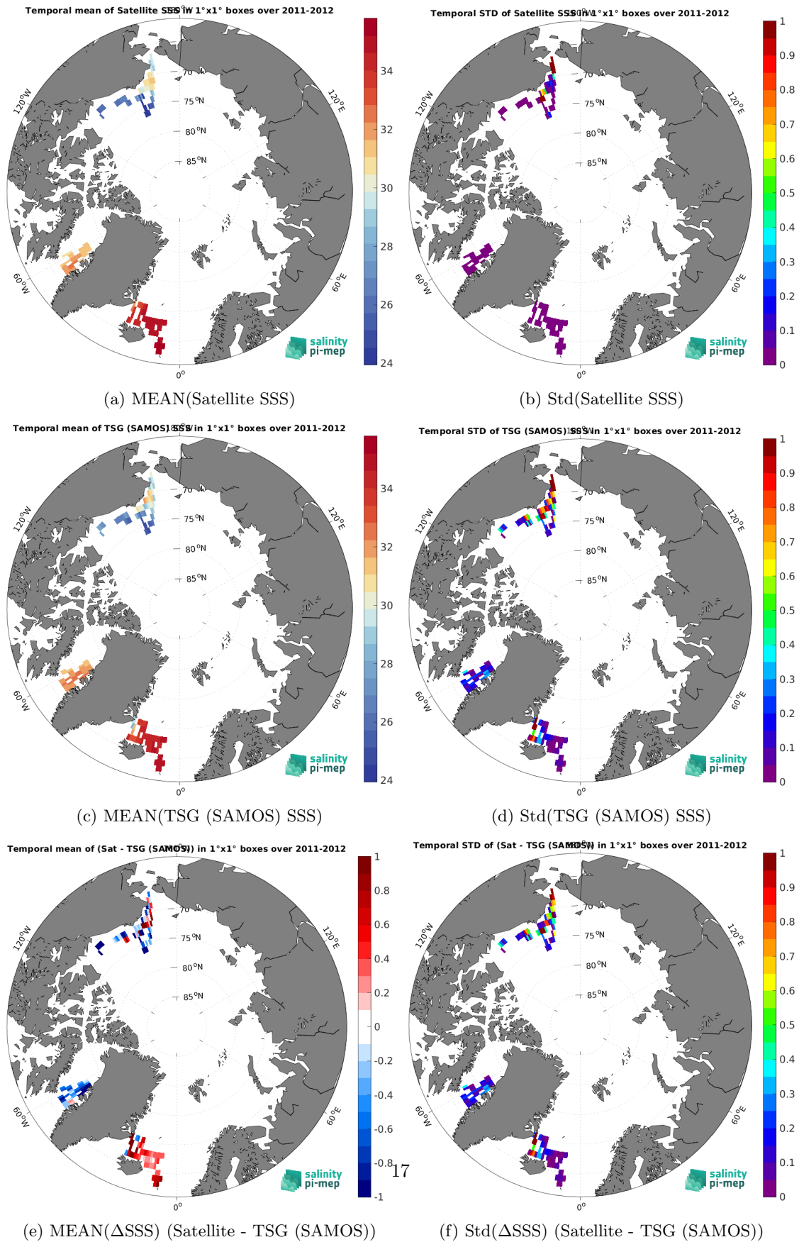
Figure 7: Temporal mean (left) and Std (right) of SSS from Aquarius SSS L3 CAP v5 - Monthly (JPL) (top), TSG (SAMOS) (middle), and of \Delta SSS (Satellite - TSG (SAMOS)). Only match-up pairs are used to generate these maps.
