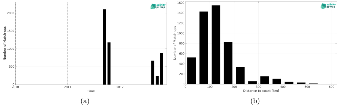
Figure 2: Number of match-ups between TSG (SAMOS) and Aquarius SSS L3 CAP v5 - Monthly (JPL) SSS as a function of time (a) and as function of the distance to coast (b) over the Arctic Ocean Pi-MEP region and for the full satellite product period.
