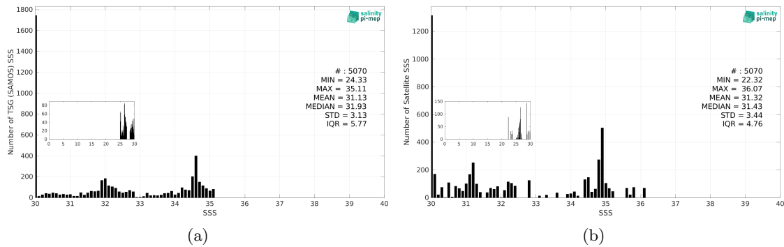
Figure 3: Histograms of SSS from TSG (SAMOS) (a) and Aquarius SSS L3 CAP v5 - Monthly (JPL) (b) considering all match-up pairs per bins of 0.1 over the Arctic Ocean Pi-MEP region and for the full satellite product period.
