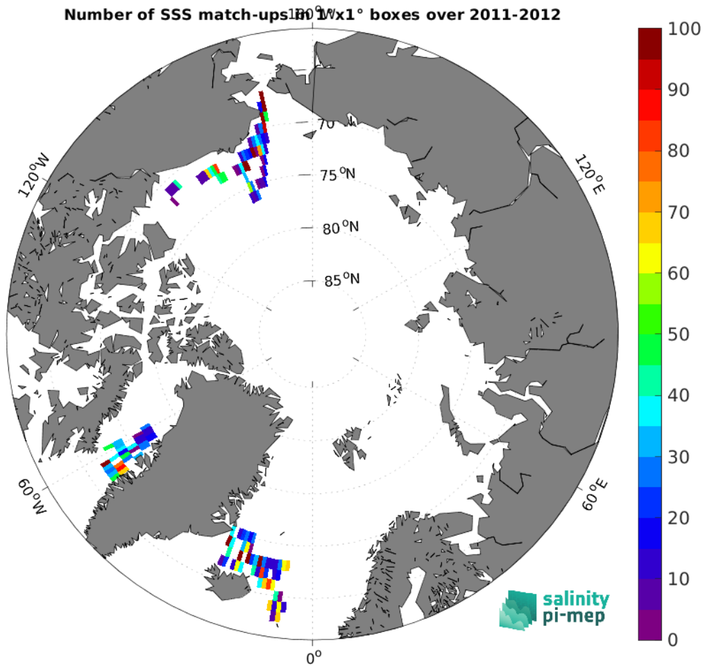
Figure 5: Number of SSS match-ups between TSG (SAMOS) SSS and the Aquarius SSS L3 CAP v5 - Monthly (JPL) SSS product for the Arctic Ocean Pi-MEP region over 1^\circ \times 1^\circ boxes and for the full satellite product period.
