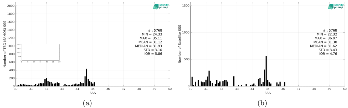
Figure 2: Histograms of SSS from TSG (SAMOS) (a) and Aquarius SSS L3 CAP v5 - Monthly (JPL) (b) considering all match-up pairs per bins of 0.1 over the Arctic Ocean Pi-MEP region and for the full satellite product period.
