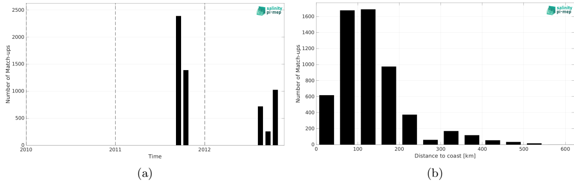
Figure 1: Number of match-ups between TSG (SAMOS) and Aquarius SSS L3 CAP v5 - Monthly (JPL) SSS as a function of time (a) and as function of the distance to coast (b) over the Arctic Ocean Pi-MEP region and for the full satellite product period.
