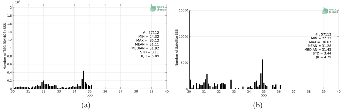
Figure 2: Histograms of SSS from TSG (SAMOS) (a) and Aquarius SSS L3 CAP v5 - Monthly (JPL) (b) considering all match-up pairs per bins of 0.1 over the Arctic Ocean Pi-MEP region and for the full satellite product period.
