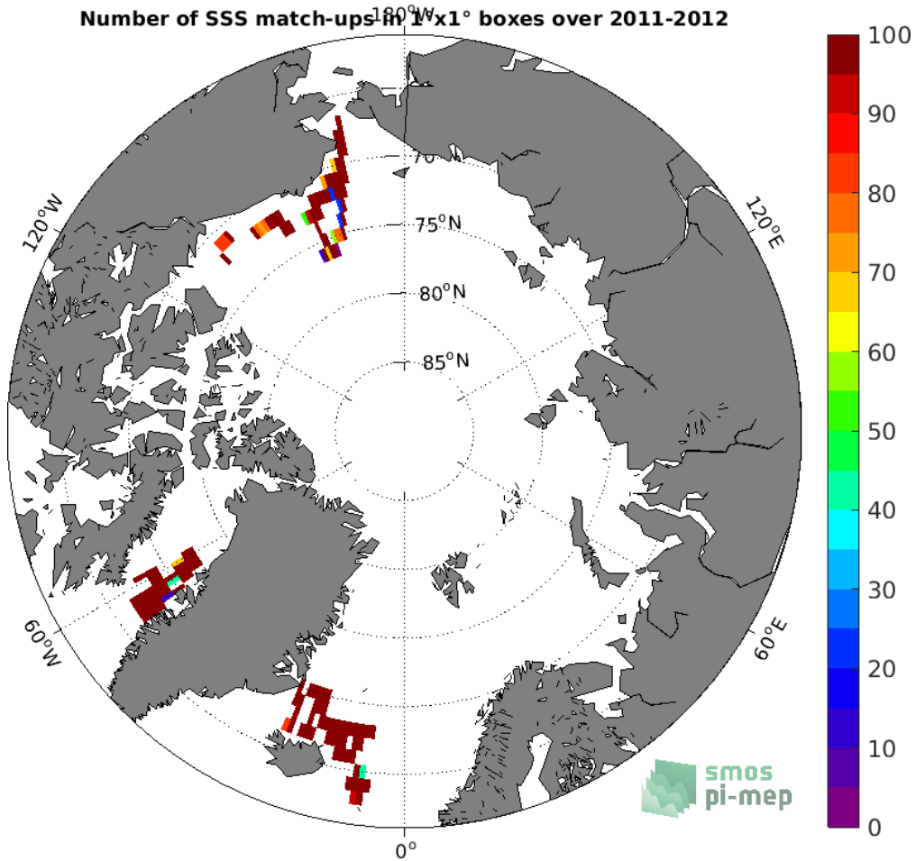
Figure 4: Number of SSS match-ups between TSG (SAMOS) SSS and the Aquarius SSS L3 CAP v5 - Monthly (JPL) SSS product for the Arctic Ocean Pi-MEP region over 1^\circ \times 1^\circ boxes and for the full satellite product period.
