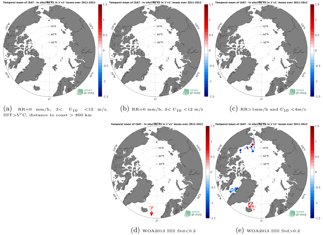
Figure 12: Temporal mean gridded over spatial boxes of size 1^{\circ}\times 1^{\circ} of \Delta\text{SSS} (Aquarius SSS L3 CAP v5 - Monthly (JPL) - TSG (SAMOS)) for 5 different subdatasets corresponding to:RR=0 mm/h, 3 < U_{10} < 12 m/s, SST >5^{\circ}\text{C} , distance to coast > 800 km (a), RR=0 mm/h, 3 < U_{10} < 12 m/s (b), RR >1 mm/h and U_{10} < 4 m/s (c), WOA2013 SSS Std <0.2 (d), WOA2013 SSS Std >0.2 (e).
