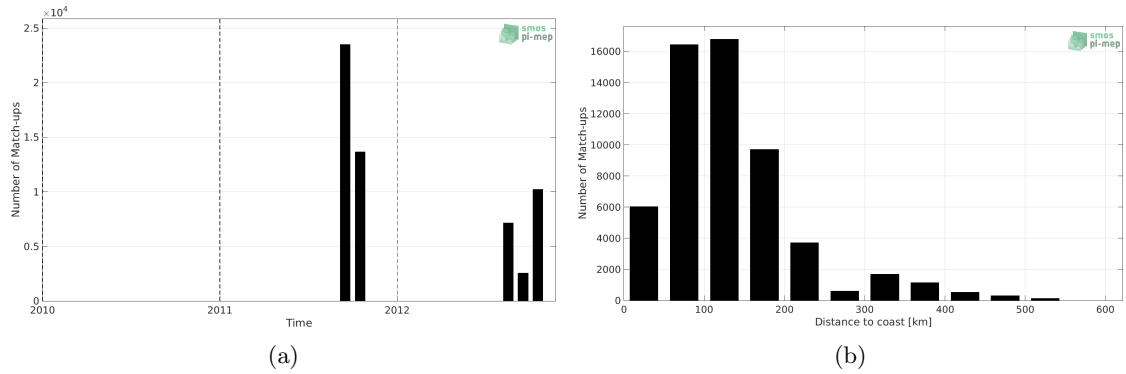
Figure 1: Number of match-ups between TSG (SAMOS) and Aquarius SSS L3 CAP v5 - Monthly (JPL) SSS as a function of time (a) and as function of the distance to coast (b) over the Arctic Ocean Pi-MEP region and for the full satellite product period.
