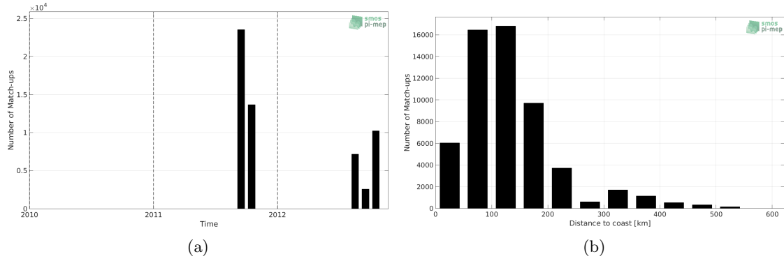
Figure 1: Number of match-ups between TSG-SAMOS and Aquarius-L3-JPL-V5-MONTHLY SSS as a function of time (a) and as function of the distance to coast (b) over the Arctic Ocean Pi-MEP region and for the full satellite product period.
