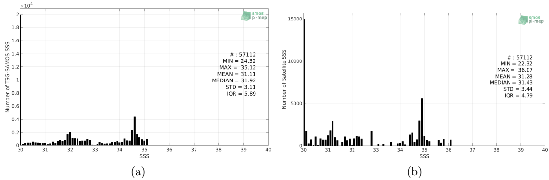
Figure 2: Histograms of SSS from TSG-SAMOS (a) and Aquarius-L3-JPL-V5-MONTHLY (b) considering all match-up pairs per bins of 0.1 over the Arctic Ocean Pi-MEP region and for the full satellite product period.
