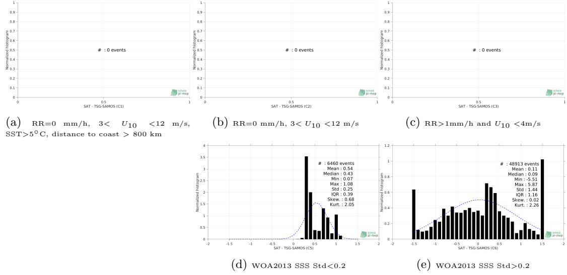
Figure 13: Normalized histogram of \Delta\text{SSS} (Aquarius-L3-JPL-V5-MONTHLY - TSG-SAMOS) for 5 different subdatasets corresponding to: RR=0 mm/h, 3 < U_{10} < 12 m/s, SST > 5^\circ\text{C} , distance to coast > 800 km (a), RR=0 mm/h, 3 < U_{10} < 12 m/s (b), RR > 1 mm/h and U_{10} < 4 m/s (c), WOA2013 SSS Std < 0.2 (d), WOA2013 SSS Std > 0.2 (e).
