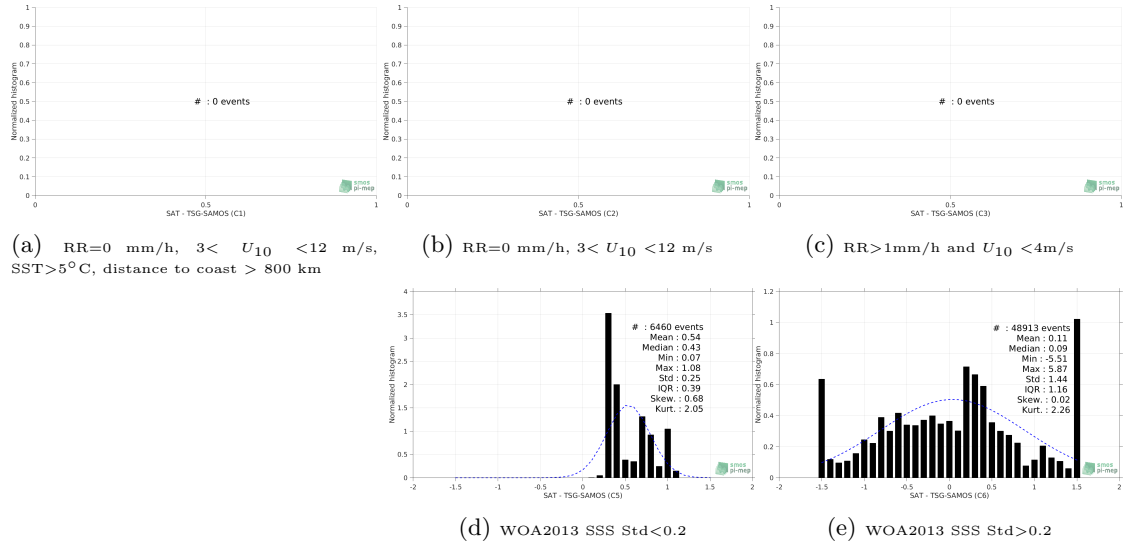
Figure 13: Normalized histogram of \Delta\text{SSS} (Aquarius-L3-JPL-V5-MONTHLY - TSG-SAMOS) for 5 different subdatasets corresponding to: RR=0 mm/h, 3 < U_{10} < 12 m/s, SST >5^{\circ}\text{C} , distance to coast > 800 km (a), RR=0 mm/h, 3 < U_{10} < 12 m/s (b), RR >1 mm/h and U_{10} < 4 m/s (c), WOA2013 SSS Std <0.2 (d), WOA2013 SSS Std >0.2 (e).
