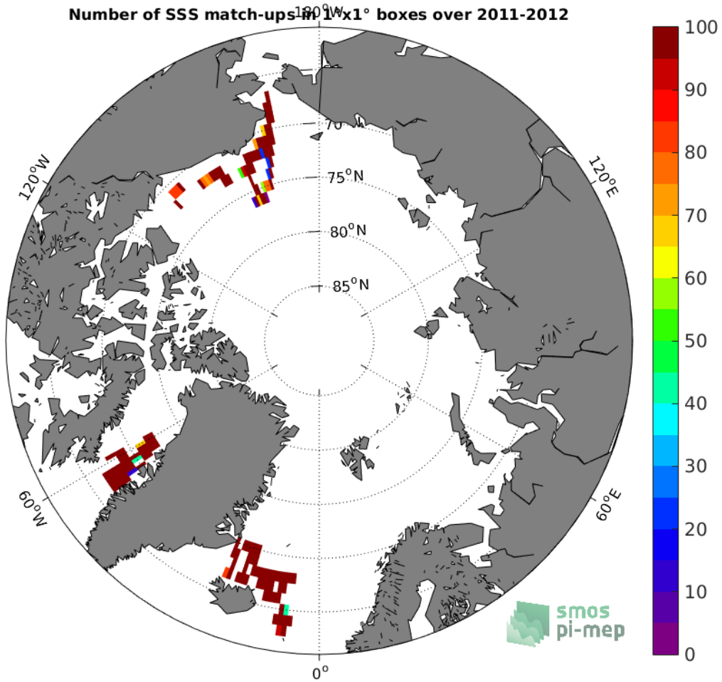
Figure 4: Number of SSS match-ups between TSG-SAMOS SSS and the Aquarius-L3-JPL-V5-MONTHLY SSS product for the Arctic Ocean Pi-MEP region over 1°x1° boxes and for the full satellite product period.
