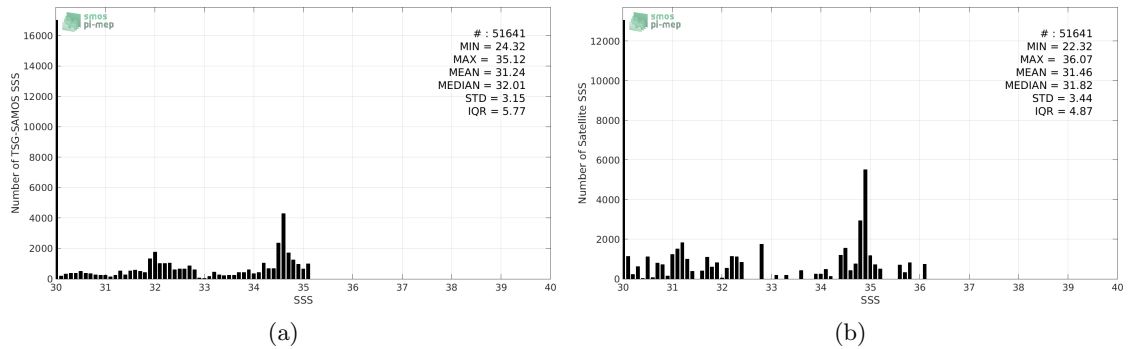
Figure 2: Histograms of SSS from TSG-SAMOS (a) and Aquarius-L3-JPL-V5-MONTHLY (b) considering all match-up pairs per bins of 0.1 over the Arctic Ocean Pi-MEP region and for the full satellite product period.
