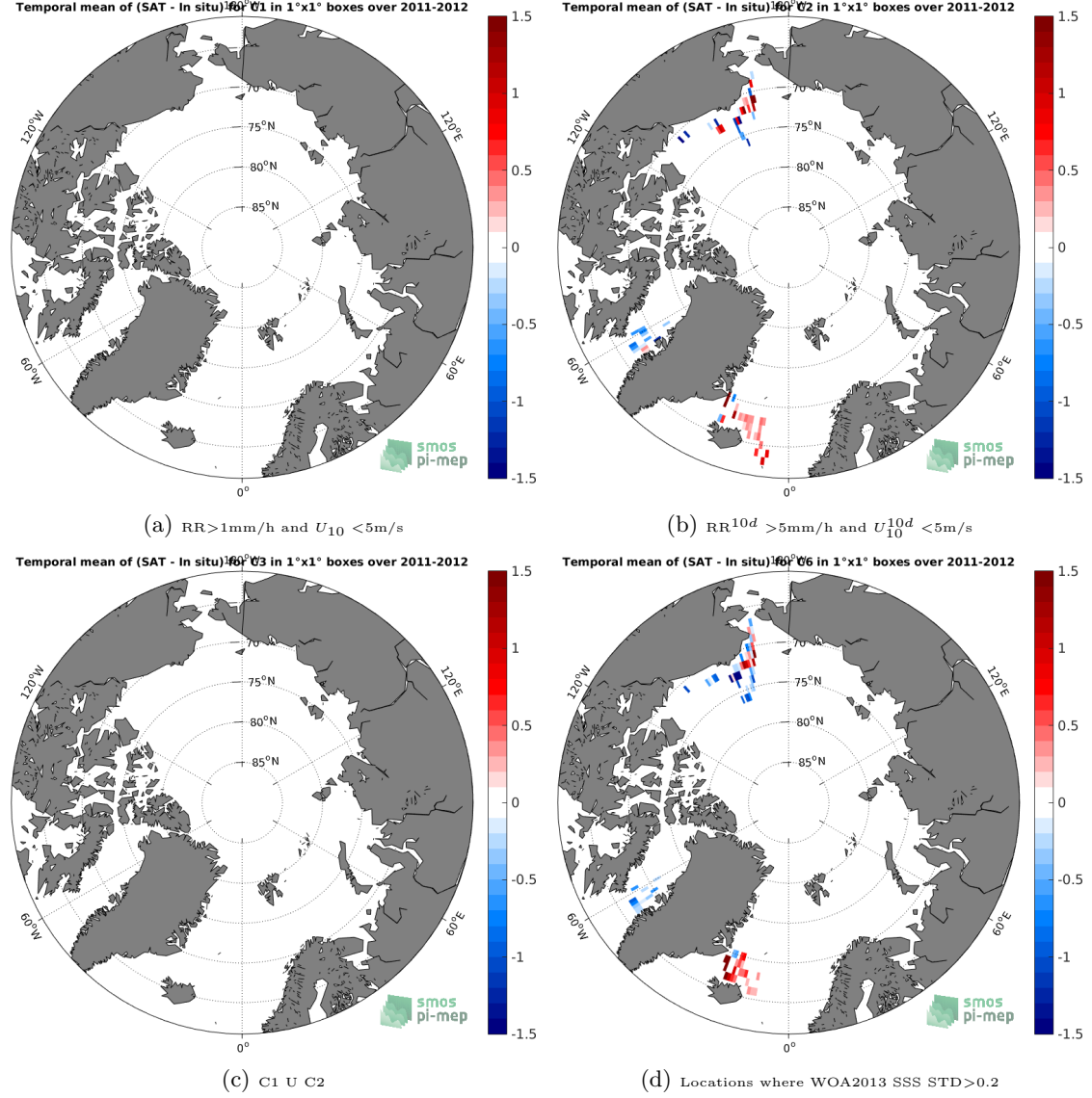
Figure 12: Temporal mean gridded over spatial boxes of size 1^\circ \times 1^\circ of \Delta SSS (Aquarius-L3-JPL-V5-MONTHLY - TSG-SAMOS) for 4 different subdatasets corresponding to: RR > 1\text{mm/h} and U_{10} < 5\text{m/s} (a), RR^{10d} > 5\text{mm/h} and U_{10}^{10d} < 5\text{m/s} (b), C1 U C2 (c), Locations where WOA2013 SSS STD > 0.2 (d).
