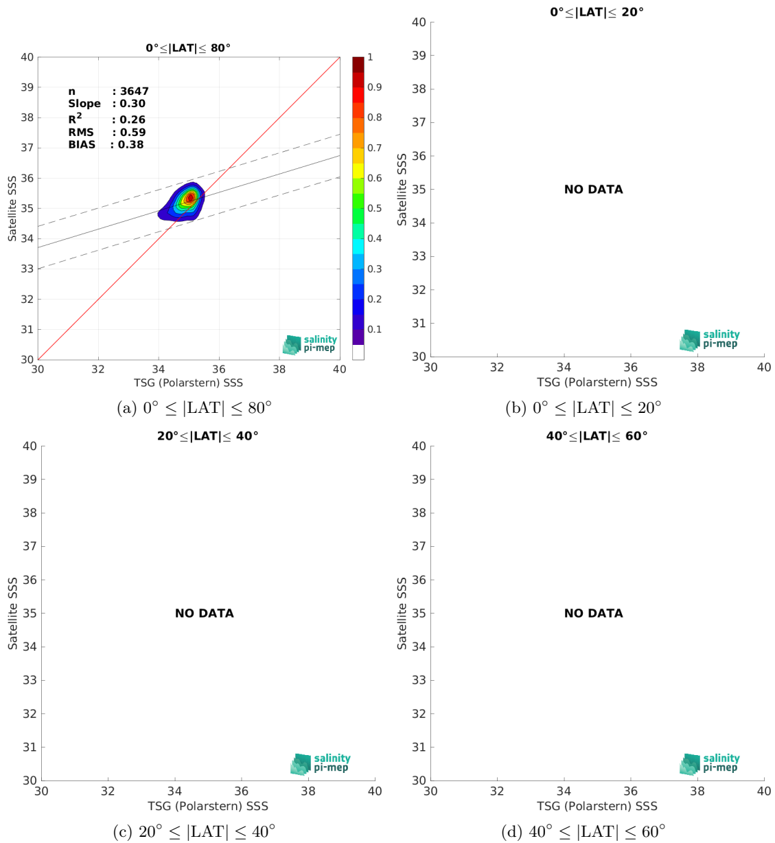
Figure 10: Contour maps of the concentration of Aquarius SSS L3 CAP v5 - Monthly (JPL) SSS (y-axis) versus TSG (Polarstern) SSS (x-axis) at match-up pairs for different latitude bands. For each plot, the red line shows x=y . The black thin and dashed lines indicate a linear fit through the data cloud and the \pm 95\% confidence levels, respectively. The number match-up pairs n , the slope and R^2 coefficient of the linear fit, the root mean square (RMS) and the mean bias between satellite and in situ data are indicated for each latitude band in each plots.
