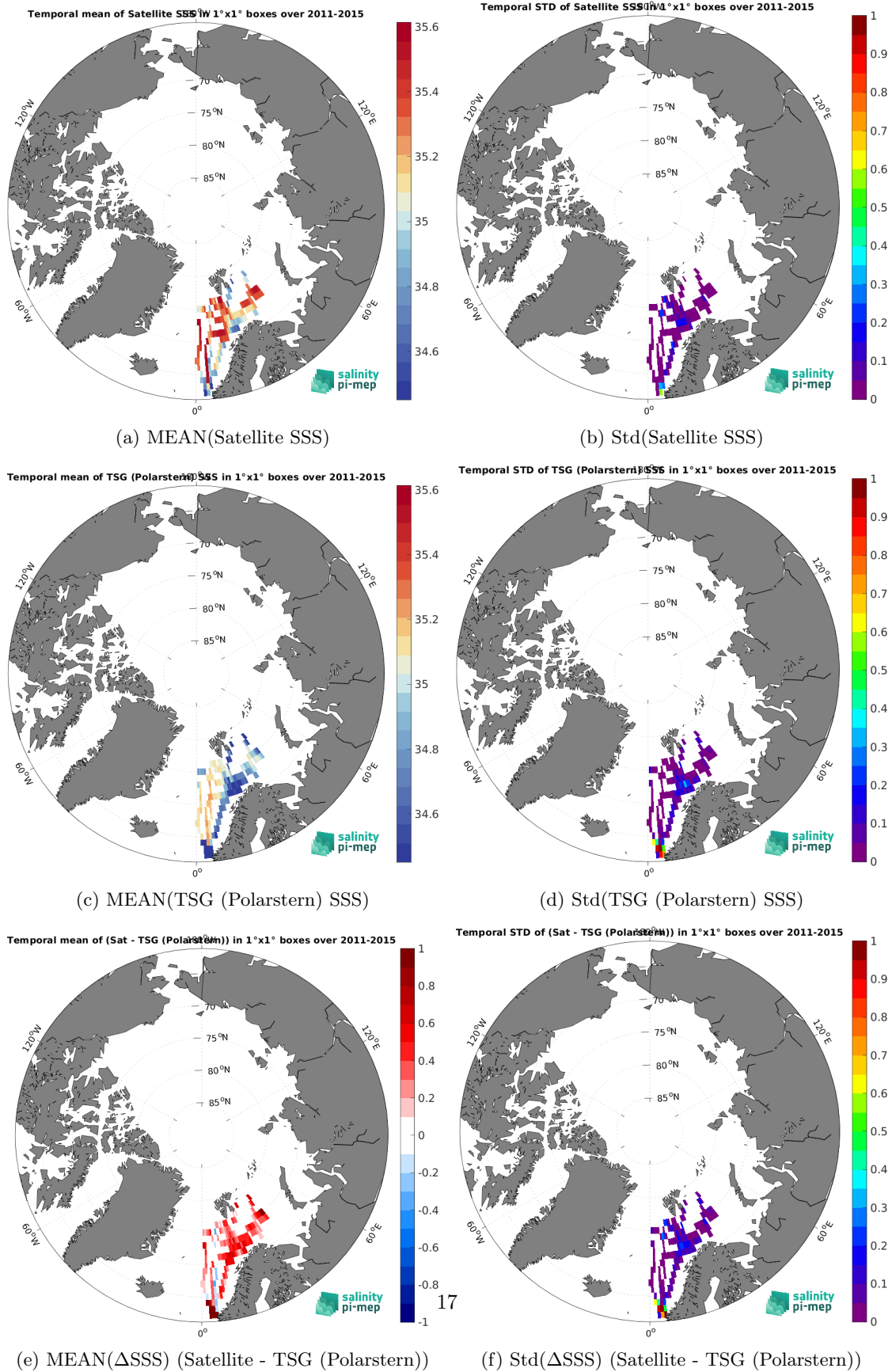
Figure 7: Temporal mean (left) and Std (right) of SSS from Aquarius SSS L3 CAP v5 - Monthly (JPL) (top), TSG (Polarstern) (middle), and of \Delta SSS (Satellite - TSG (Polarstern)). Only match-up pairs are used to generate these maps.
