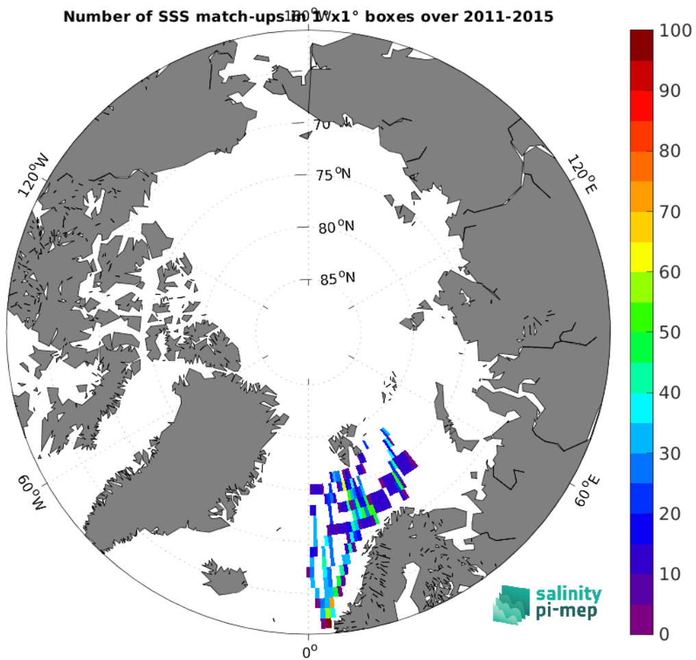
Figure 5: Number of SSS match-ups between TSG (Polarstern) SSS and the Aquarius SSS L3 CAP v5 - Monthly (JPL) SSS product for the Arctic Ocean Pi-MEP region over 1^\circ \times 1^\circ boxes and for the full satellite product period.
