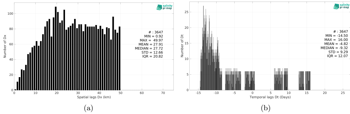
Figure 6: Histograms of the spatial (a) and temporal (b) lags between the location/time of the TSG (Polarstern) measurement and the date of the corresponding Aquarius SSS L3 CAP v5 - Monthly (JPL) SSS pixel.
