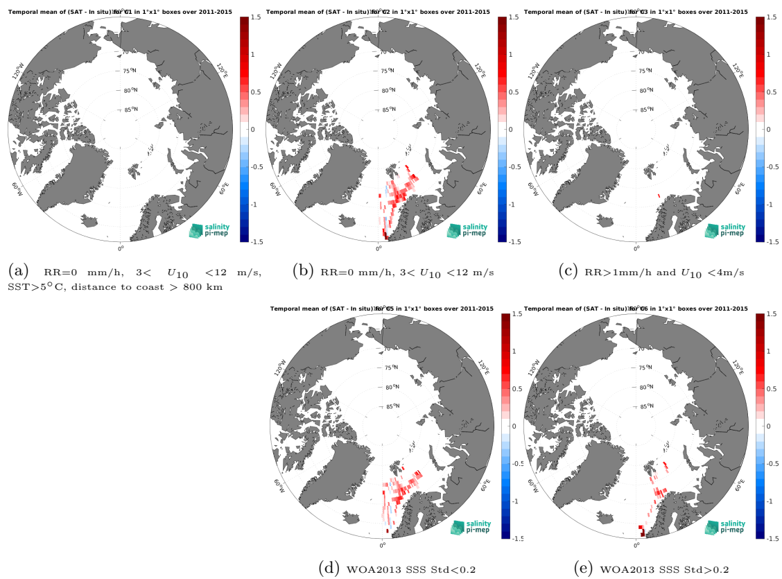
Figure 14: Temporal mean gridded over spatial boxes of size 1^\circ \times 1^\circ of \Delta\text{SSS} (Aquarius SSS L3 CAP v5 - Monthly (JPL) - TSG (Polarstern)) for 5 different subdatasets corresponding to:RR=0 mm/h, 3 < U_{10} < 12 m/s, SST > 5°C, distance to coast > 800 km (a), RR=0 mm/h, 3 < U_{10} < 12 m/s (b), RR > 1mm/h and U_{10} < 4 m/s (c), WOA2013 SSS Std < 0.2 (d), WOA2013 SSS Std > 0.2 (e).
