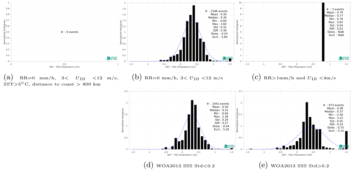
Figure 15: Normalized histogram of \Delta SSS (Aquarius SSS L3 CAP v5 - Monthly (JPL) - TSG (Polarstern)) for 5 different subdatasets corresponding to: RR=0 mm/h, 3 < U_{10} < 12 m/s, SST > 5°C, distance to coast > 800 km (a), RR=0 mm/h, 3 < U_{10} < 12 m/s (b), RR > 1mm/h and U_{10} < 4 m/s (c), WOA2013 SSS Std < 0.2 (d), WOA2013 SSS Std > 0.2 (e).
