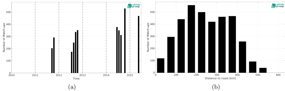
Figure 2: Number of match-ups between TSG (Polarstern) and Aquarius SSS L3 CAP v5 - Monthly (JPL) SSS as a function of time (a) and as function of the distance to coast (b) over the Arctic Ocean Pi-MEP region and for the full satellite product period.
