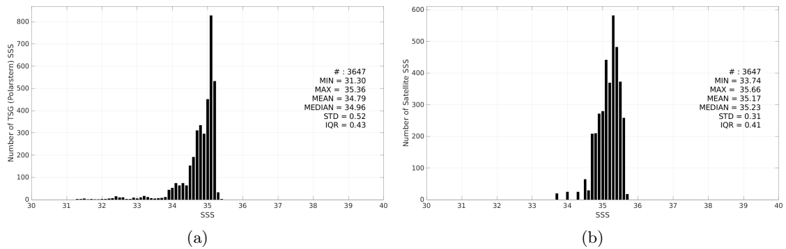
Figure 3: Histograms of SSS from TSG (Polarstern) (a) and Aquarius SSS L3 CAP v5 - Monthly (JPL) (b) considering all match-up pairs per bins of 0.1 over the Arctic Ocean Pi-MEP region and for the full satellite product period.
